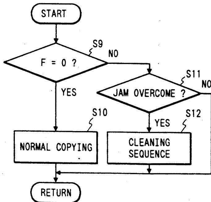
SUB-ROUTINE FOR COPYING OPERATION
