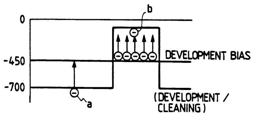
FIG. 16c PRIOR ART
