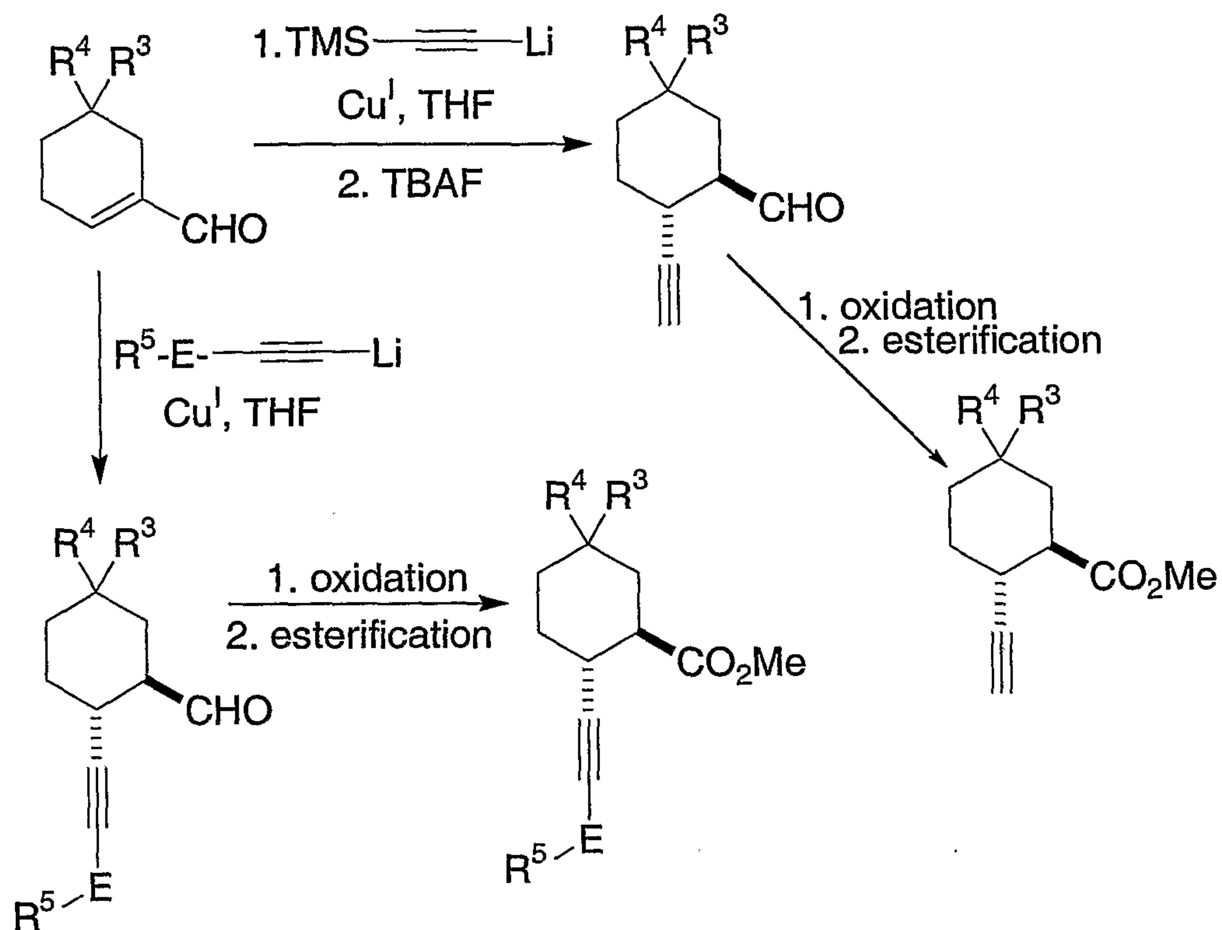
SCHEME 9
