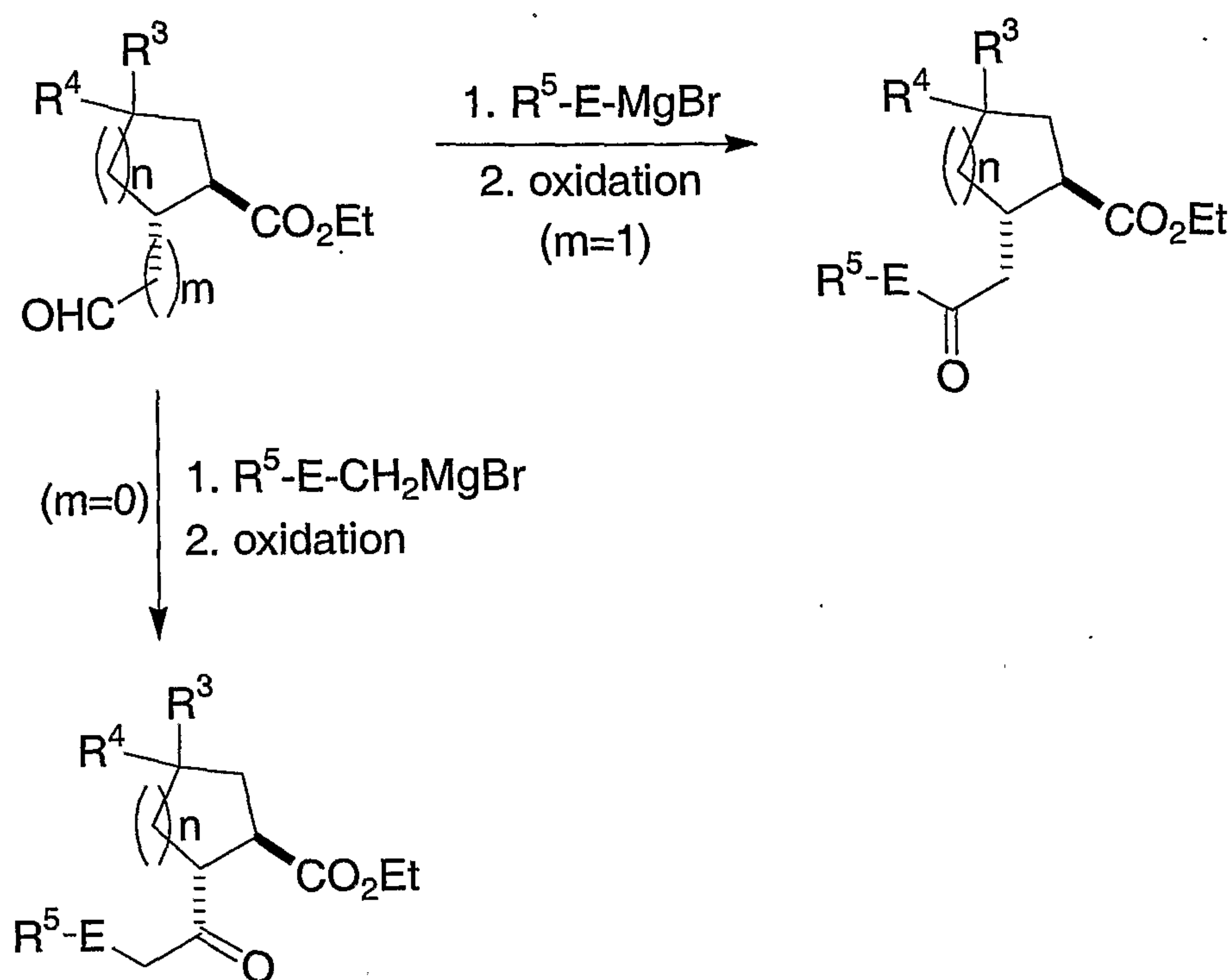
SCHEME 5C
