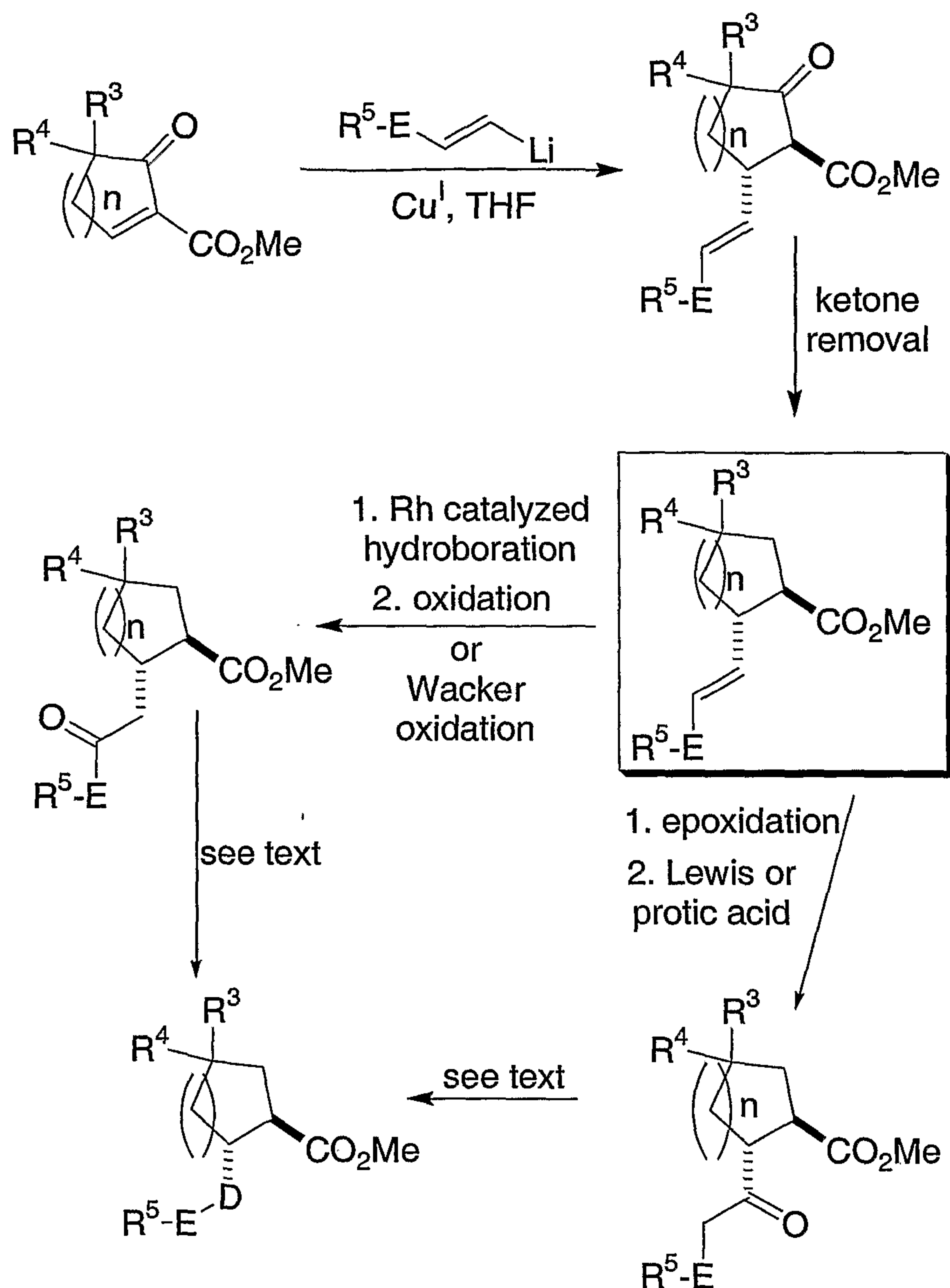
SCHEME 4
