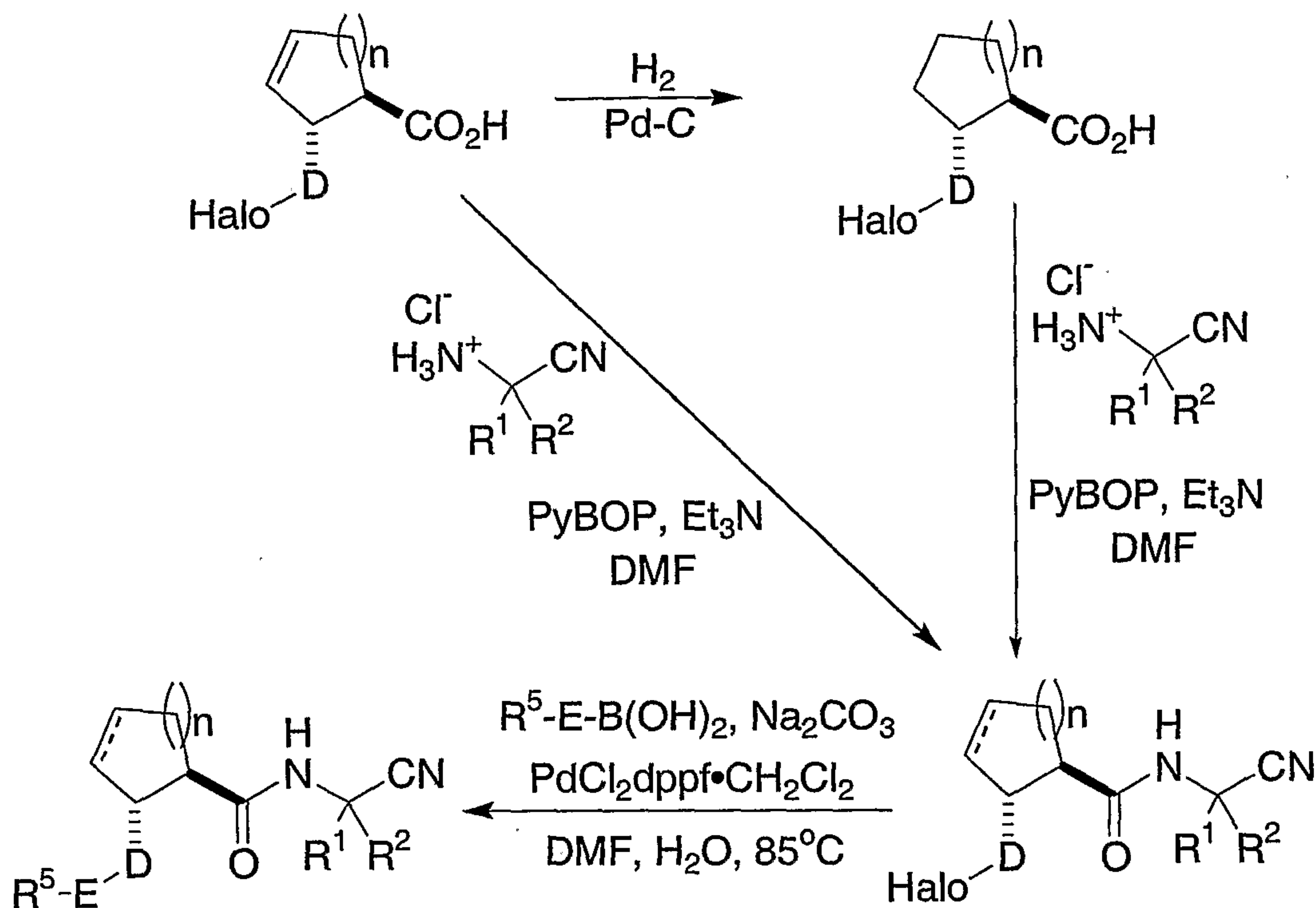
SCHEME 1
