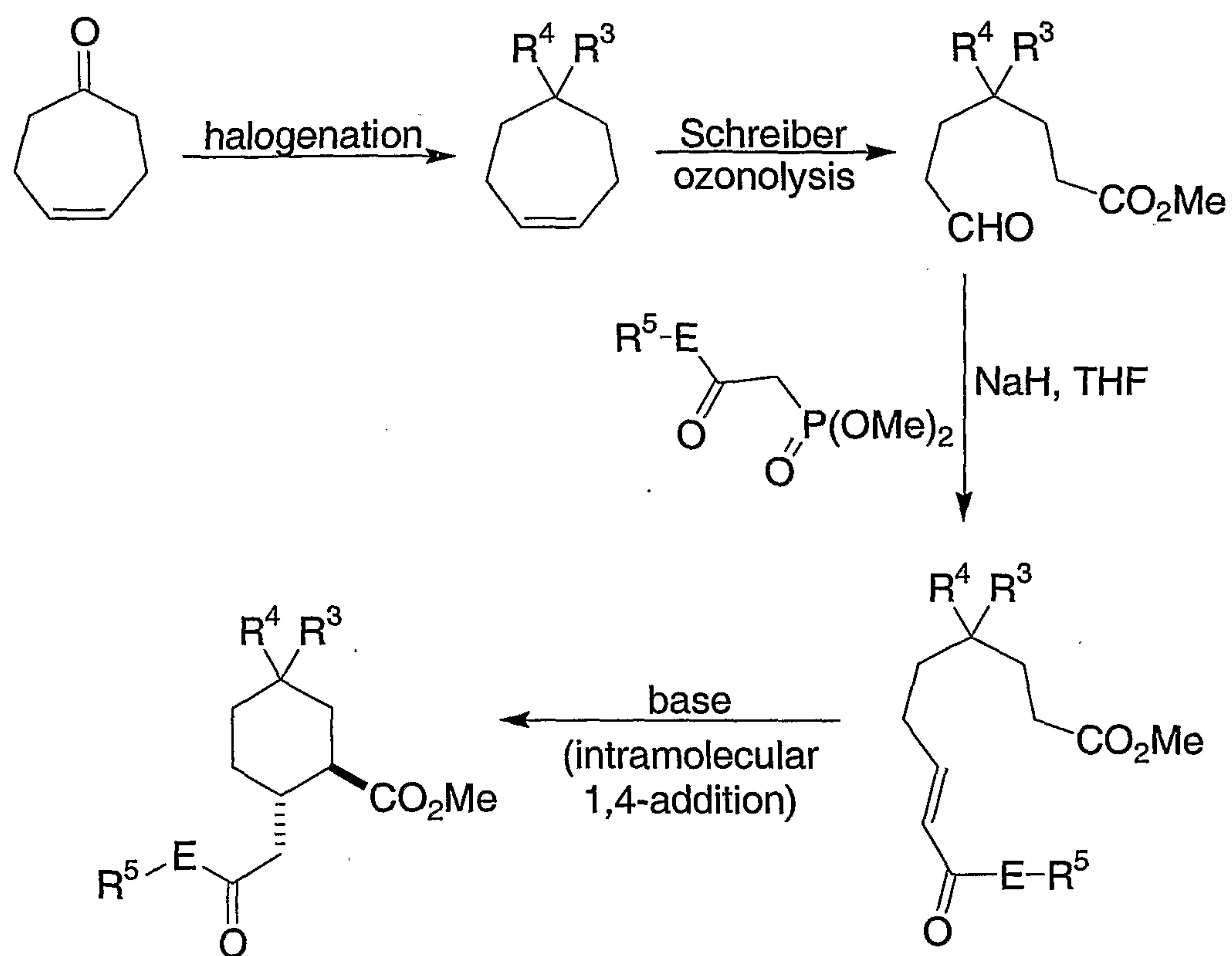
SCHEME 6
