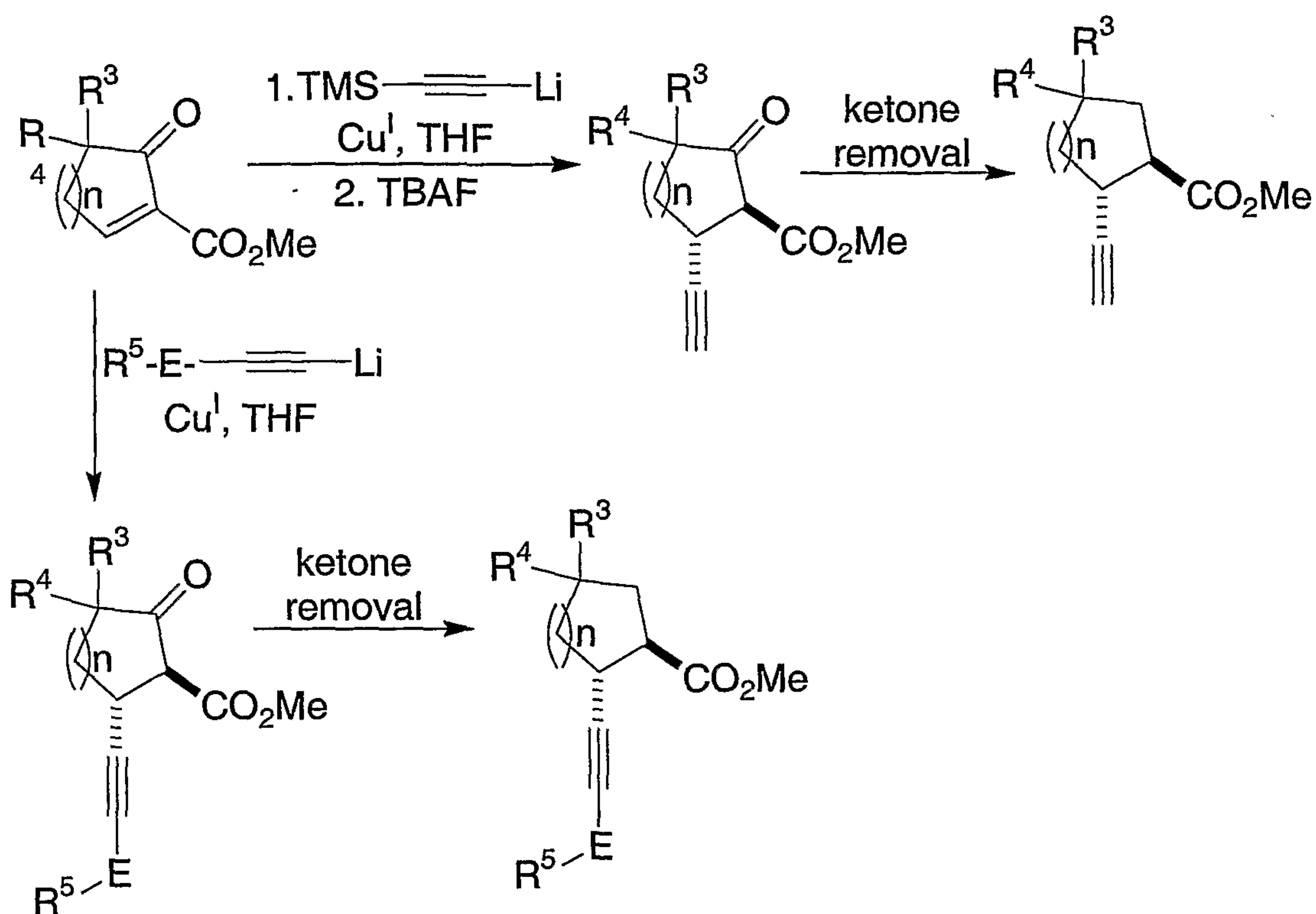
SCHEME 5B
