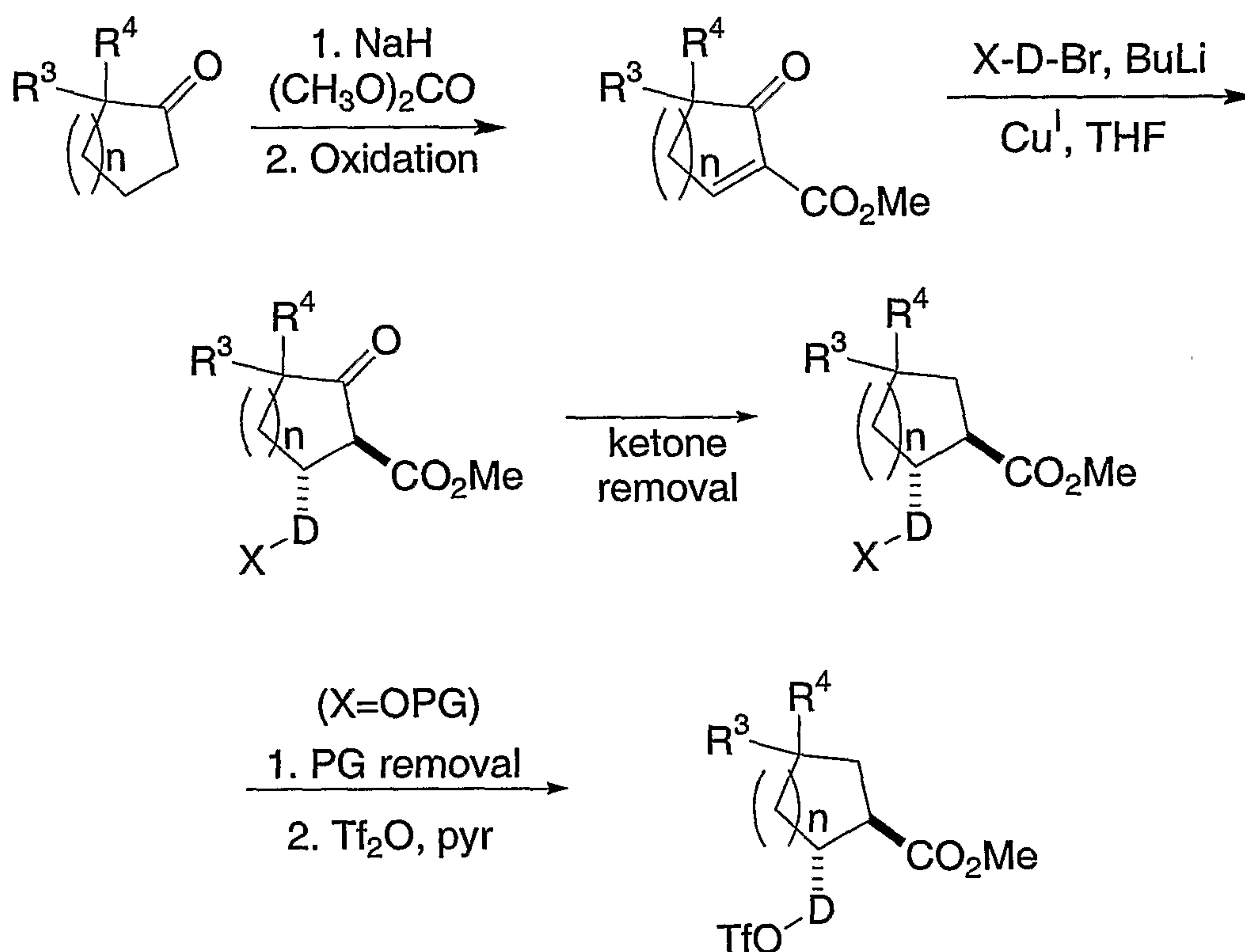
SCHEME 3
