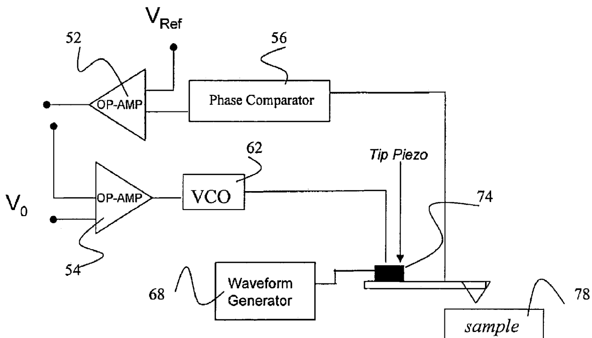
Figure 7. Micro-cantilever resonance feedback circuit.
