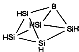
Compound 11
