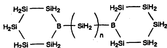
Compound 10
