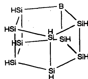
Compound 13
