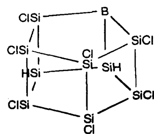
Compound 23
