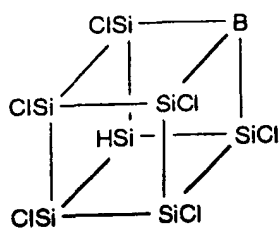
Compound 22
