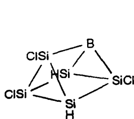
Compound 21
