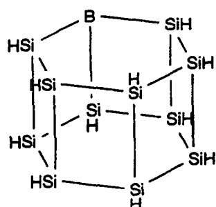
Compound 14
