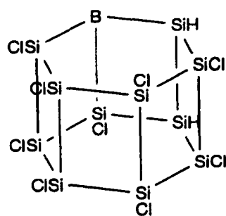
Compound 24
