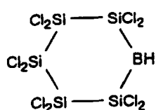
Compound 17
