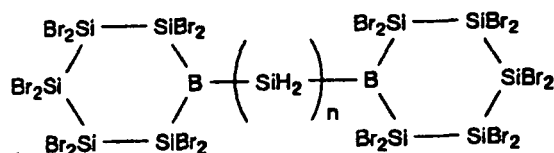
Compound 20
