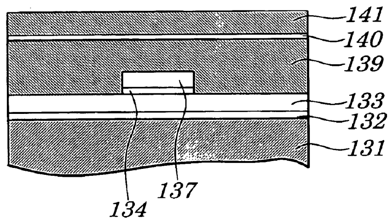
FIG. 14D (PRIOR ART)
