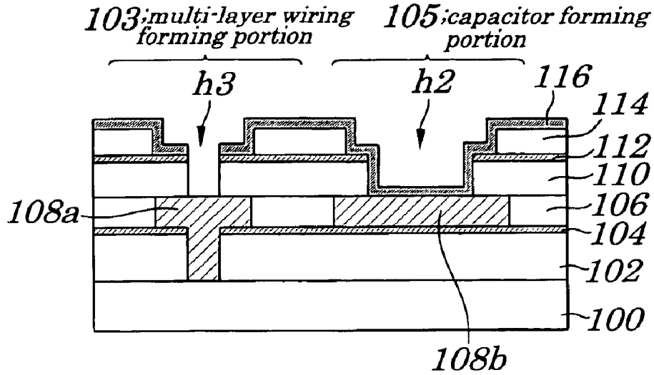
FIG. 12E (PRIOR ART)
