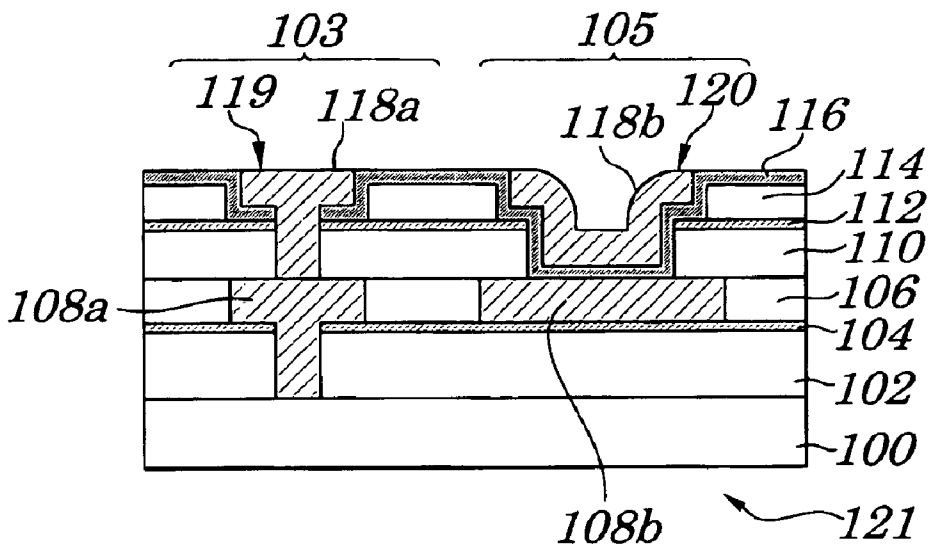
FIG. 12E (PRIOR ART)
