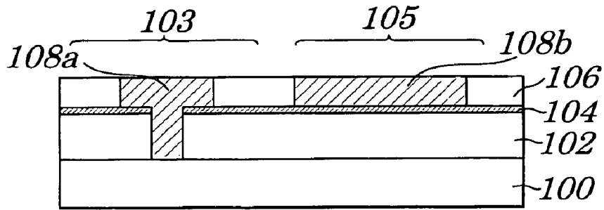
FIG. 12B (PRIOR ART)
