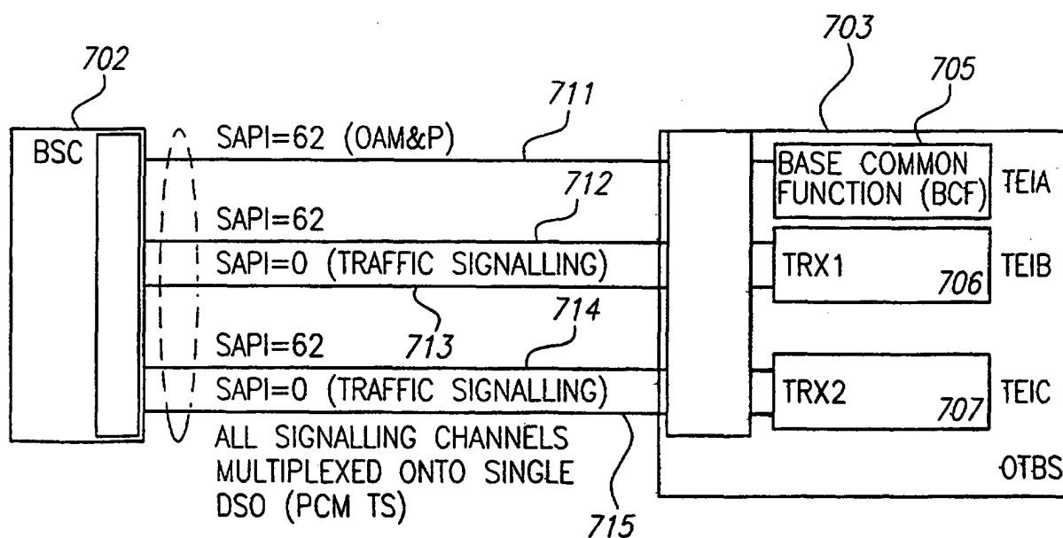
INTERFACE SIGNALLING STRUCTURES
