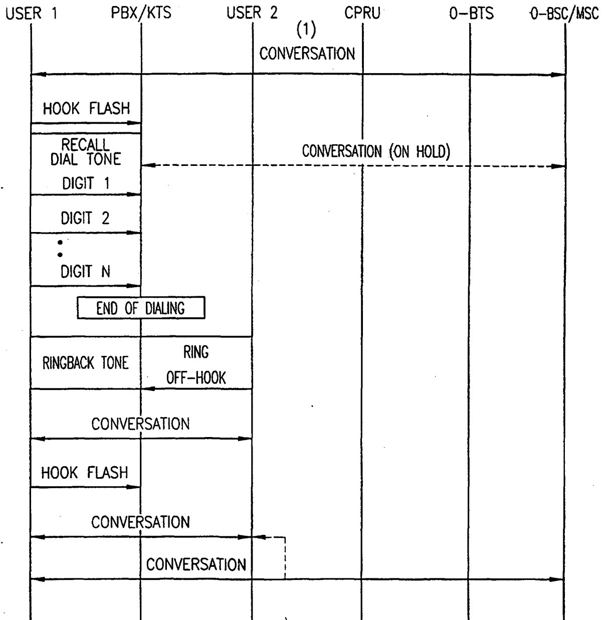
THREE-WAY CALL SETUP SCENARIO
