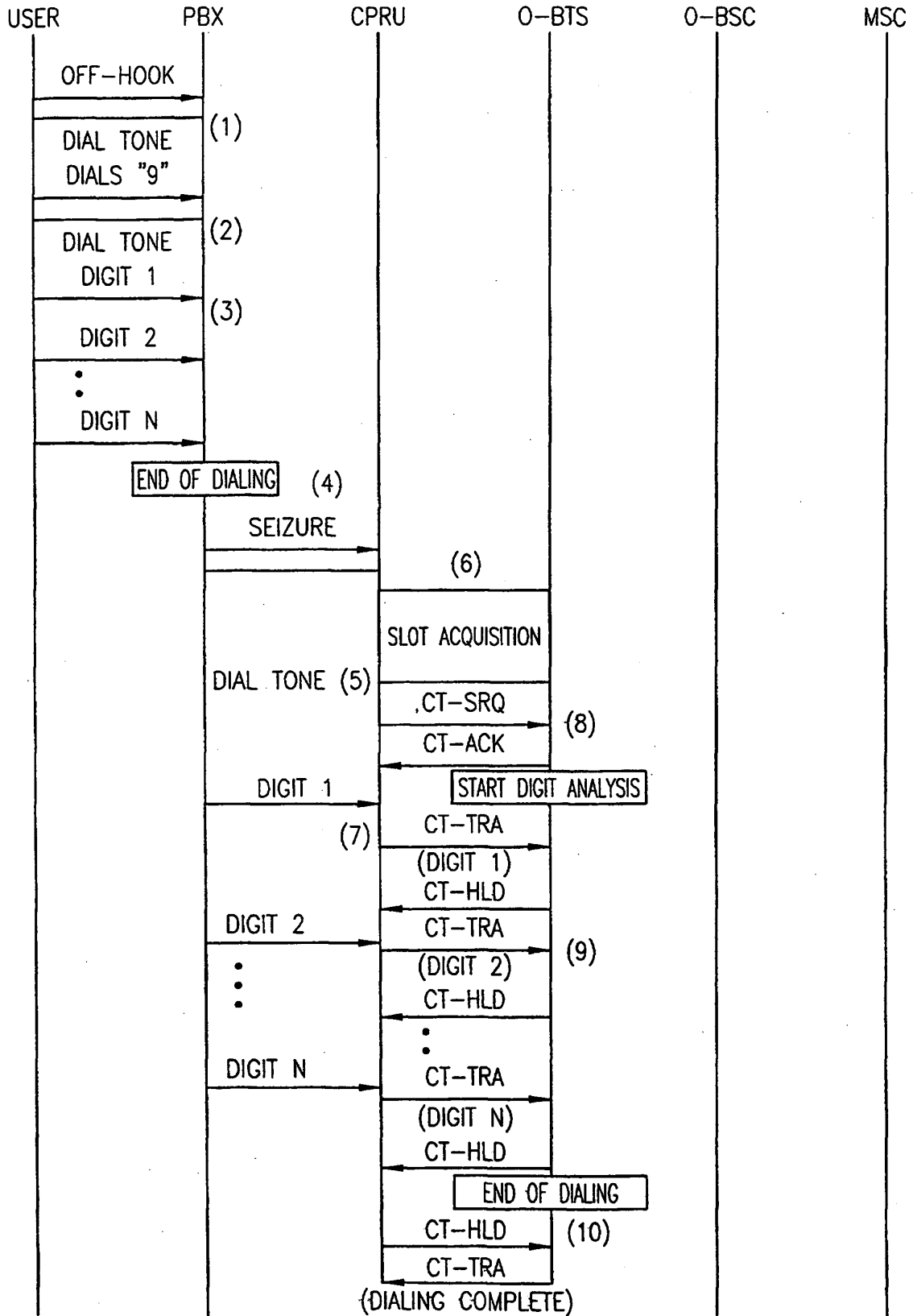
DIAL TONE, DIGIT TRANSMISSION AND DIGIT ANALYSIS FOR A MORE MODERN PBX
