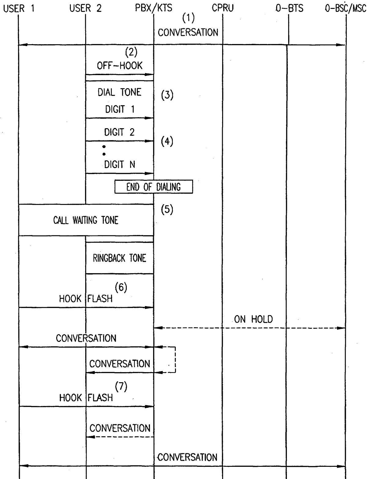
CALL WAITING SCENARIO
