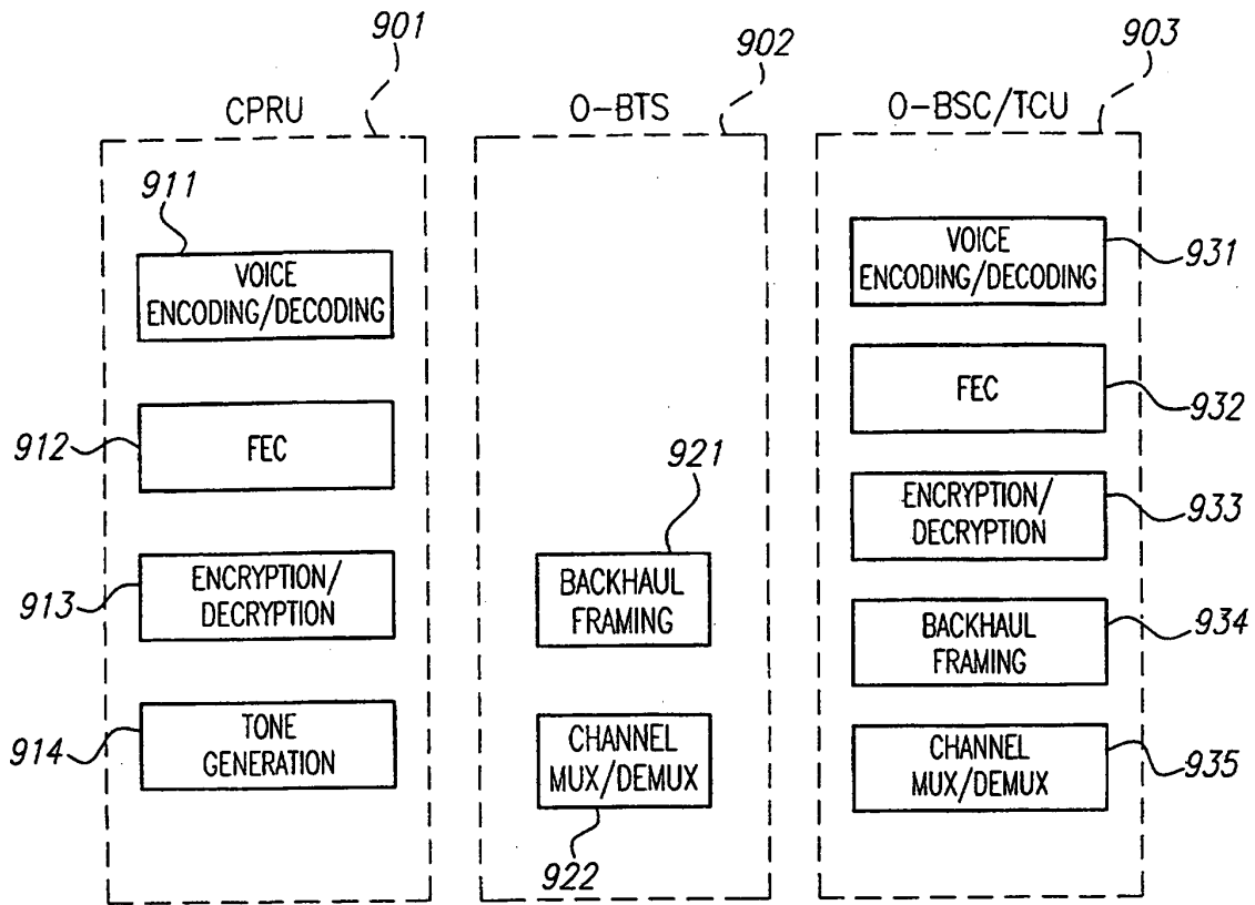
BEARER PATH FUNCTIONS
