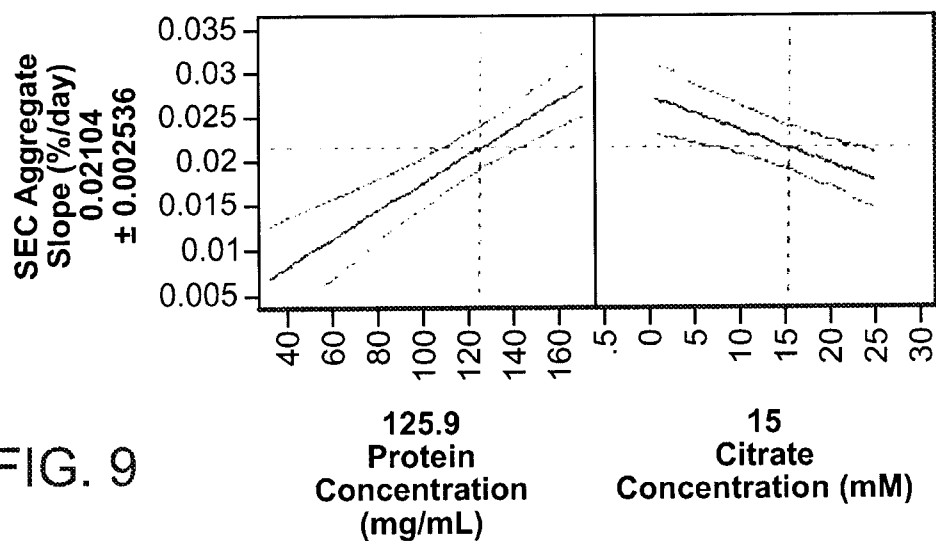
Prediction Profiler
