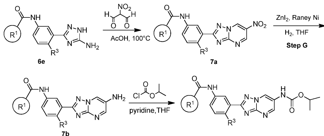
Scheme 8.
