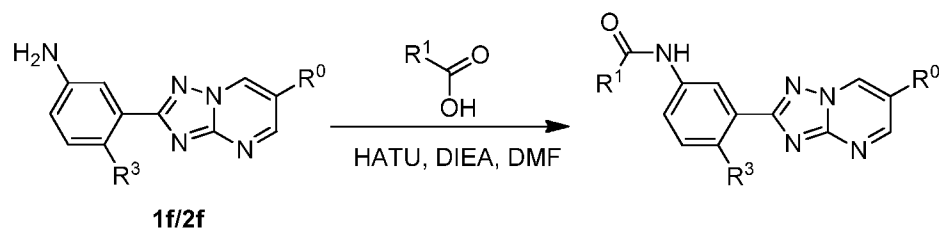
Scheme 3. Coupling of -C(O)-R 1 where R 1 is C 5-6 heteroaryl or C 3-6 cycloalkyl to the phenyl-triazolopyrimidine
