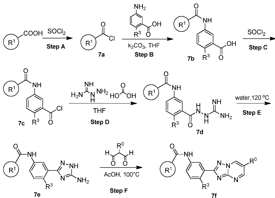
Scheme 8.
