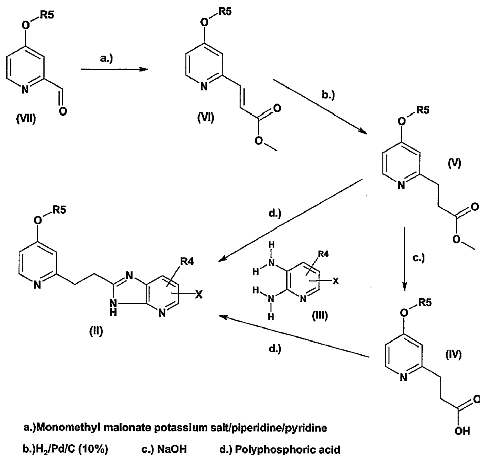
Reaction Scheme 2:
