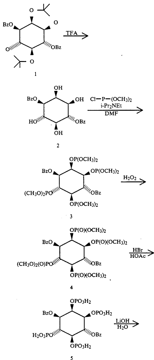
Scheme 2. Synthesis of Myo-inositol 1,2,4,5-Tetrakis(phosphate) (6).
