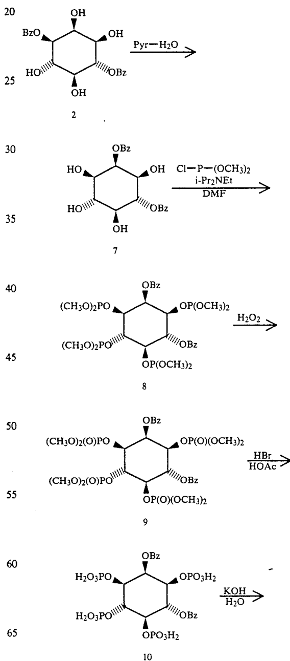
Synthesis of Myo-inositol 1,3,4,5-Tetrakis(phosphate) (11).
