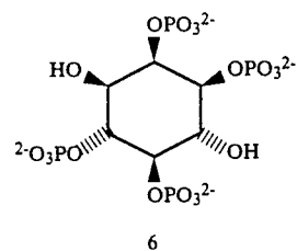
Synthesis of Myo-inositol 1,2,4,5-Tetrakis(phosphate) (6).
