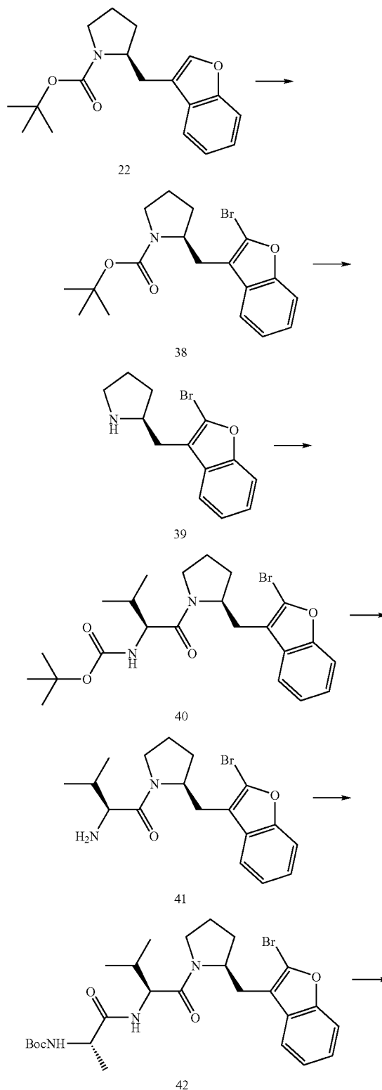
Scheme V
