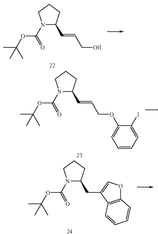
Scheme IV(a)
