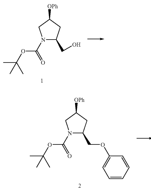
Scheme I
