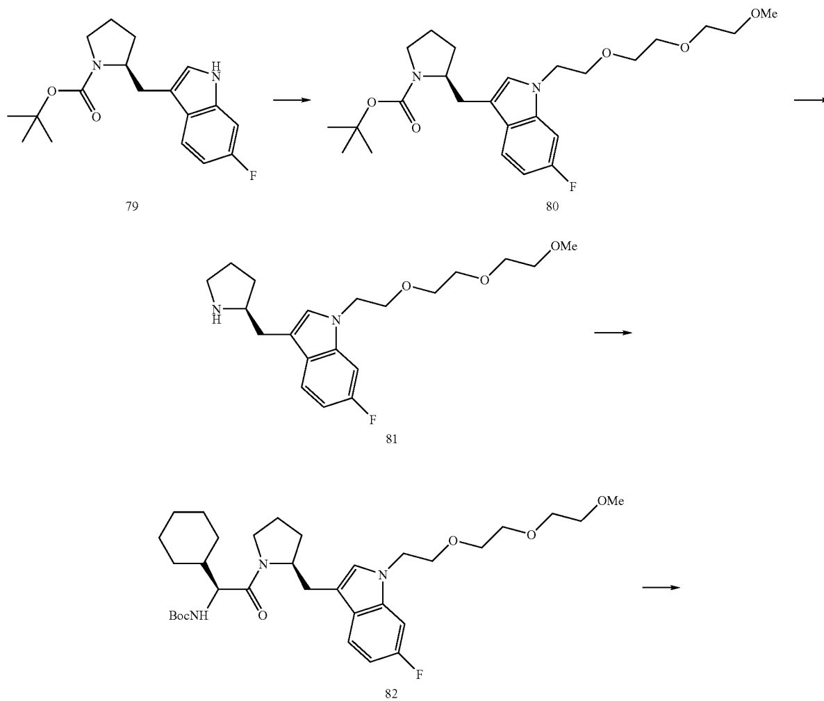
Scheme VIII
