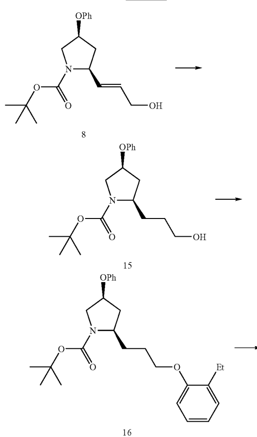
Scheme III
