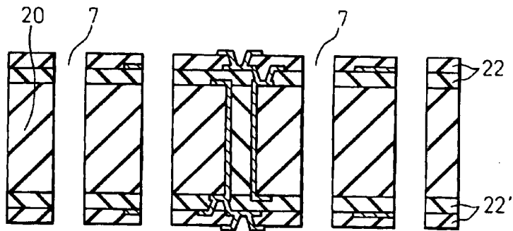
Fig.9B PRIOR ART
