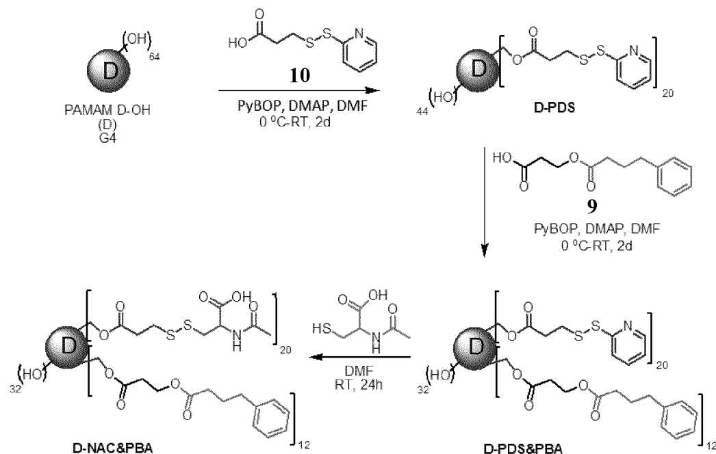
Scheme 7. Synthesis route for D-NAC&PBA through propionyl linkers for 4th generation PAMAM dendrimer
