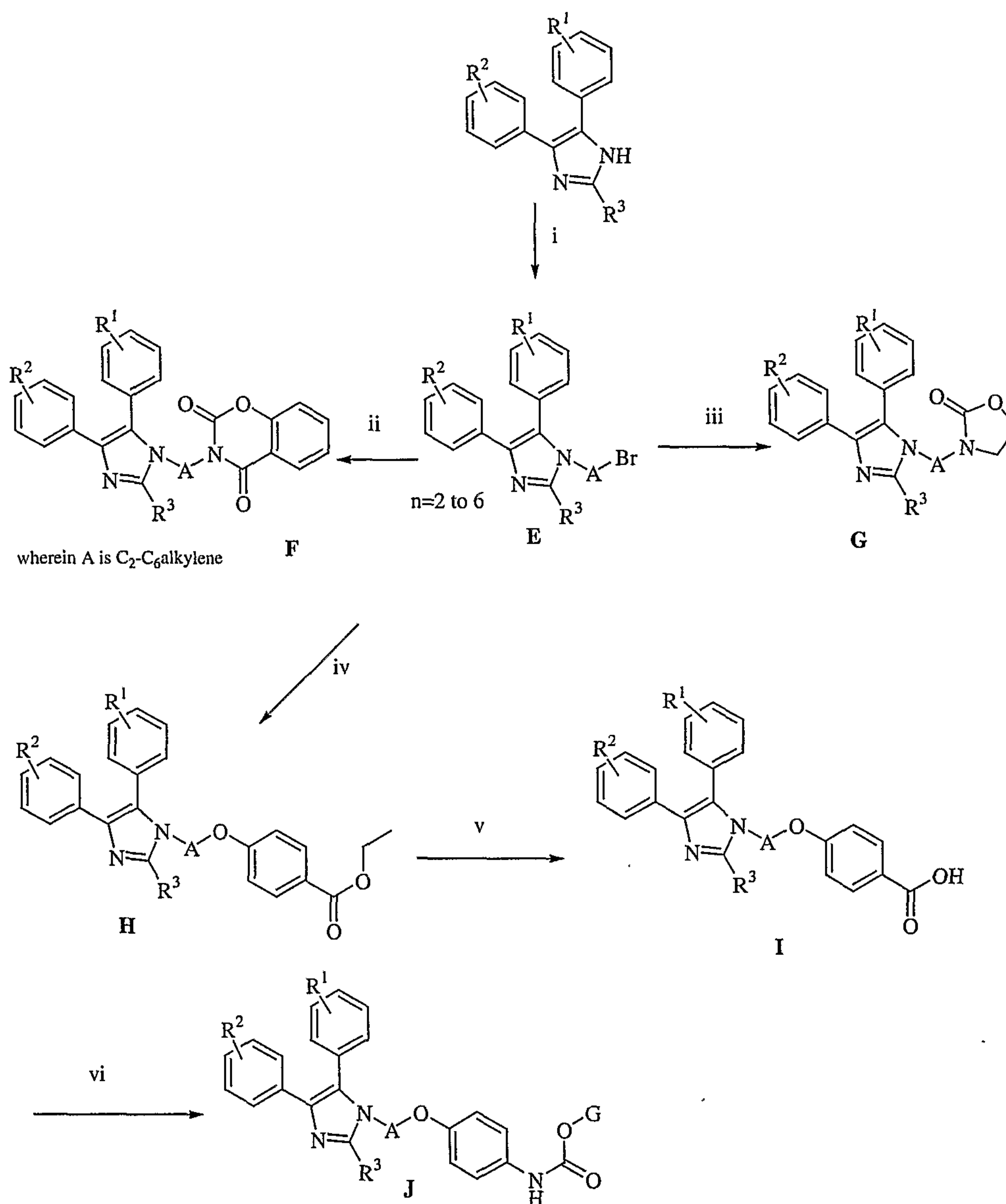
Scheme 2. Reaction conditions: (i) dibromide, NaH, DMF, rt; (ii) 2 H-1,3-benzoxazine-2,4(3 H)-dione, K 2 CO 3 , DMF, 85 °C; (iii) 2-oxazolidone, NaH, DMF, rt; (iv) ethyl 4-hydroxybenzoate, K 2 CO 3 , DMF, 55 °C; (v) NaOH, EtOH, rt; (vi) (a) N 3 P(O)(OPh) 2 , Et 3 N, toluene, 105 °C, (b) GOH, 80 °C.
