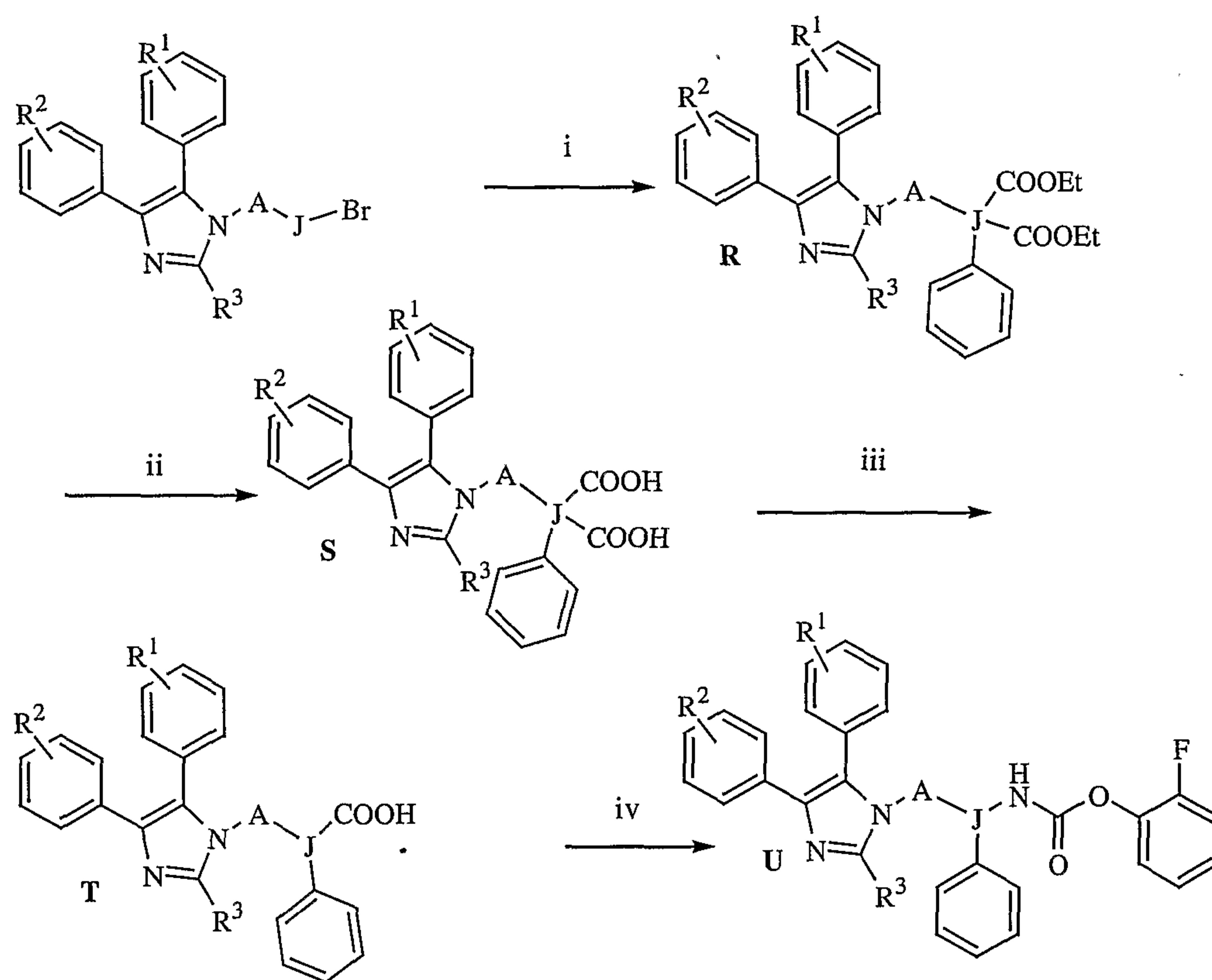
Scheme 4. Reaction conditions: (i) (a) NaH, DMF, rt, (b) diethyl phenyl malonate, 45-50 °C (ii) NaOH, THF, 80 °C; (iii) CH 3 COOH, reflux; (iv) (a) N 3 P(O)(OPh) 2 , Et 3 N, toluene, 108 °C, (b) 2-fluorophenol, 100 °C.
