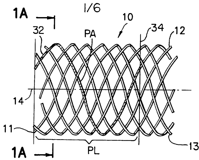
FIG. 1 PRIOR ART
