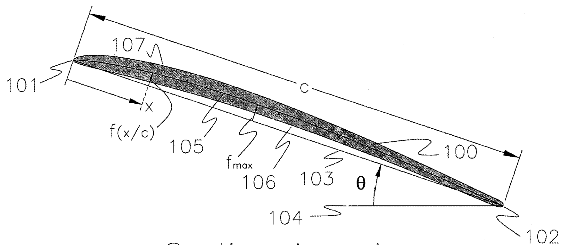
Section A — A Figure 3a
