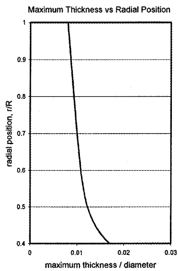
prior art Figure 5a
