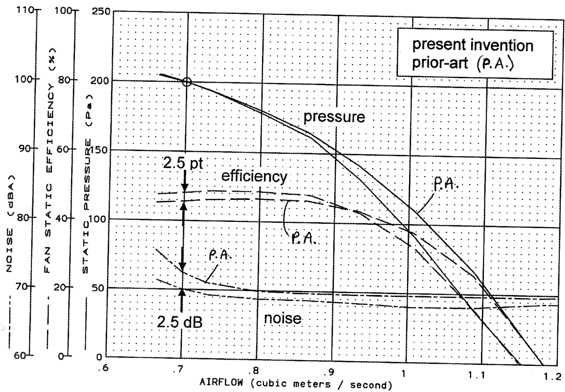
performance of present invention vs prior art Figure 11
