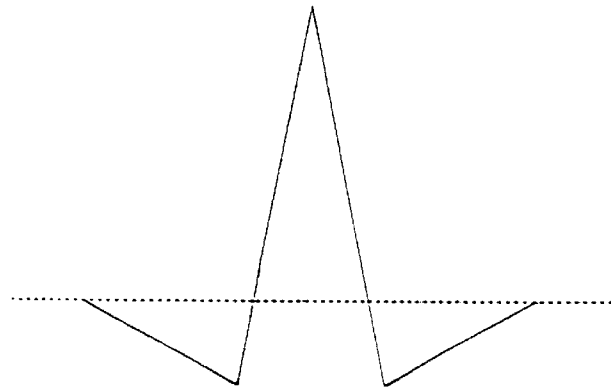
Figure 2: Cohen-Daubechies-Feauveau (2.2) biorthogonal wavelet.
