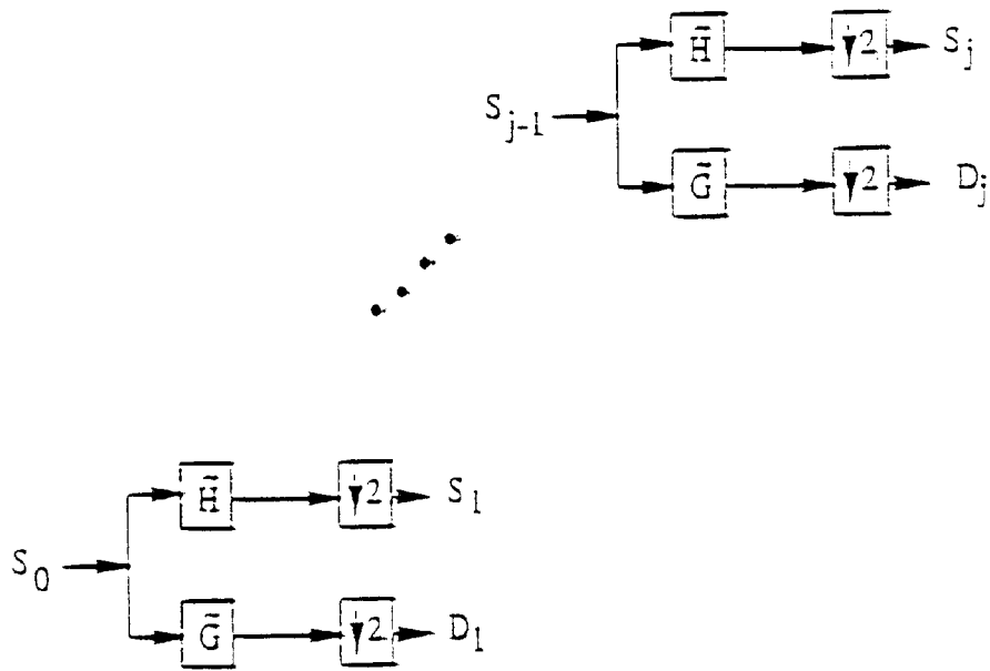
Figure 4: Block diagram of multi-resolution wavelet transform.
