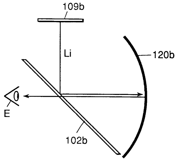
FIG.2 ( PRIOR ART )
