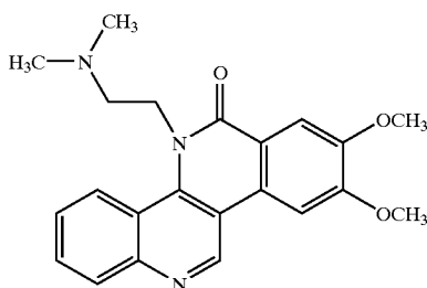
8,9-Dimethoxy-5-[2-(N,N-dimethylamino)ethyl]-5H-dibenzo[h,1,6-naphthyridin-6-one (5).
