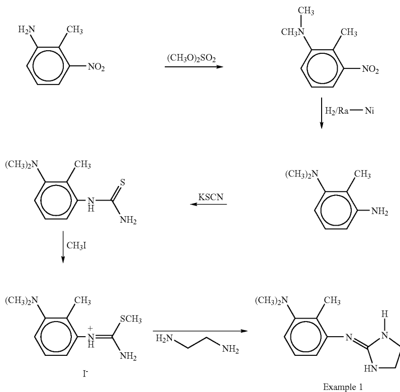
Synthetic Scheme II
