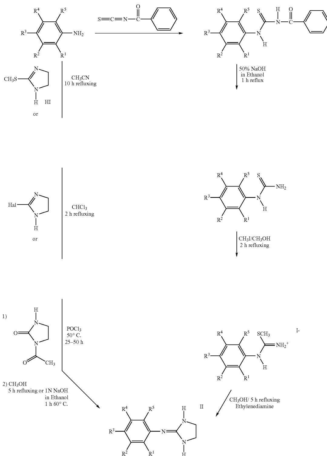
Synthetic Scheme I
