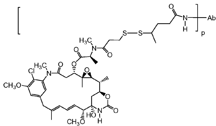
Ab-SPP-DM1
