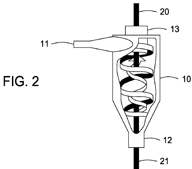
Carbon Arc in Cyclone separator
