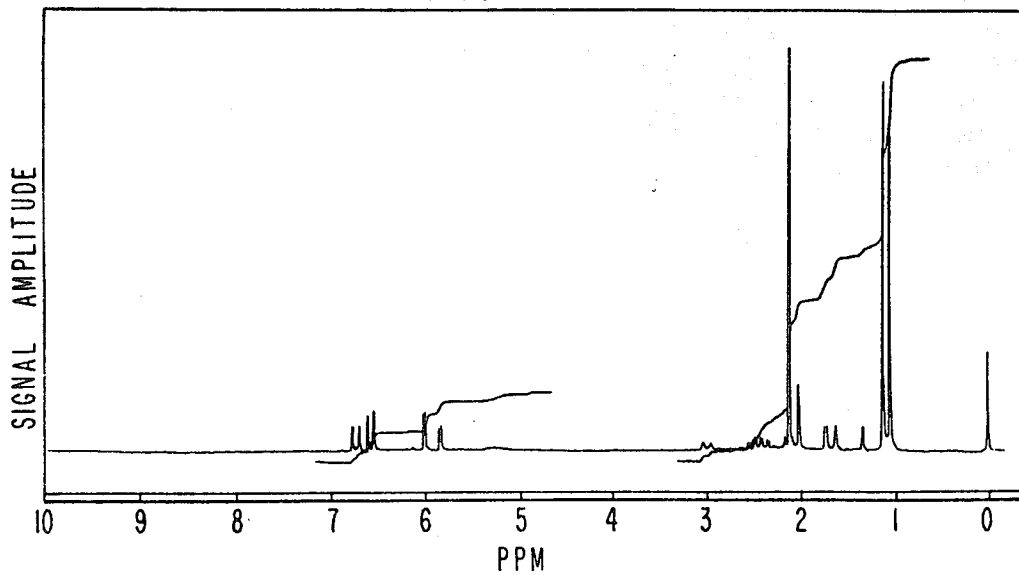
NMR SPECTRUM FOR EXAMPLE A .
