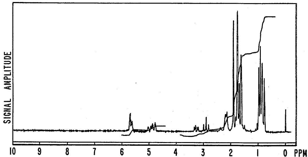
NMR SPECTRUM FOR PEAK 4A OF EXAMPLE I.
