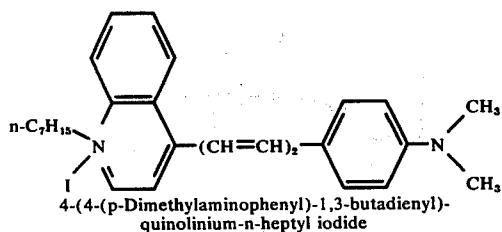
Compound II-23
