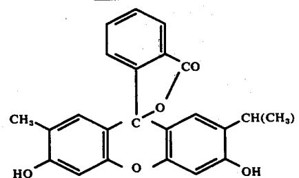
Compound VIII-5
