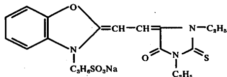
Compound III-13
