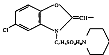
Compound III-17
