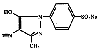
Compound VII-1
