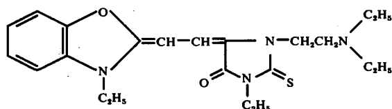
Compound III-16
