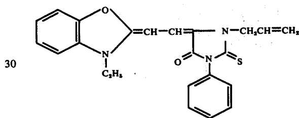
Compound III-7
