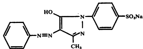
Compound VI-3
