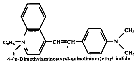
Compound II-16
