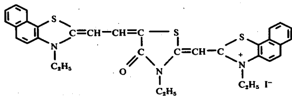
Compound I-6
