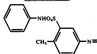
Compound VI-6
