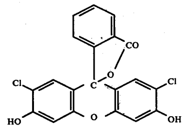
Compound VIII-2
