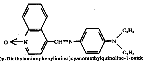
Compound II-15
