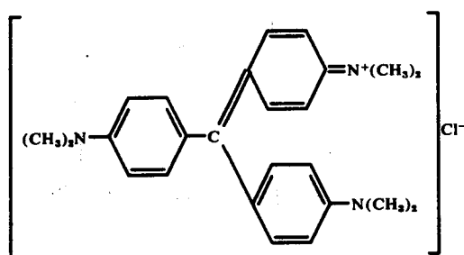
Compound V-7
