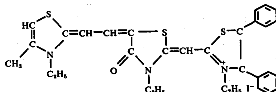
Compound I-2
