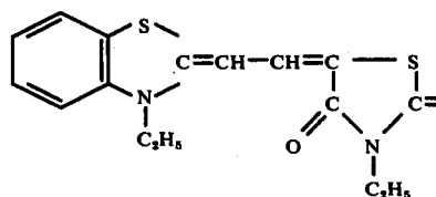
Compound I-15
