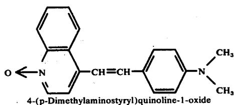
Compound II-14
