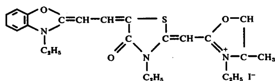
Compound I-14
