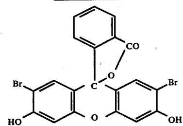
Compound VIII-3
