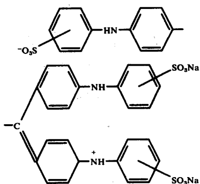
Compound V-5
