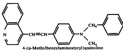
Compound II-13
