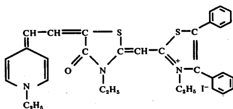
Compound I-8
