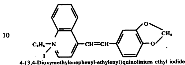
15 Compound II-18
