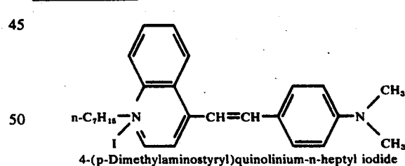
Compound II-21
