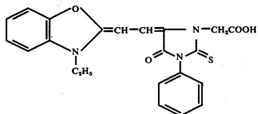
Compound III-16
