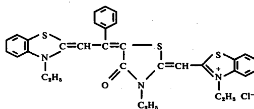
Compound I-16
