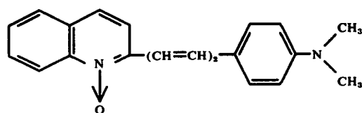
Compound II-16
