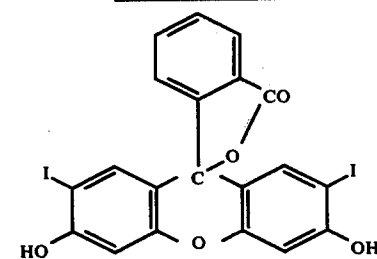
Compound VIII-5
