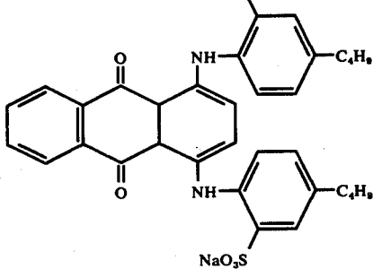
Compound VII-5
