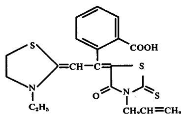
Compound III-19
