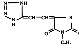
Compound III-20
