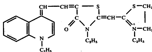
Compound I-13
