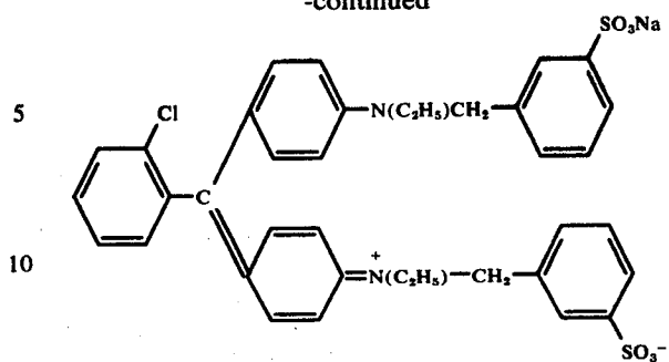
Compound VI-1
