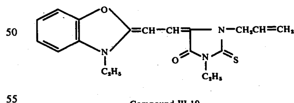
Compound III-10
