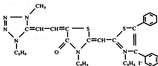
Compound I-7
