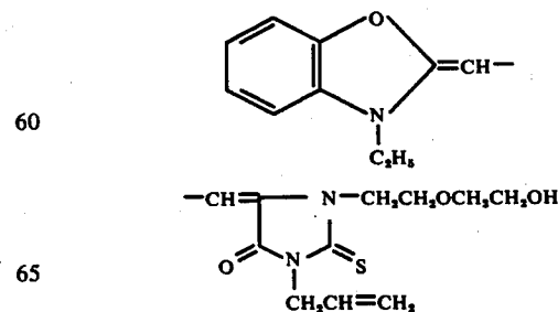
Compound III-10
