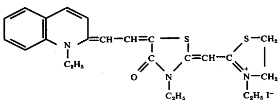
Compound I-11
