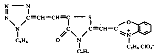
Compound I-15
