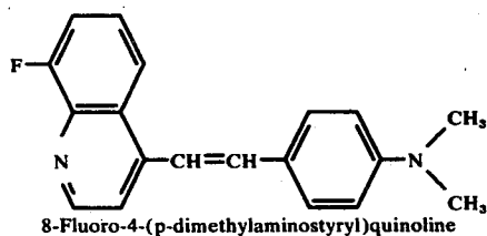
Compound II-11
