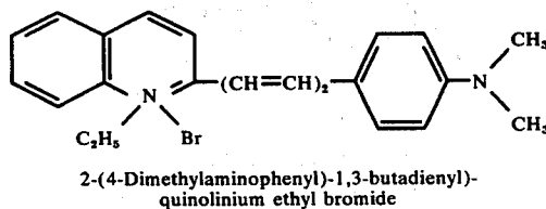
Compound II-23
