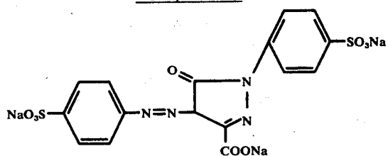
Compound VI-2
