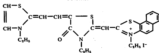
Compound I-5
