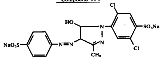
Compound VI-4
