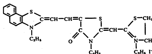
Compound I-3
