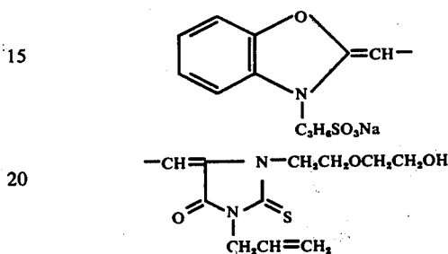
Compound III-6
