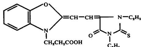
Compound III-14
