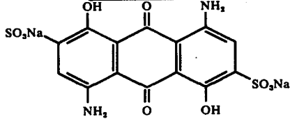
Compound VII-5
