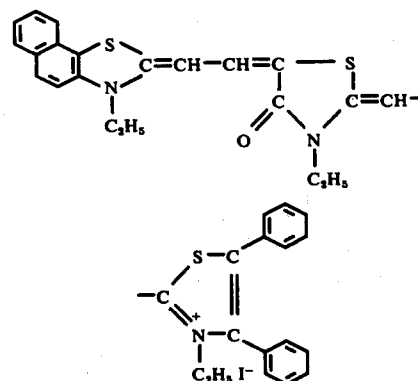
Compound I-4
