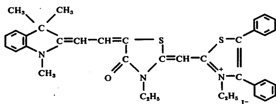
Compound I-9
