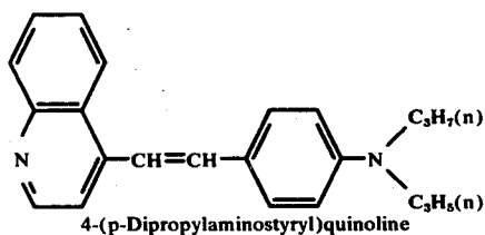
Compound II-12
