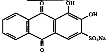
Compound VII-2
