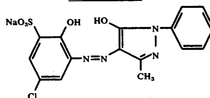
Compound VI-6
