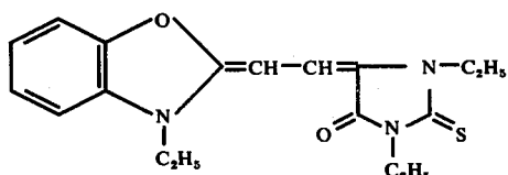
Compound III-12
