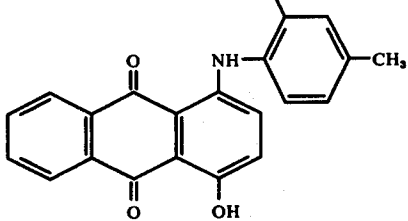
Compound VII-3
