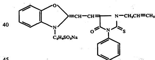
Compound III-8
