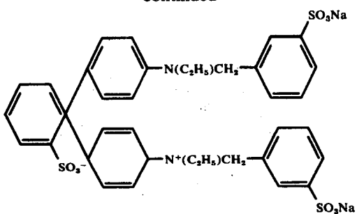
Compound V-5
