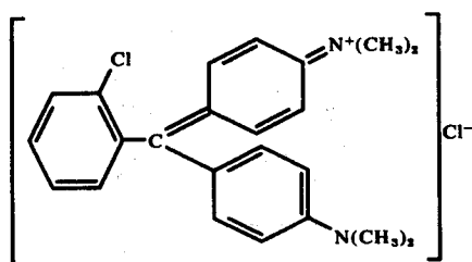
Compound V-9
