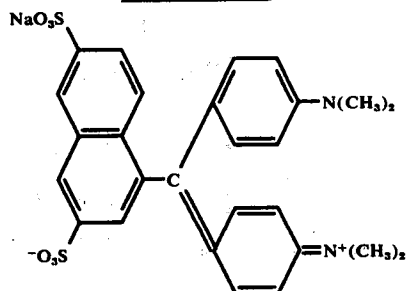
Compound V-6
