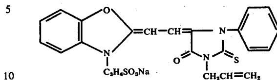
Compound III-5
