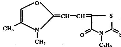
Compound III-20
