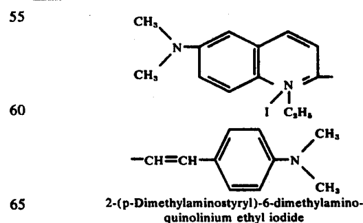
Compound II-22
