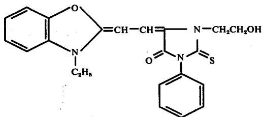
Compound III-15
