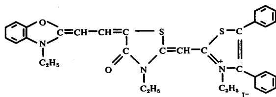
Compound I-10
