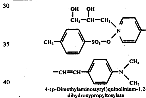
Compound II-20
