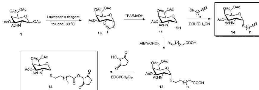
Scheme 47
