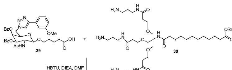
Scheme 10
