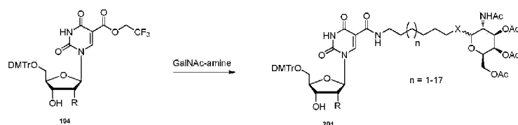
Scheme 35. Synthesis of uridine analogs with GalNAc ligand at C-5 position
