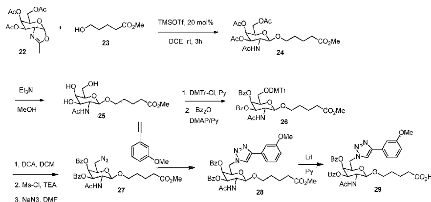
Scheme 9
