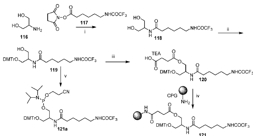
Scheme 99
