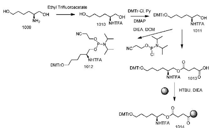
Scheme 76
