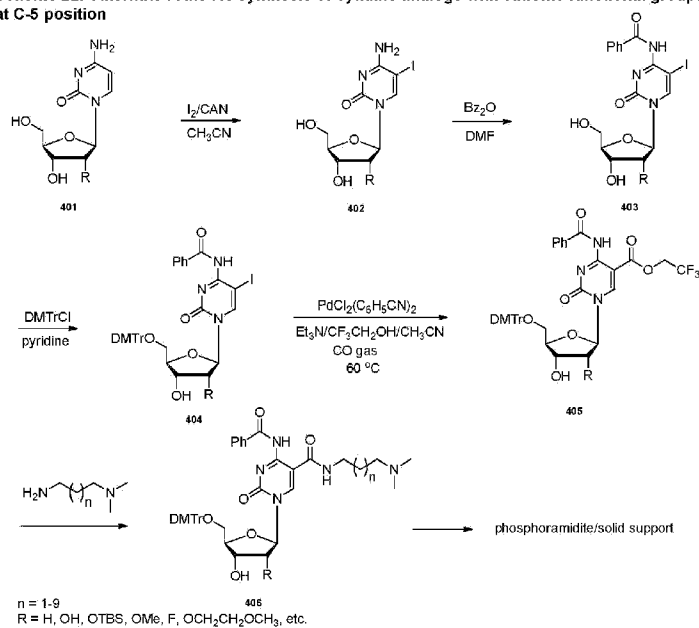
Scheme 23. Synthesis of cytidine analogs with GalNAc ligand at C-5 position
