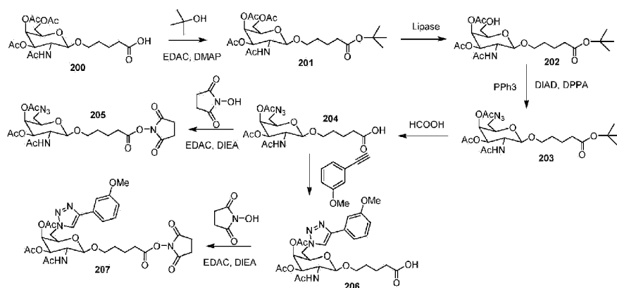
Scheme 110
