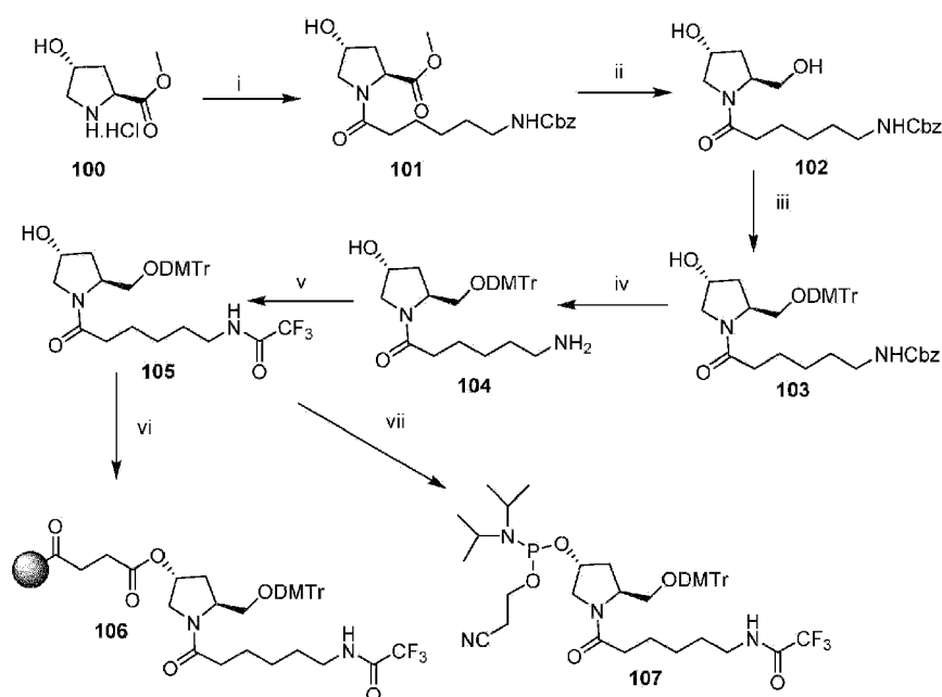
Scheme 98
