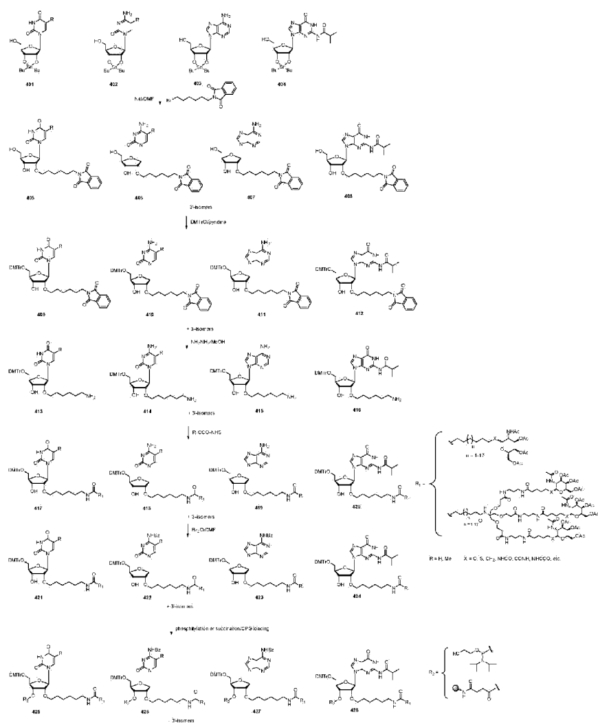
Scheme 38. Synthesis of nucleoside building blocks for GalNAc conjugational 2' position via carbamate linkage.
