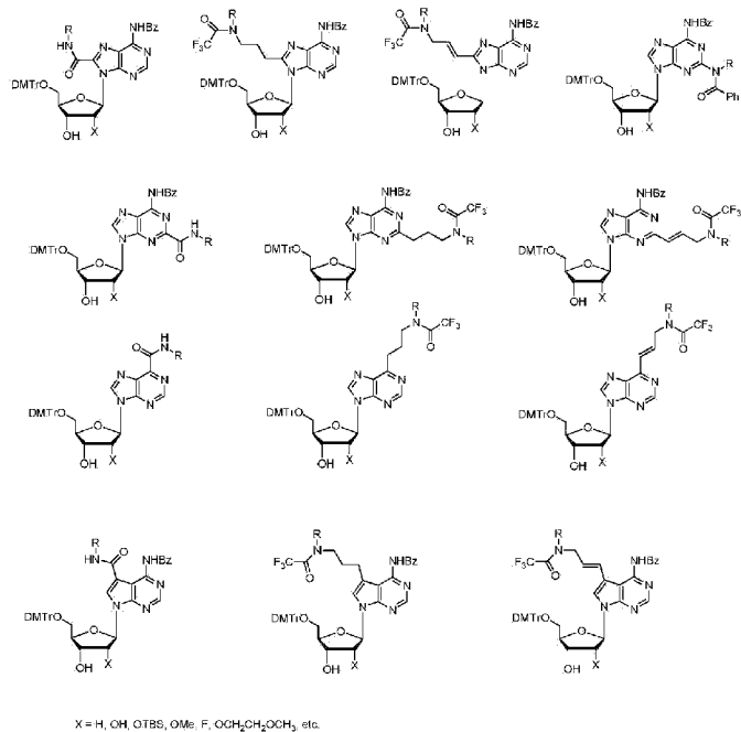
Scheme 28. Adenosine analogs bearing GalNAc targeting ligands
