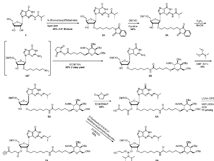
Scheme 123
