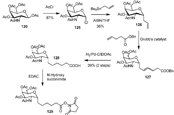
Scheme 86
