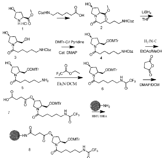
Scheme 17
