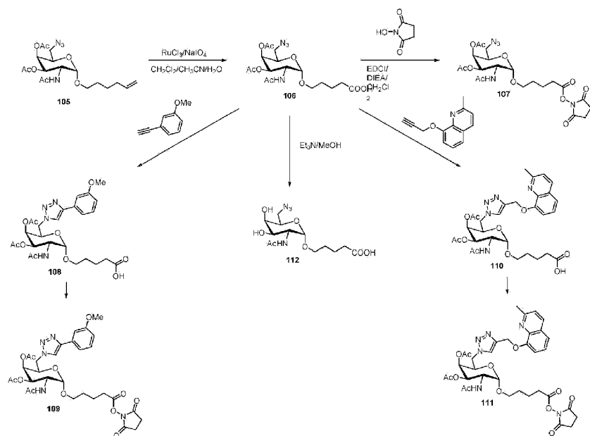
Scheme 107
