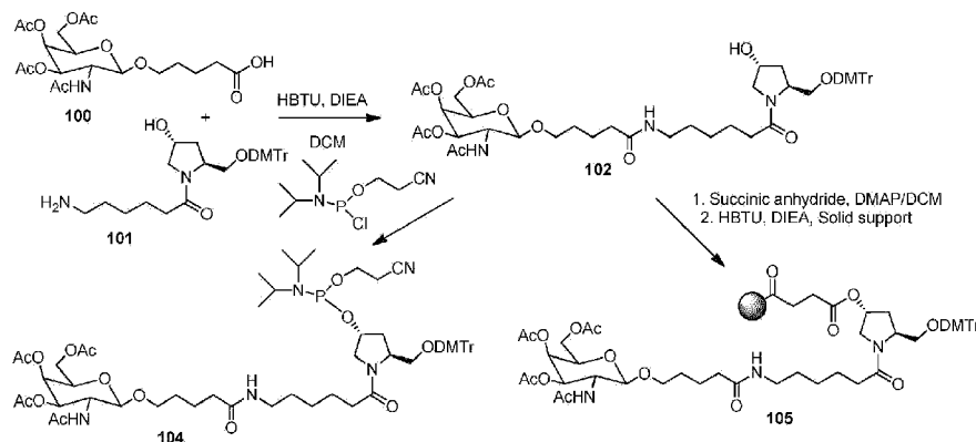
Scheme 80
