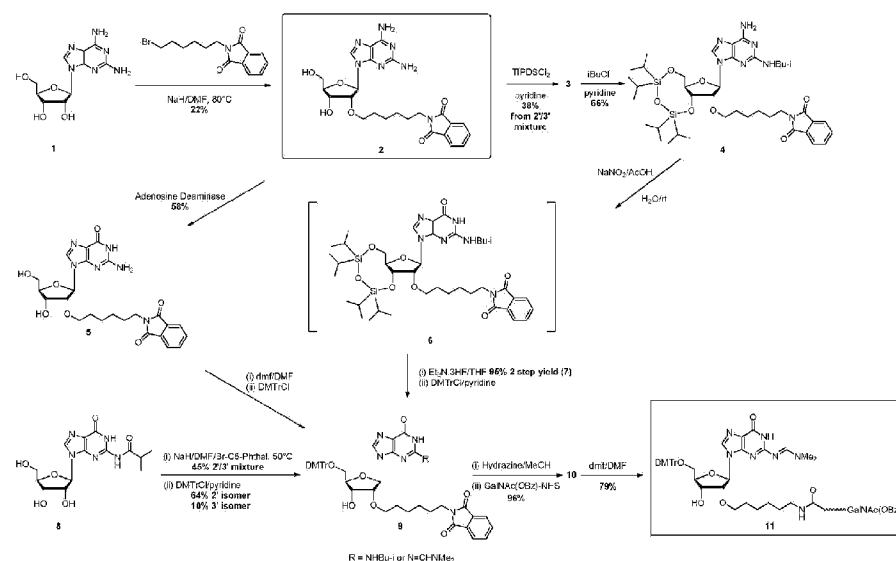
Scheme 125
