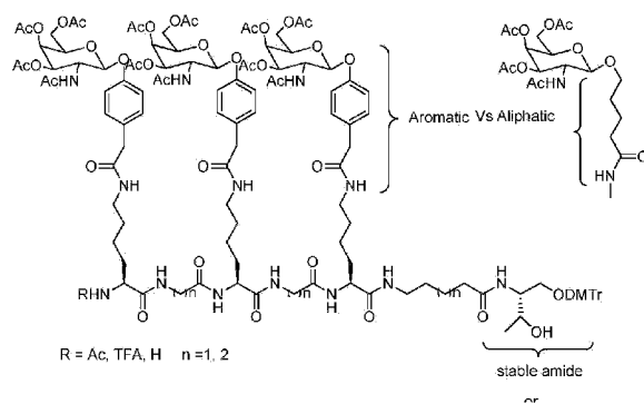
Scheme 72
