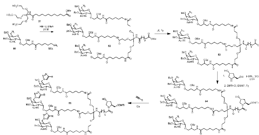
Scheme 15
