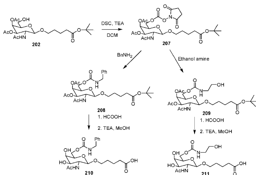
Scheme 111
