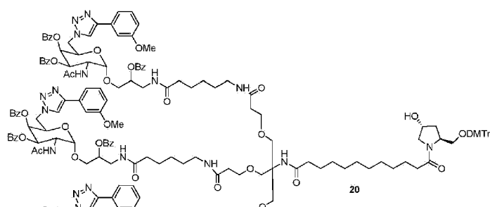
Scheme 8
