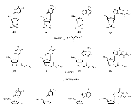
Scheme 42. Synthesis of nucleoside building blocks for post-synthetic GalNac conjugation
