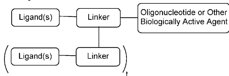
Formula V
