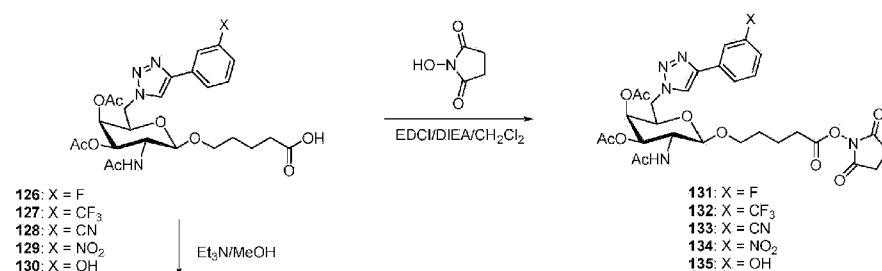
Scheme 109
