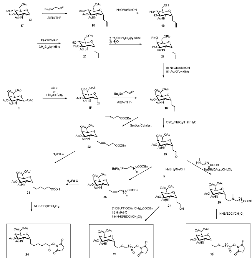
Scheme 47
