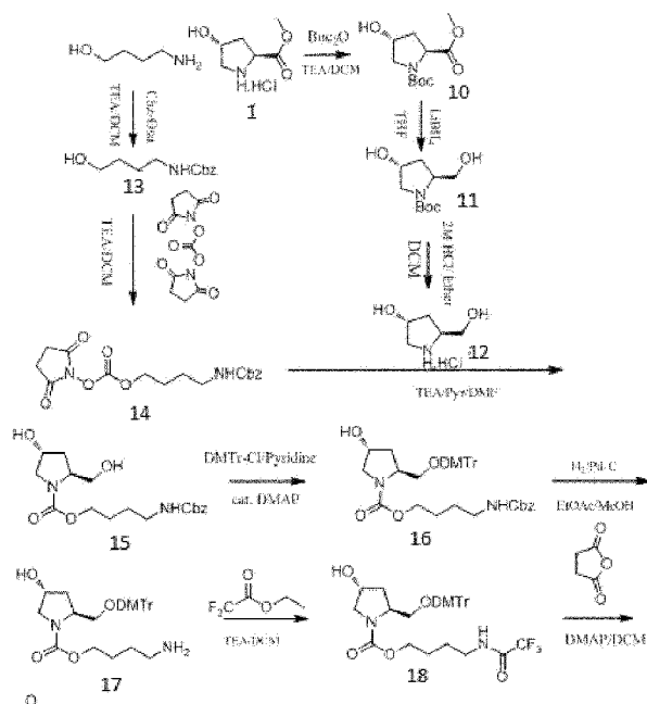
Scheme 18
