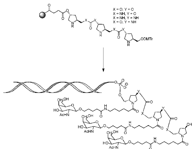
Scheme 69
