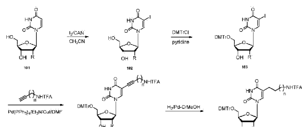
Scheme 24. GalNAc-bearing uridine via C5 alkylamino linker
