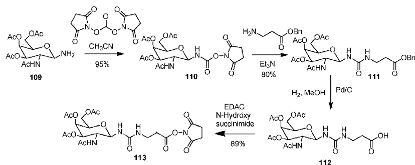
Scheme 83
