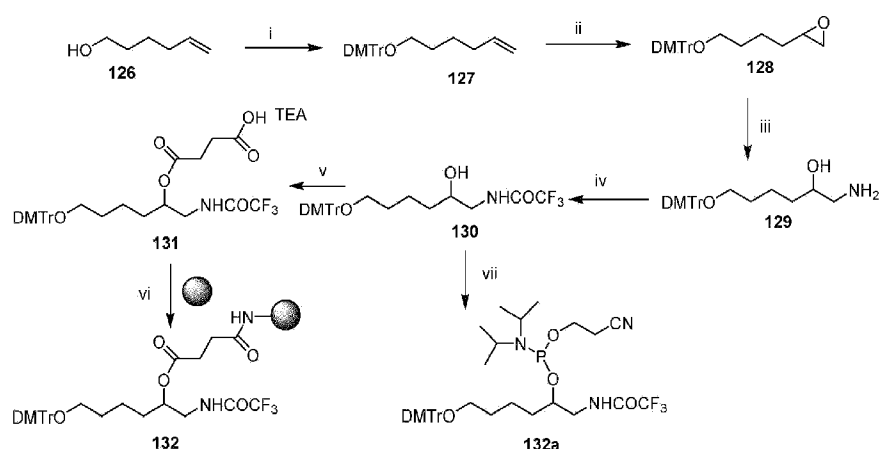
Scheme 101
