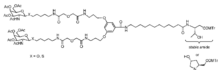
Scheme 68
