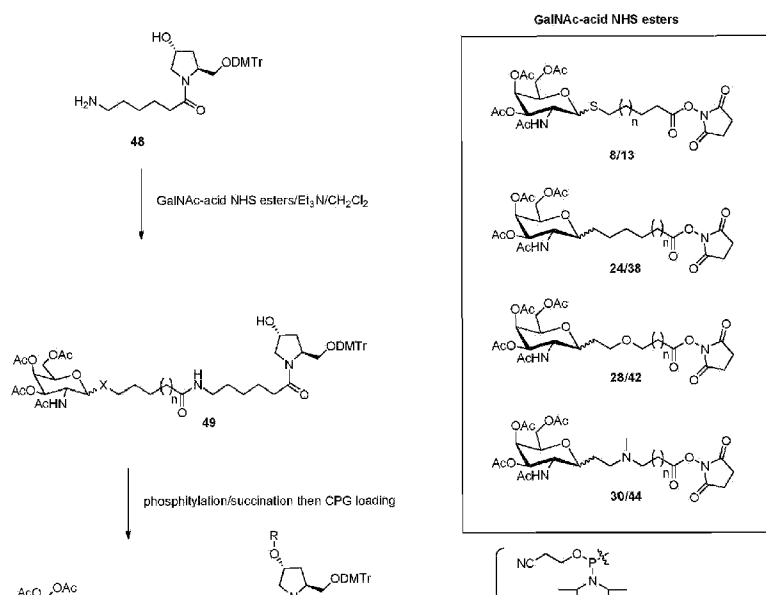
Scheme 50
