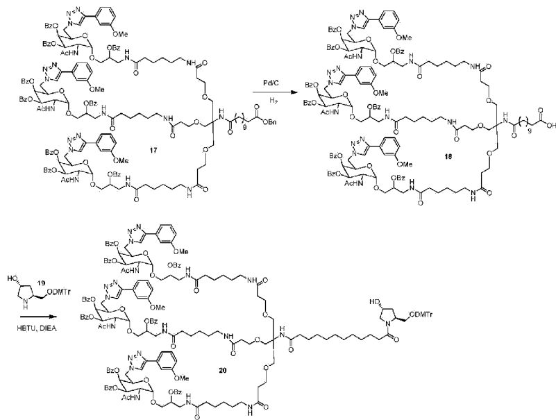
Scheme 7
