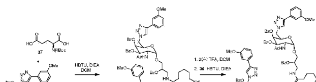
Scheme 12
