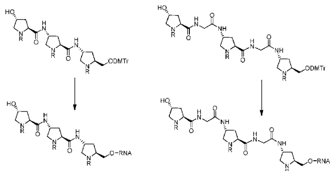
Scheme 67
