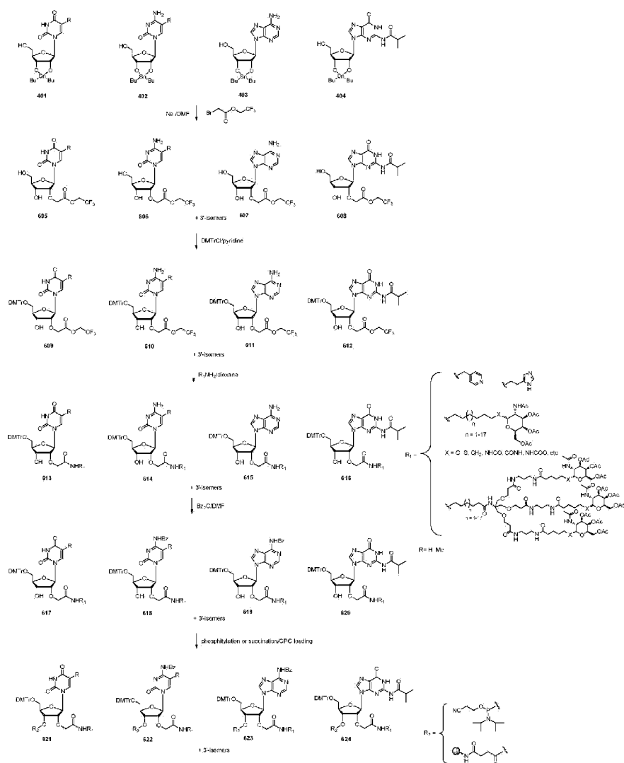
Scheme 42. Synthesis of nucleoside building blocks for post-synthetic GalNac conjugation
