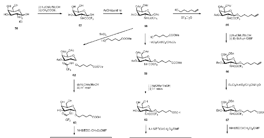
Scheme 52
