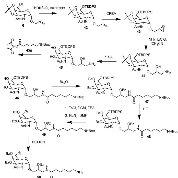
Scheme 14
