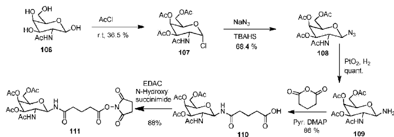
Scheme 82
