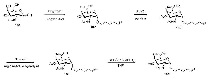
Scheme 106
