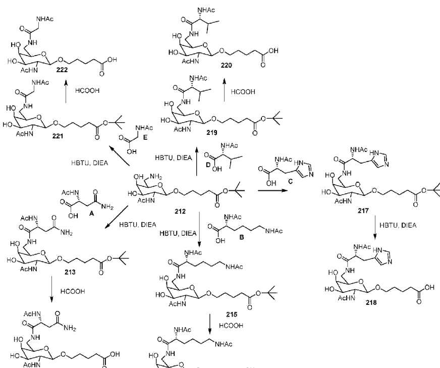
Scheme 112
