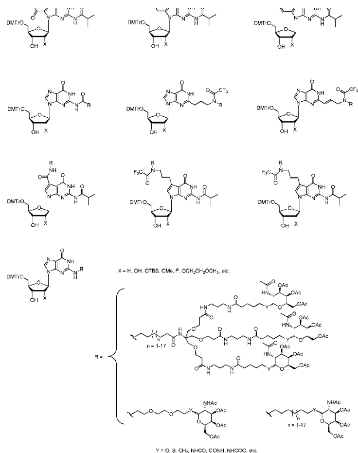
Scheme 30. Synthesis of GalNAc ligand at abasic site
