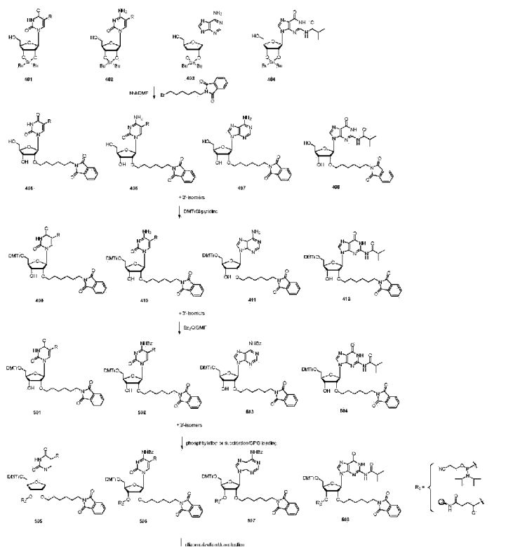
Scheme 40. Synthesis of nucleoside building blocks for post-synthetic GelBac conjugation
