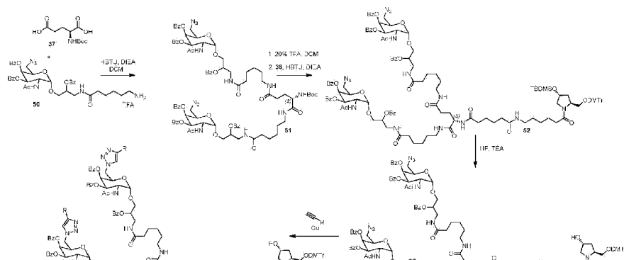
Scheme 14
