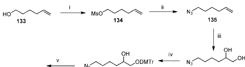
Scheme 102
