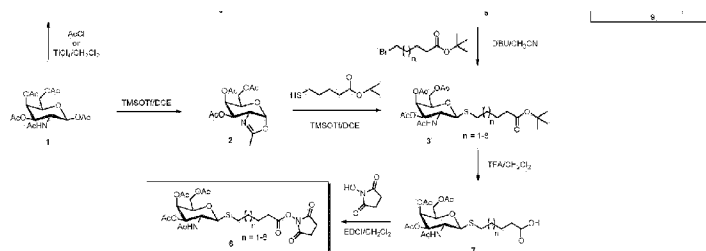
Scheme 46
