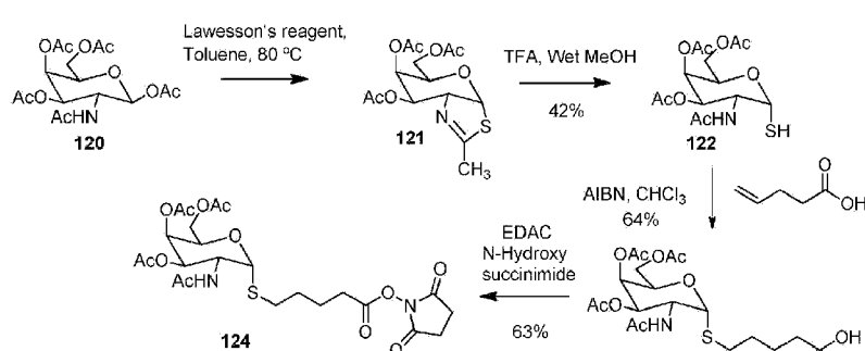
Scheme 84
