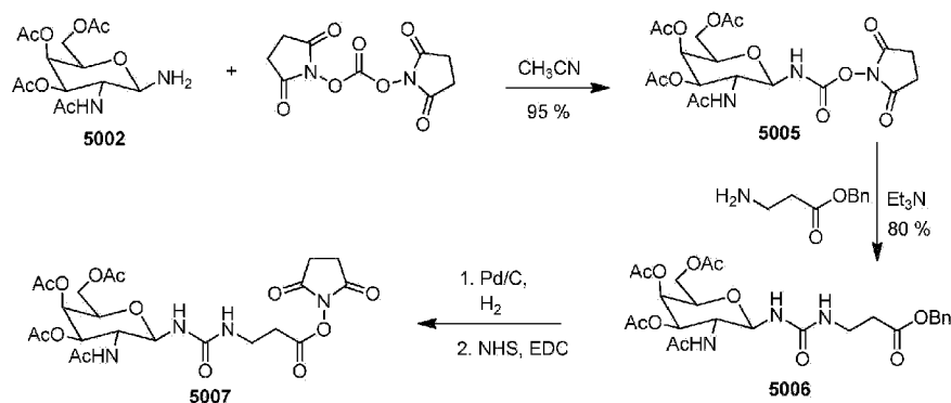
Scheme 88
