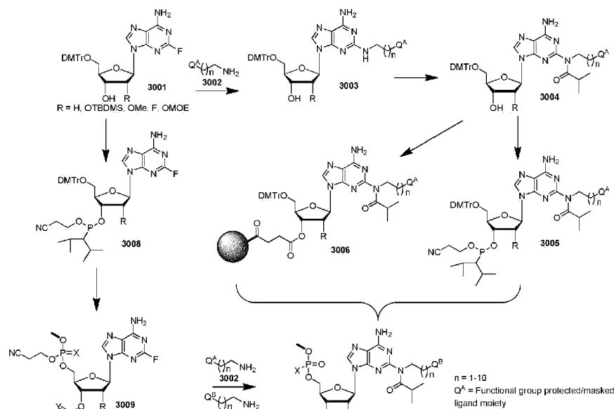
Scheme 78
