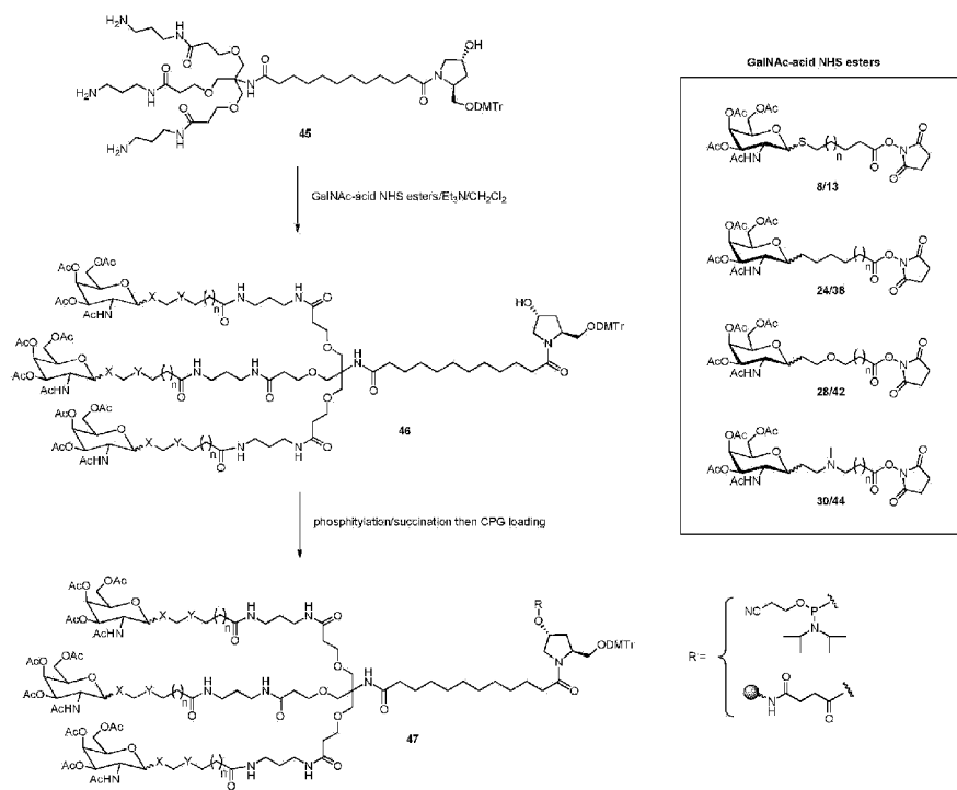
Scheme 50
