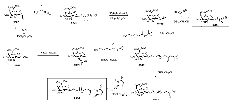
Scheme 89
