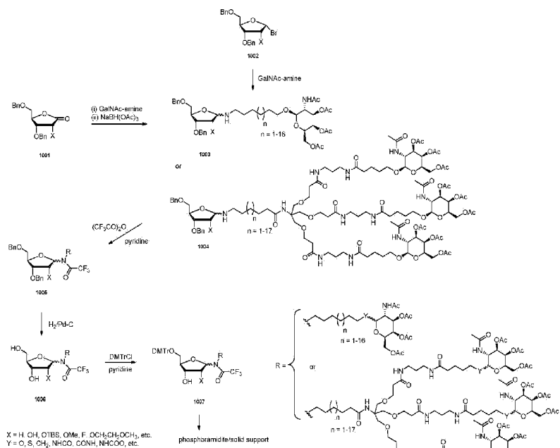
Scheme 30. Synthesis of GalNAc ligand at abasic site
