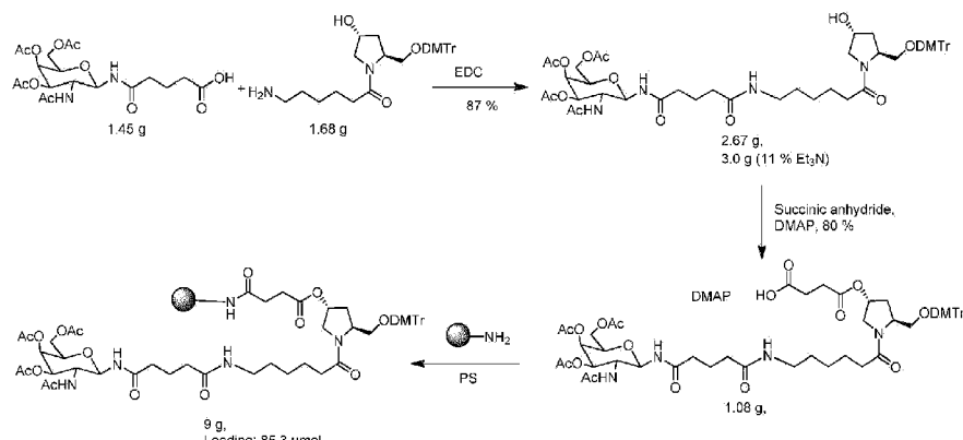
Scheme 58
