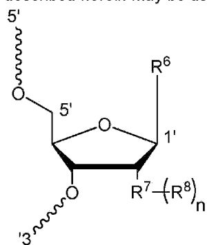
Formula VII
