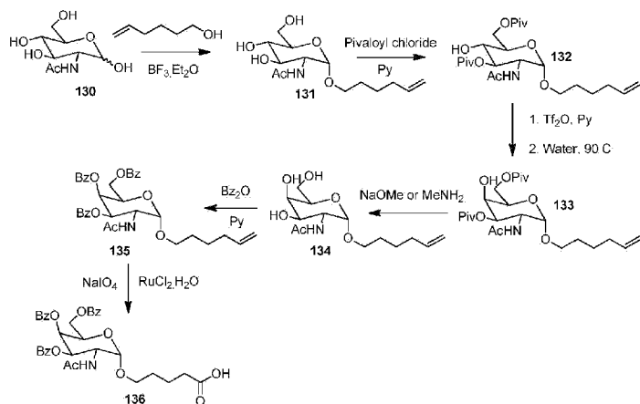
Scheme 86
