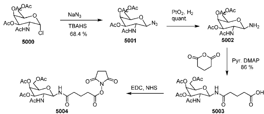
Scheme 87
