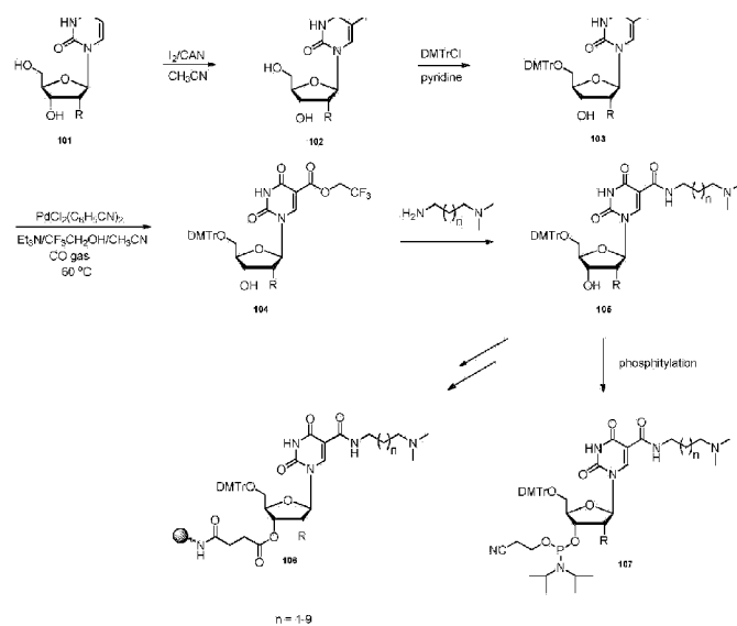
Scheme 20. Synthesis of uridine analogs with GalNAc ligand at C-5 position
