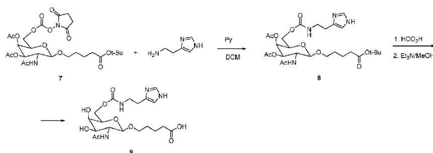
Scheme 105
