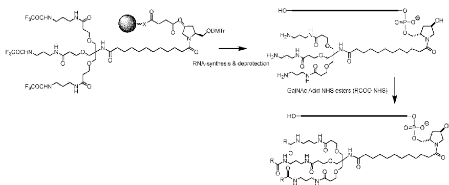
Scheme 94
