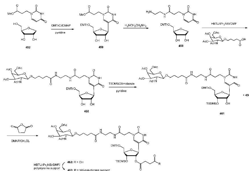
Scheme 56
