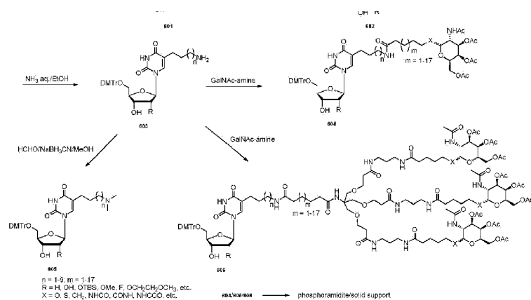
Scheme 25. GalNAc-bearing cytidine via C5 alkylamino linker
