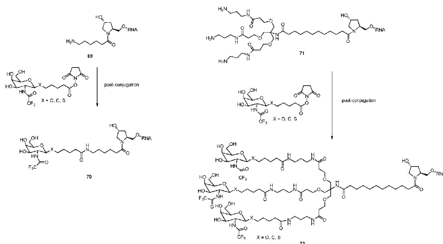
Scheme 53
