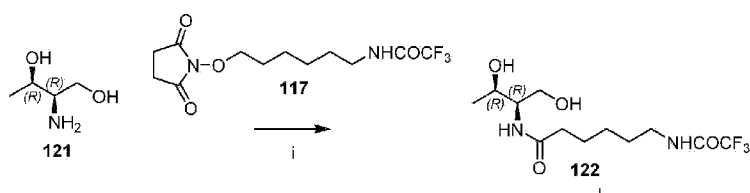
Scheme 100
