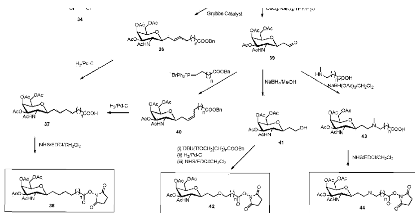
Scheme 49
