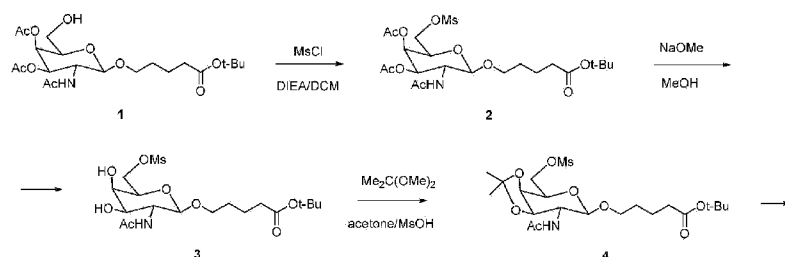
Scheme 104
