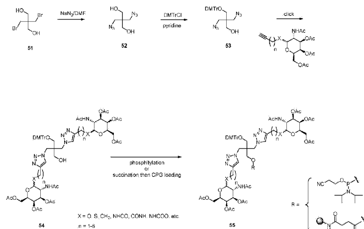
Scheme 51
