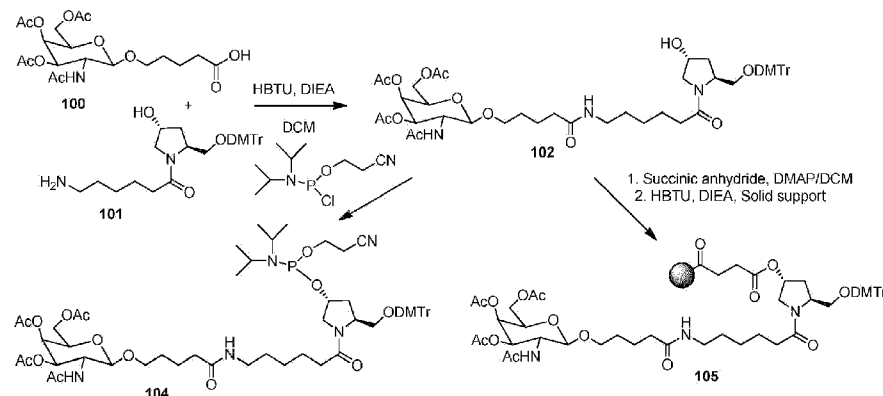
Scheme 97
