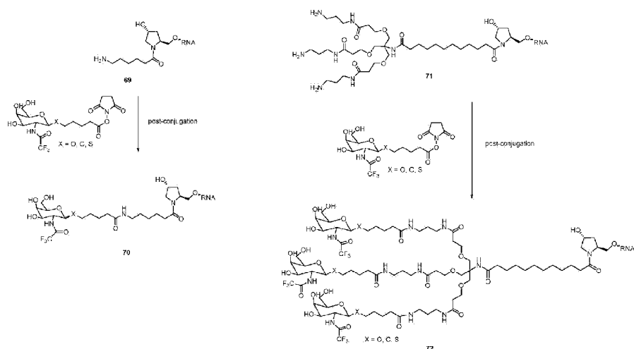
Scheme 114
