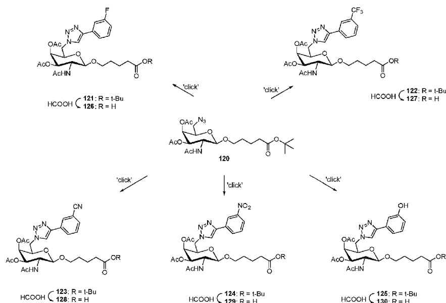
Scheme 108
