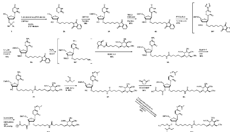
Scheme 121
