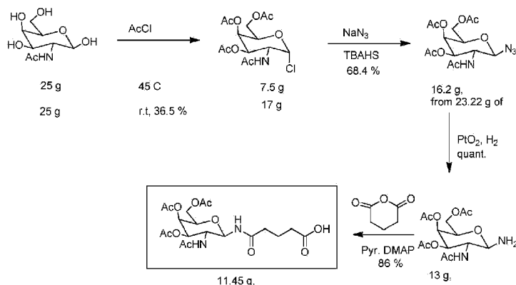
Scheme 58
