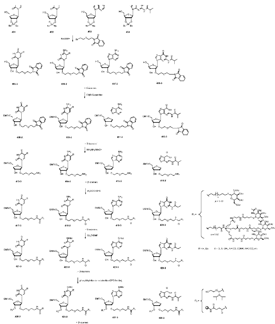
Scheme 40. Synthesis of nucleoside building blocks for post-synthetic GelBac conjugation
