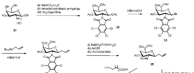
Scheme 48
