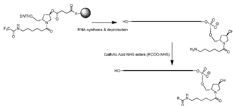
Scheme 96
