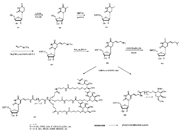
Scheme 27. GalNAc-bearing cytidine via C5 alkylamino linker
