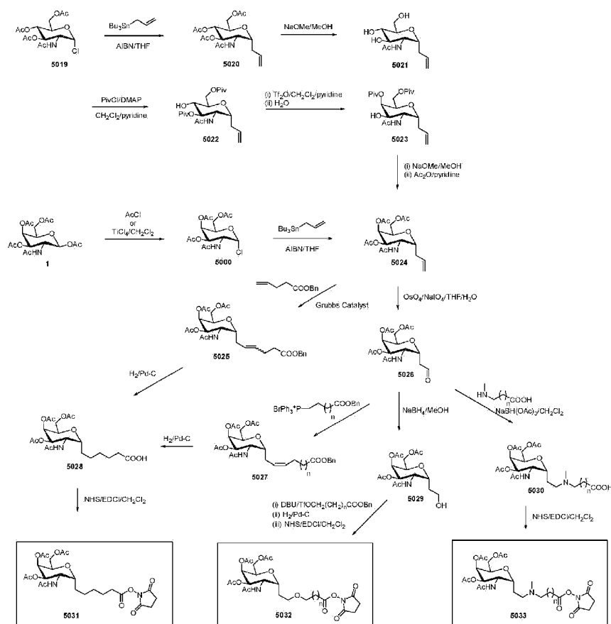
Scheme 91
