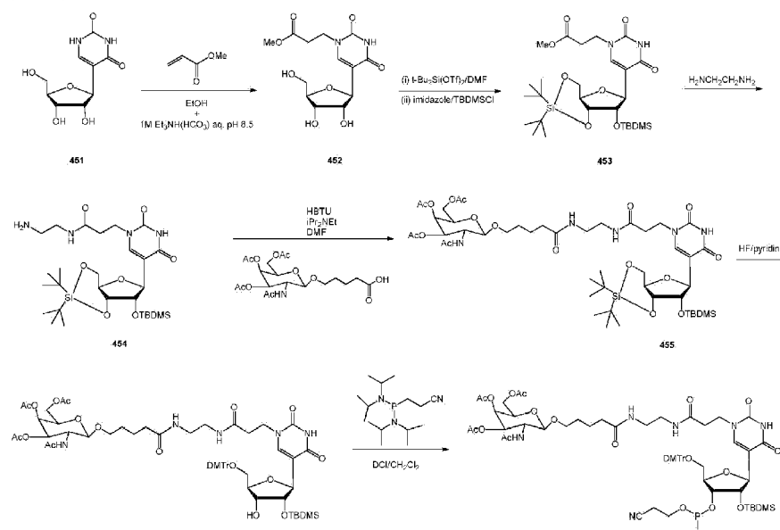
Scheme 55
