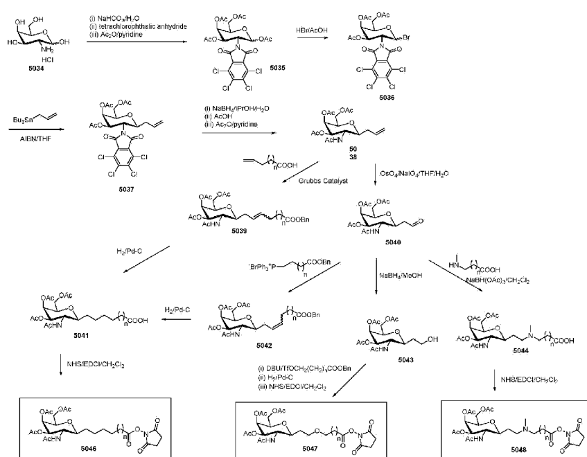
Scheme 92
