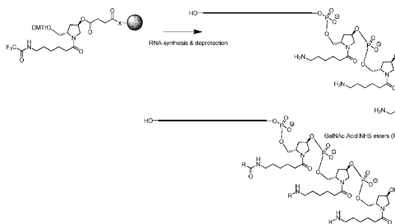
Scheme 96
