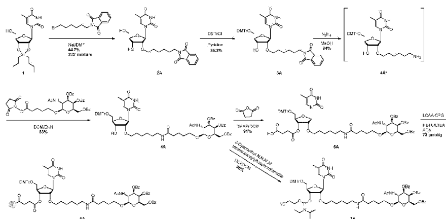
Scheme 117
