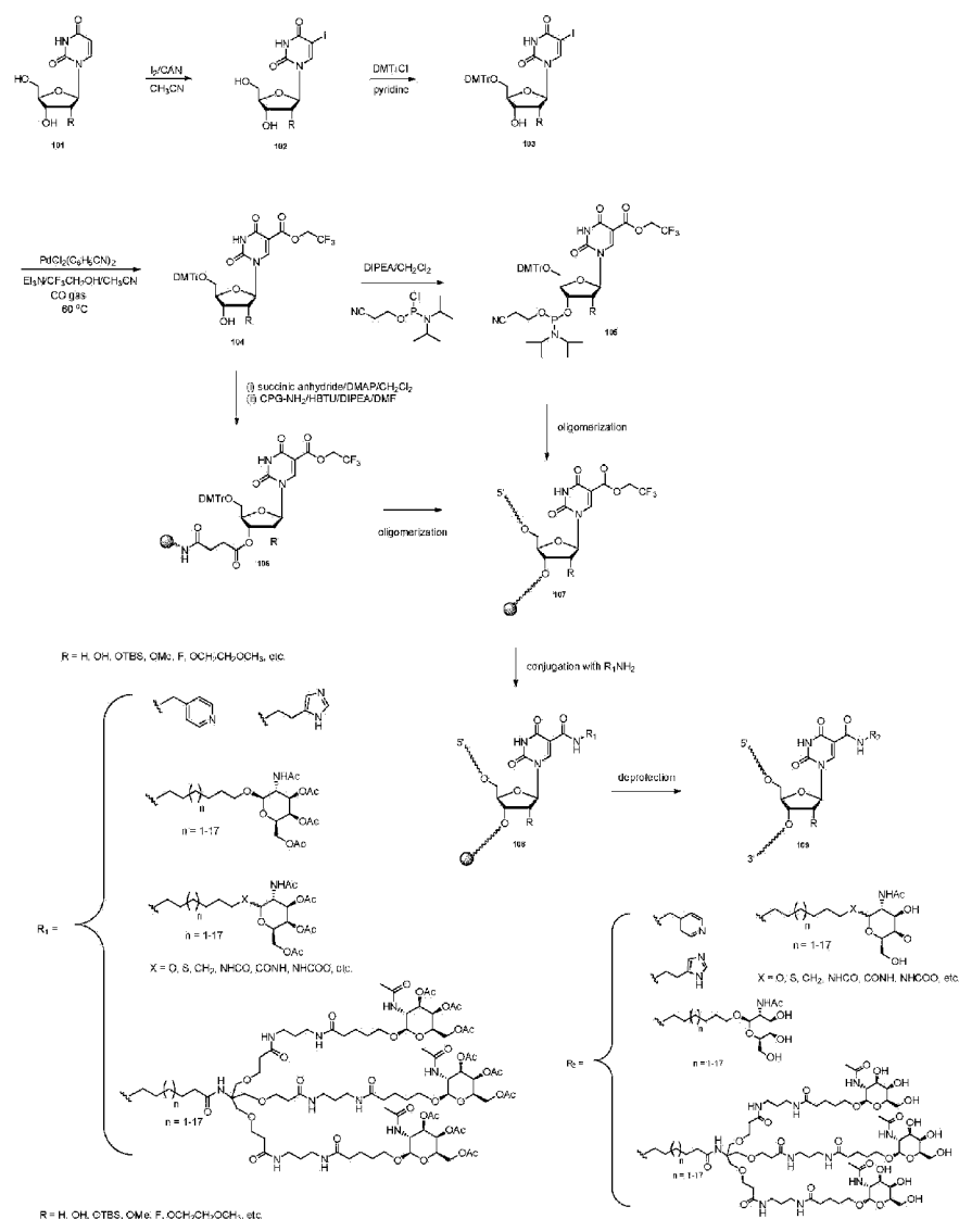
Scheme 35. Synthesis of uridine analogs with GalNAc ligand at C-5 position
