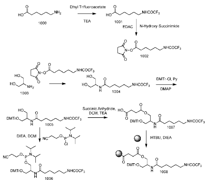
Scheme 75
