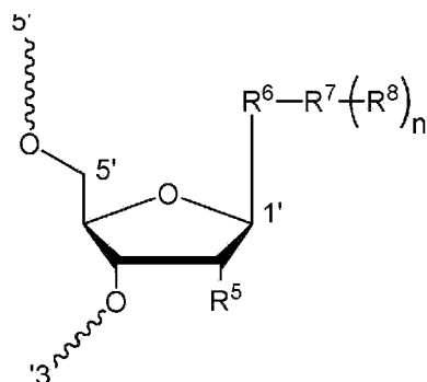
Formula VI
