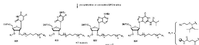
Scheme 44. Synthesis of 2'-O-Alkyl-GalNAc Nucleoside Derivatives
