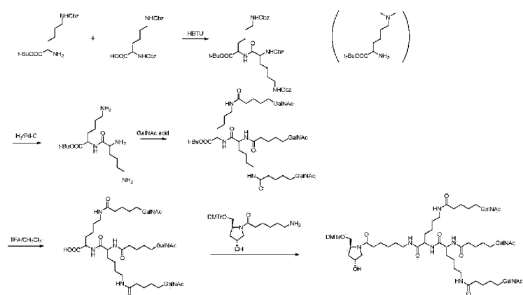
Scheme 73
