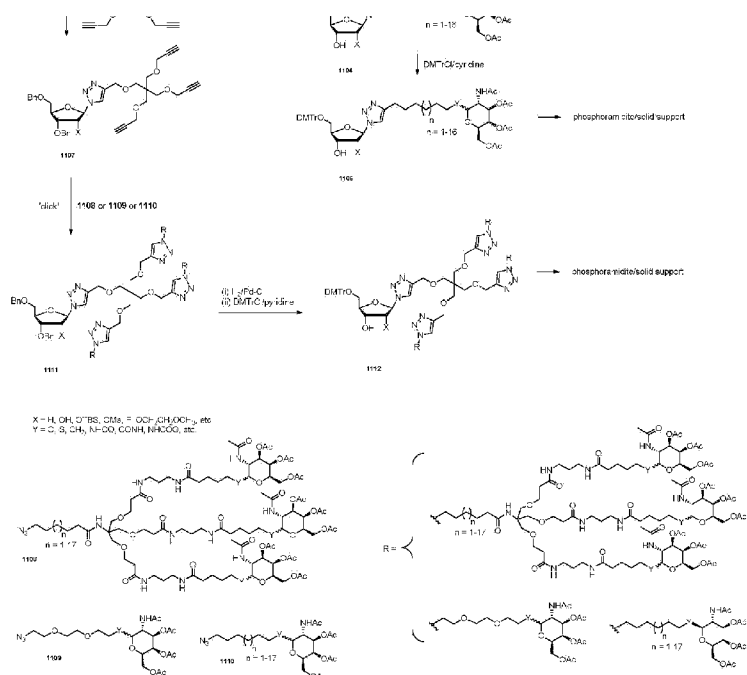
Scheme 32. Synthesis of GalNAc ligand at abasic site by click reaction-2
