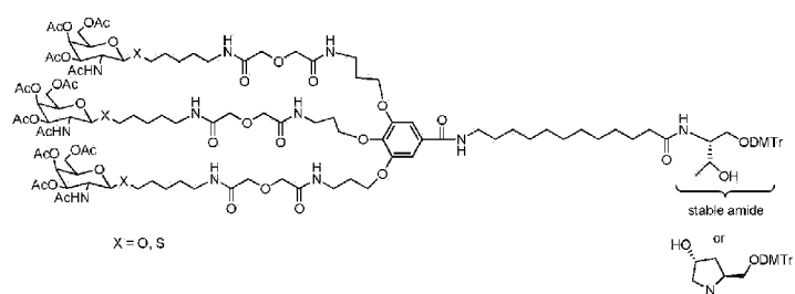
Scheme 67
