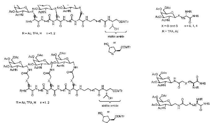
Scheme 70
