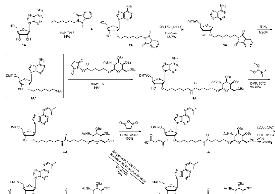
Scheme 119
