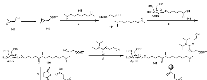
Scheme 103
