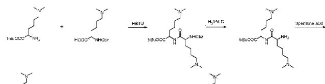
Scheme 73
