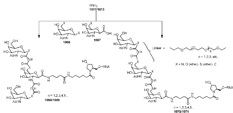
Scheme 77
