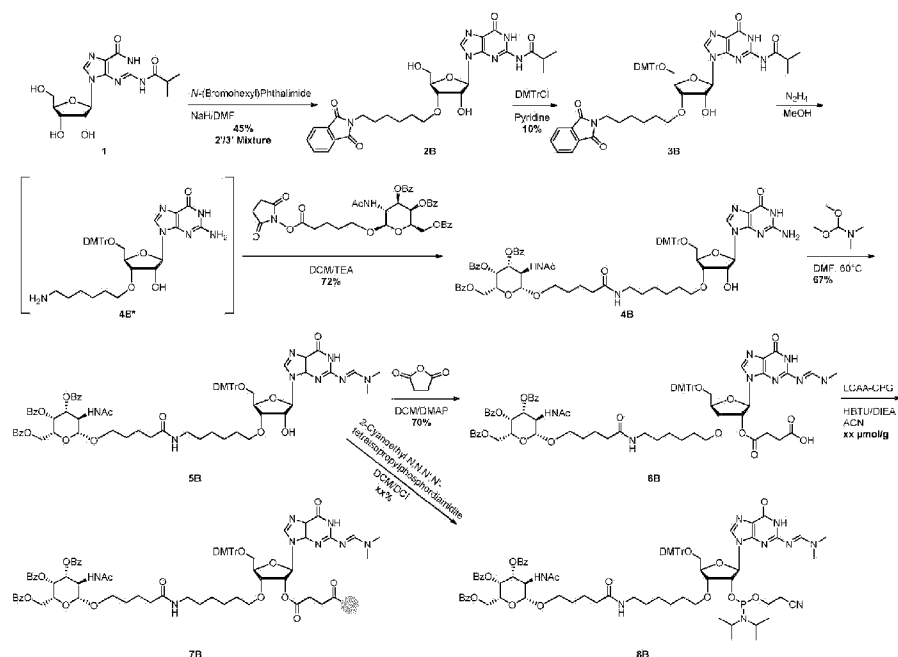
Scheme 124
