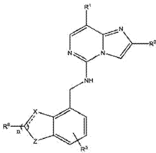
Formel (I)
