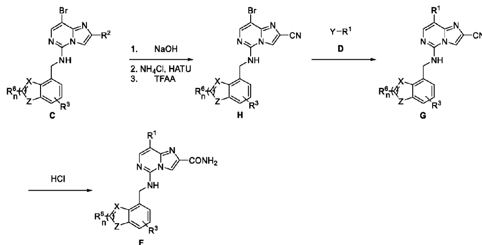
General Reaction Scheme II
