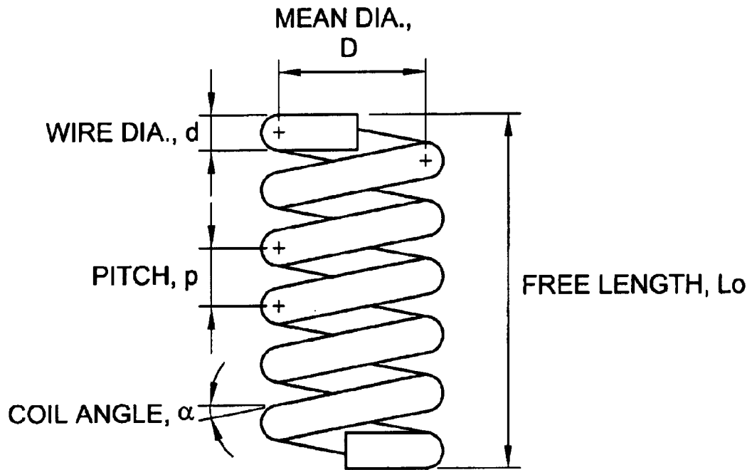
Figure 1, Conventional Compression Spring
