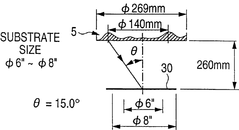
CONFIGURATION OF LOW-PRESSURE LONG-DISTANCE SPUTTERING
