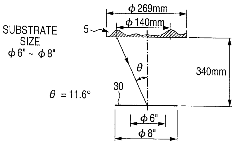
CONFIGURATION OF LOW-PRESSURE LONG-DISTANCE SPUTTERING
