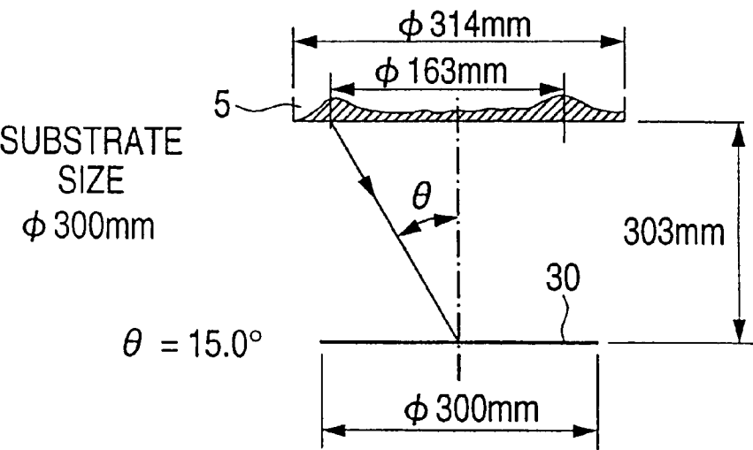
CONFIGURATION OF LOW-PRESSURE LONG-DISTANCE SPUTTERING
