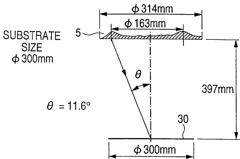
CONFIGURATION OF LOW-PRESSURE LONG-DISTANCE SPUTTERING
