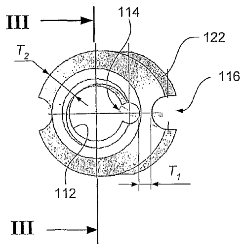
VIEW II
