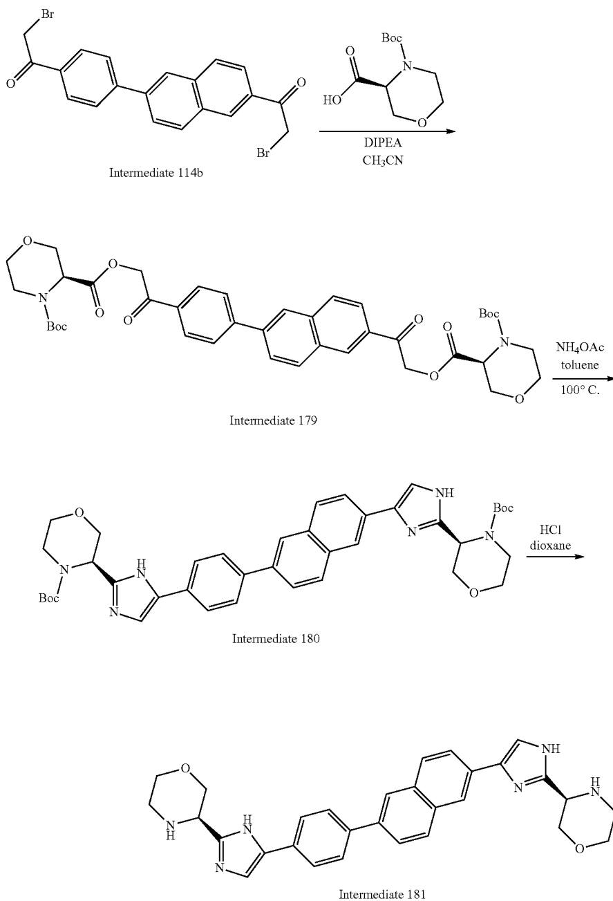
Scheme 46
