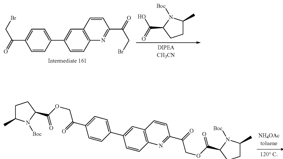
Scheme 42
