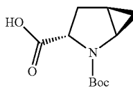
(1R,3S,5R)-2-(tert-Butoxycarbonyl)-2-azabicyclo[3.1.0]hexane-3-carboxylic acid
