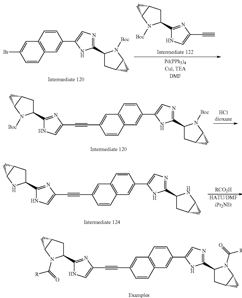
Scheme 32
