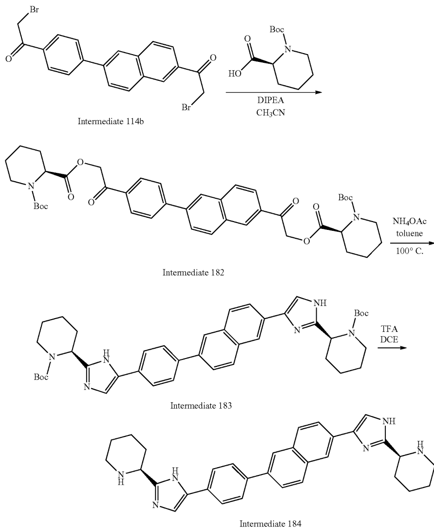
Scheme 47
