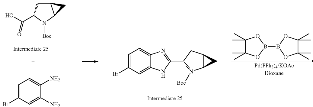
Scheme 6
