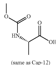
(S)-2-(Methoxycarbonylamino)propanoic acid
