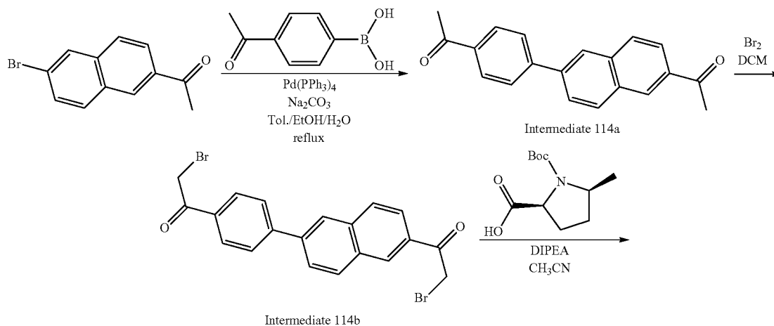
Scheme 29
