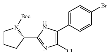
(S)-tert-Butyl 2-(5-(4-bromophenyl)-4-chloro-1H-imidazol-2-yl)pyrrolidine-1-carboxylate
