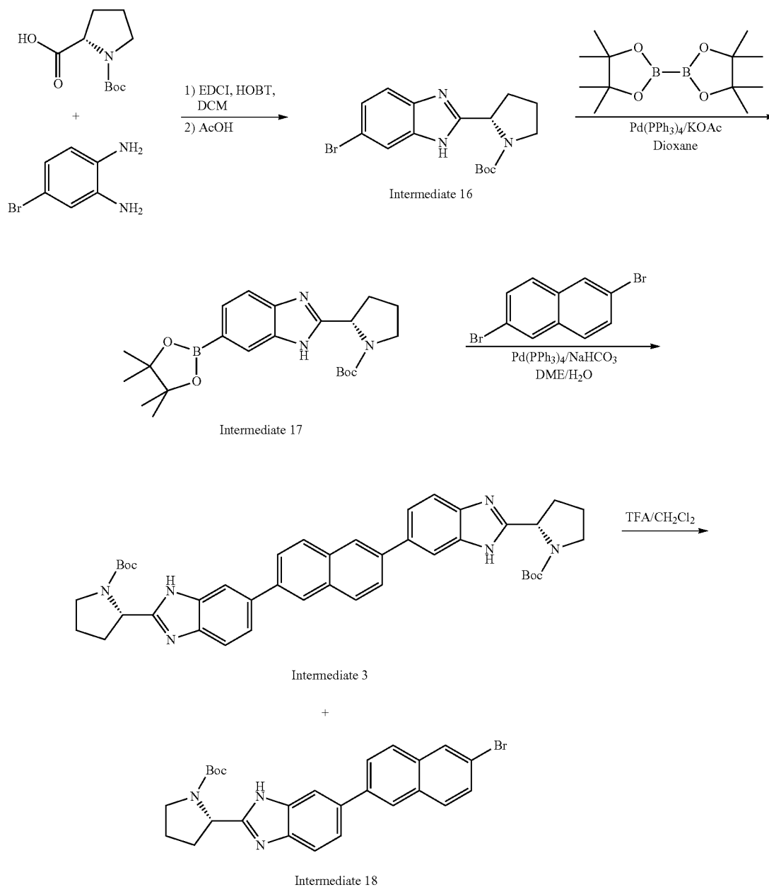
Scheme 3
