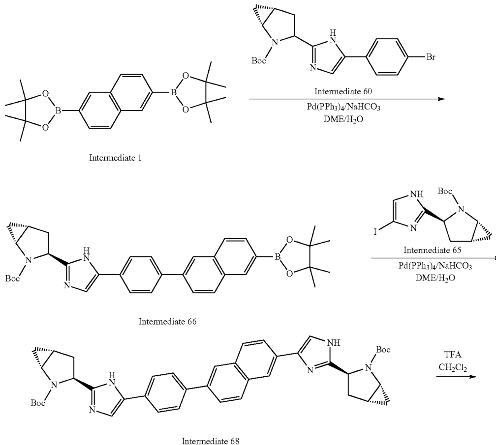
Scheme 15
