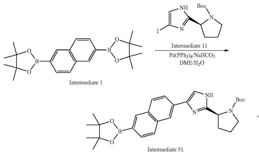
Scheme 11
