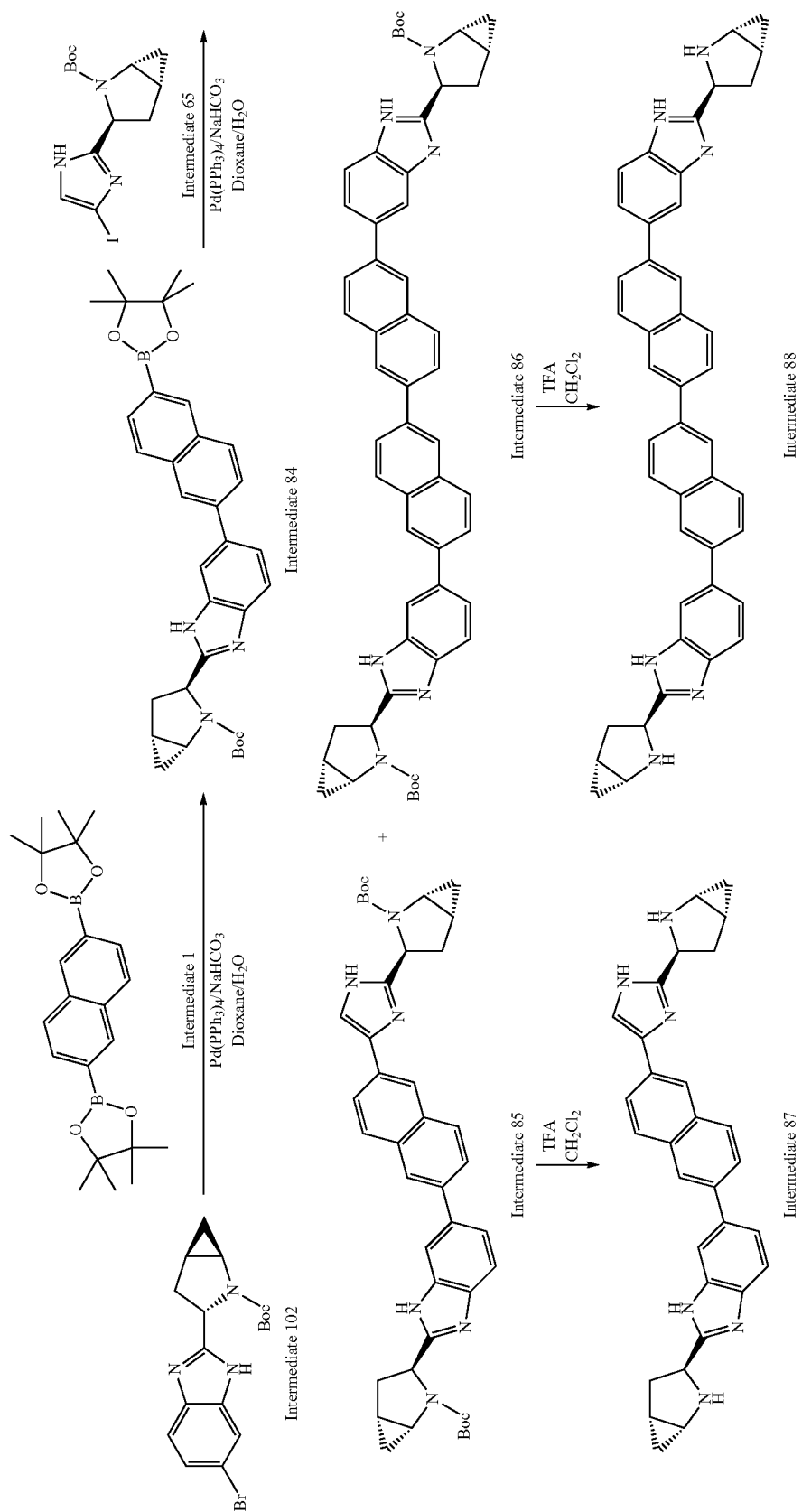
Scheme 21
