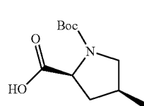
(2S,4S)-1-(tert-Butoxycarbonyl)-4-methylpyrrolidine-2-carboxylic acid
