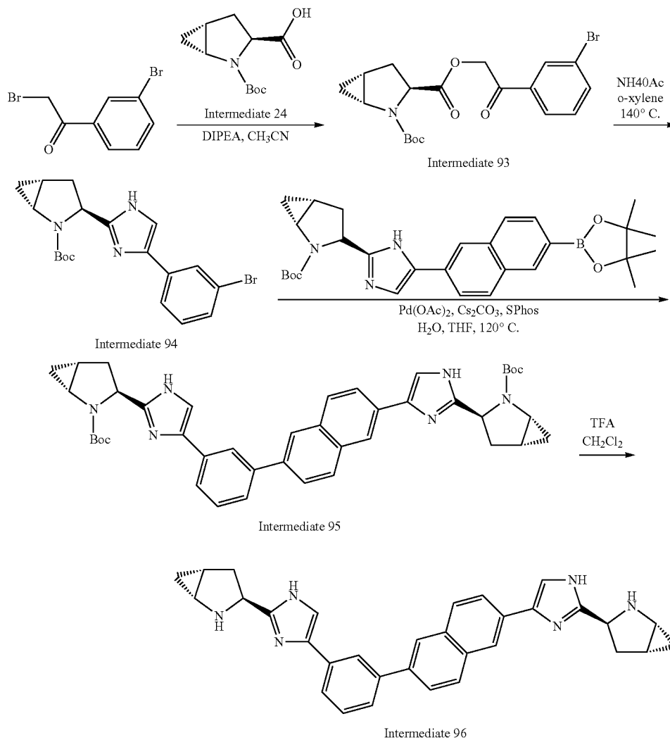
Scheme 24
