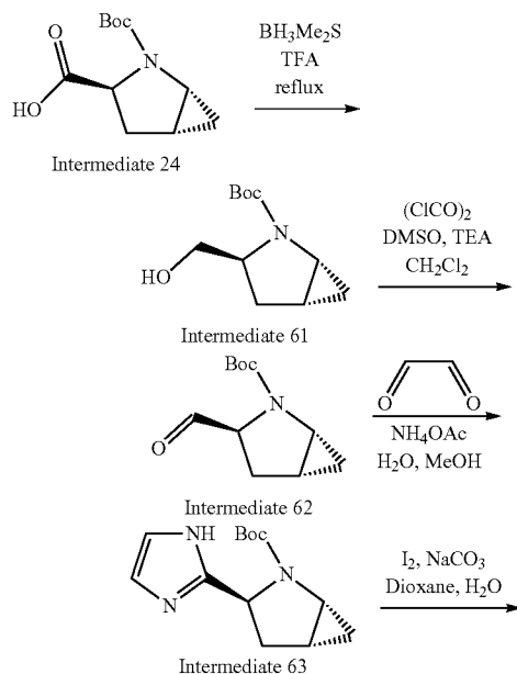
Scheme 14
