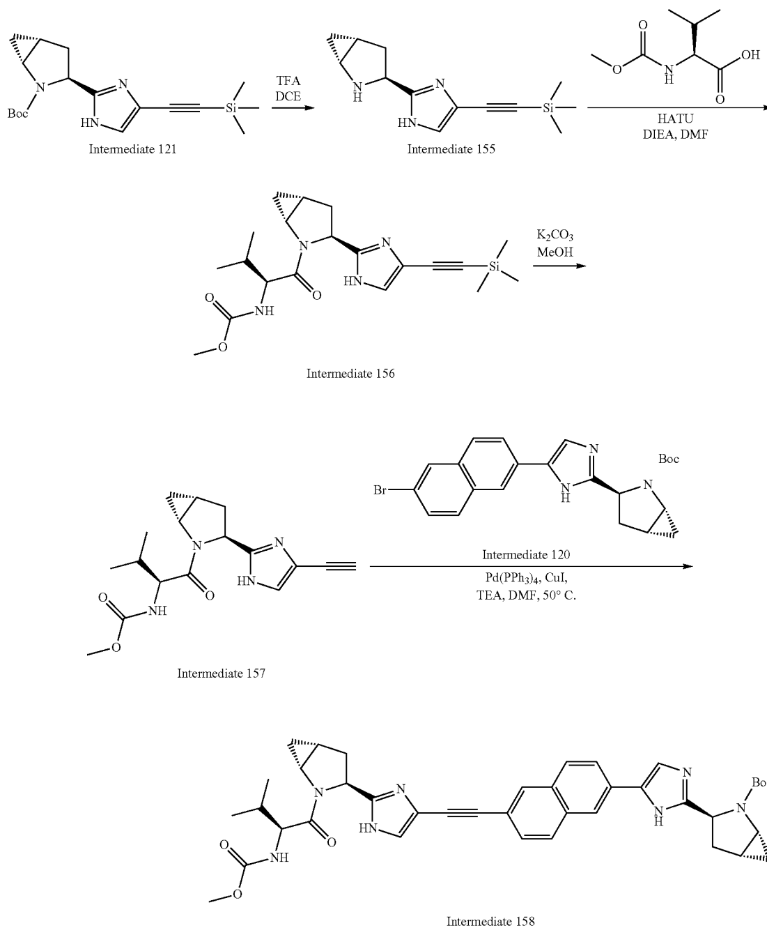
Scheme 40
