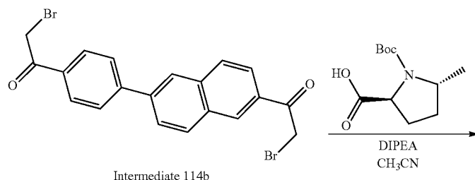
Scheme 48
