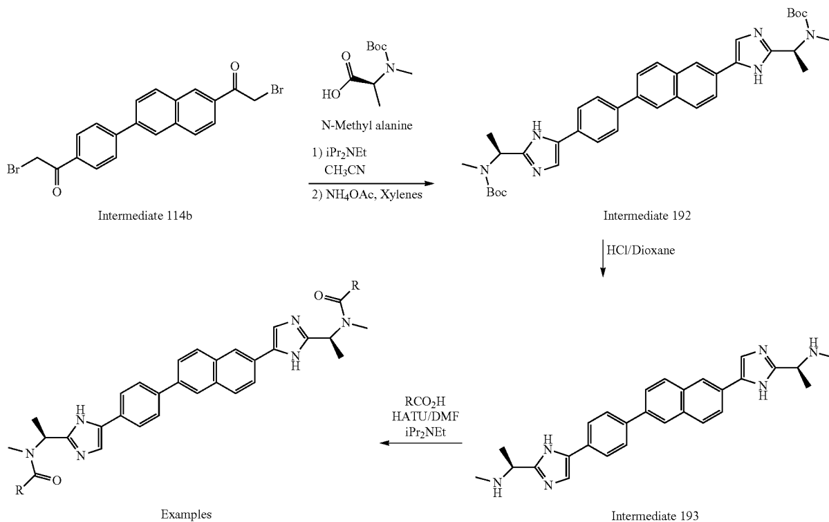
Scheme 51
