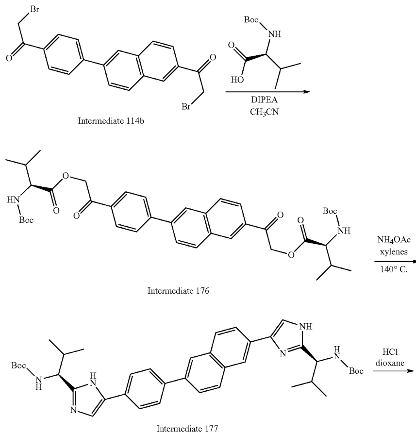
Scheme 45
