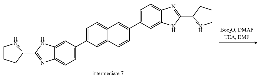
Scheme 10
