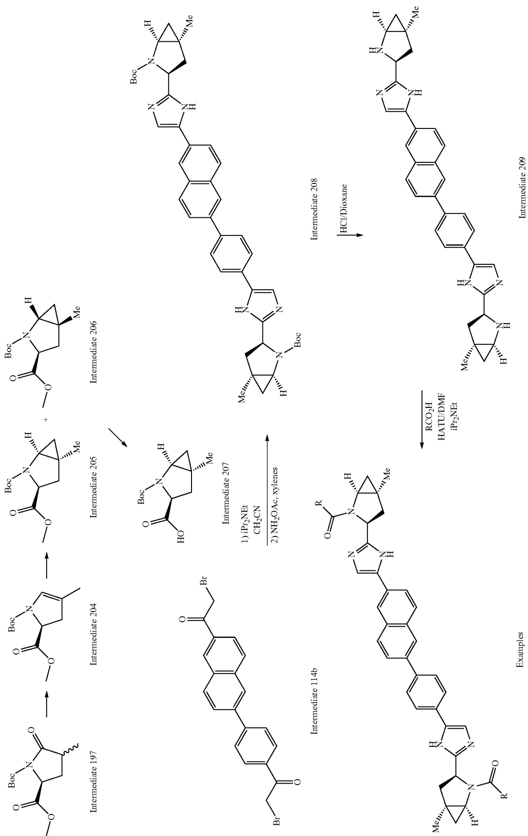
Scheme 55
