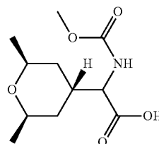
Racemic mixture
