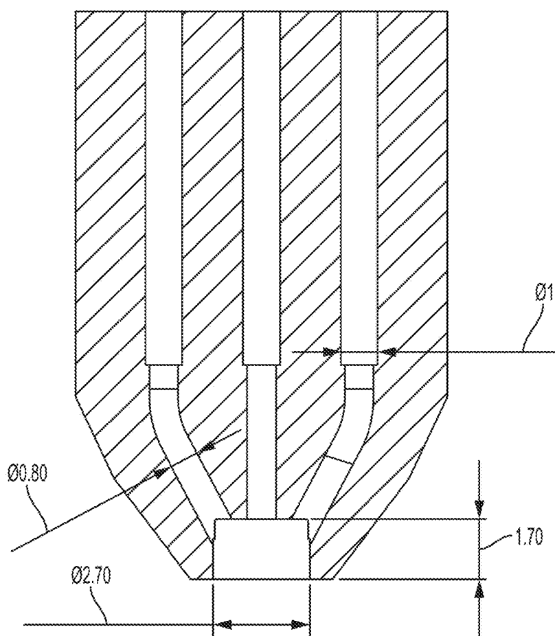
SECTION B-B FIG. 1F
