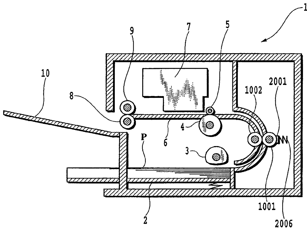
FIG.19 (PRIOR ART)
