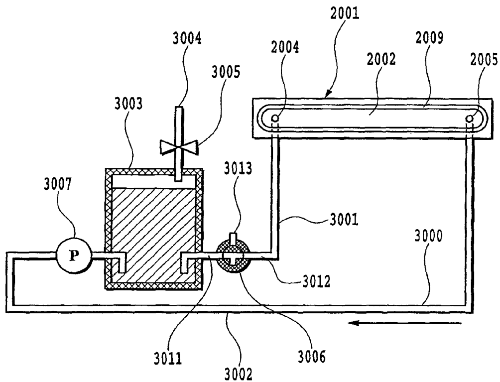
FIG.11 (PRIOR ART)
