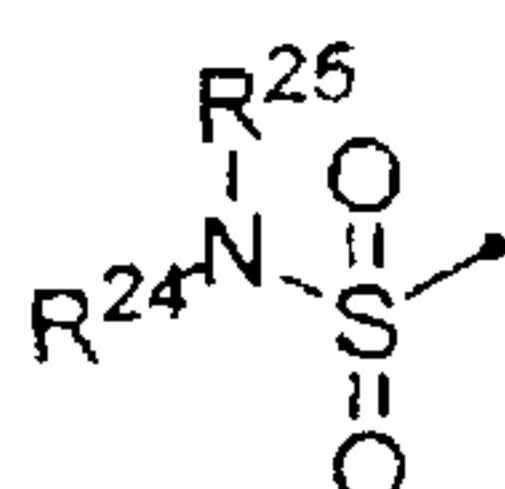
Sulfamoyl group
