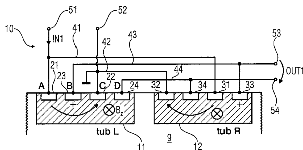
Clock phase 1: cross-section
