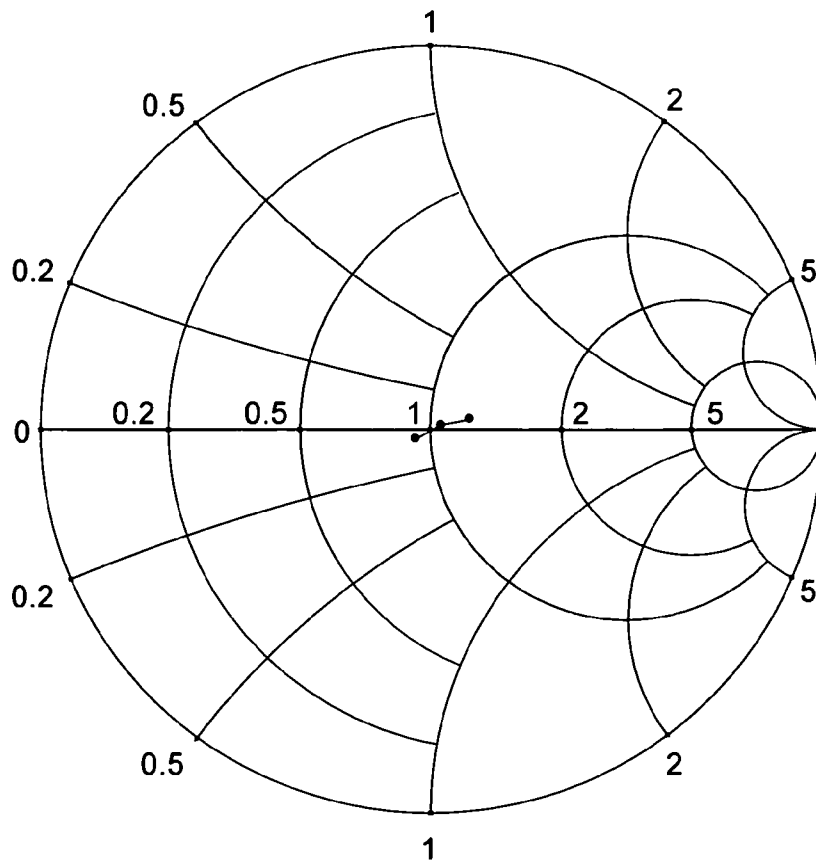
IMPEDANCE LOCUS, 36.7-37.0 GHz
