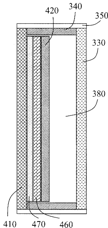
SECTION X-X
