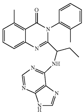
5-Methyl-2-(1-(9H-purin-6-ylamino)propyl)-3-o-tolyl-3H-quinazolin-4-one (D-081b)
