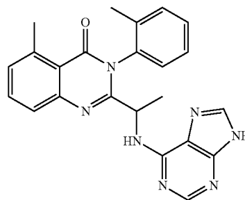
5-Methyl-2-[1-(9H-purin-6-ylamino)ethyl]-3-o-tolyl-3H-quinazolin-4-one (D-081)
