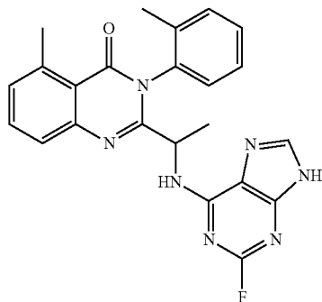
2-[1-(2-Fluoro-9H-purin-6-ylamino)ethyl]-5-methyl-3-o-tolyl-3H-quinazolin-4-one (D-080)
