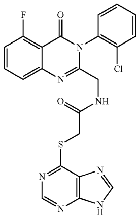
N-[3-(2-Chlorophenyl)-5-fluoro-4-oxo-3,4-dihydroquinazolin-2-ylmethyl]-2-(9H-purin-6-ylsulfanyl)acetamide (D-077)
