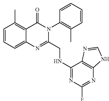
2-[(2-Fluoro-9H-purin-6-ylamino)methyl]-5-methyl-3-o-tolyl-3H-quinazolin-4-one (D-076)
