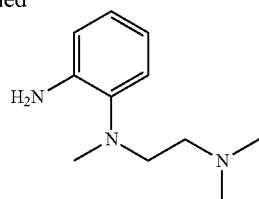
Intermediate E-3
