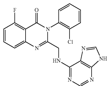
3-(2-Chlorophenyl)-5-fluoro-2-[(9H-purin-6-ylamino)methyl]-3H-quinazolin-4-one (D-072)
