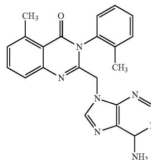
D-030
