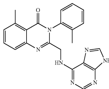
5-Methyl-2-[(9H-purin-6-ylamino)methyl]-3-o-tolyl-3H-quinazolin-4-one (D-071)
