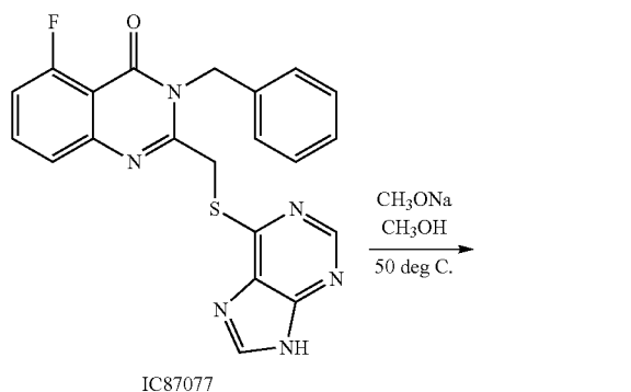
Scheme H
