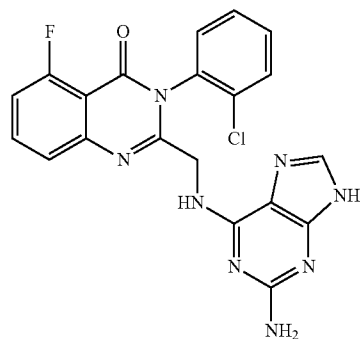
2-[(2-Amino-9H-purin-6-ylamino)methyl]-3-(2-chlorophenyl)-5-fluoro-3H-quinazolin-4-one (D-074)
