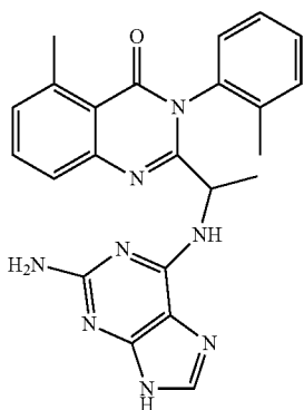
2-(1-(2-Amino-9H-purin-6-ylamino)ethyl)-5-methyl-3-o-tolyl-3H-quinazolin-4-one (D-081a)
