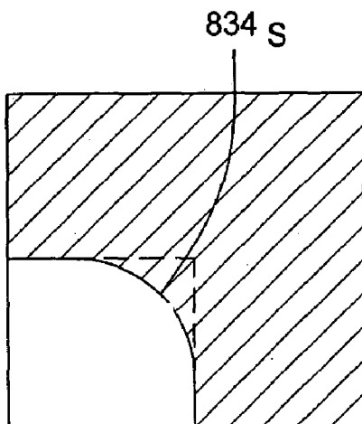
UNCORRECTED CONCAVE CORNER
