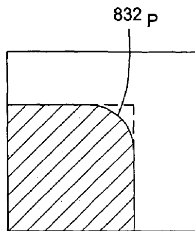
CORRECTED CONVEX CORNER
