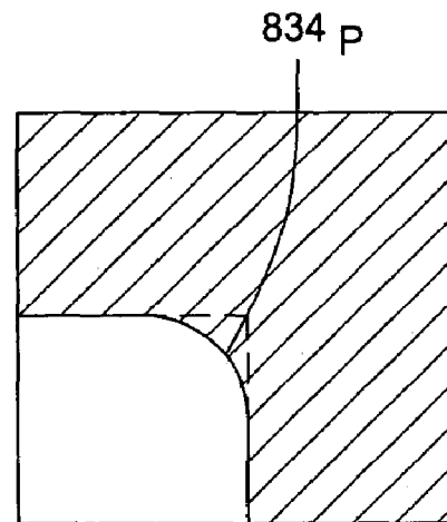
CORRECTED CONCAVE CORNER
