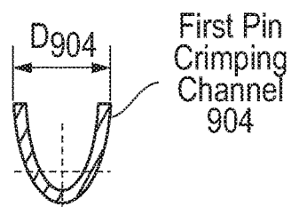
SECT 9C-9C
