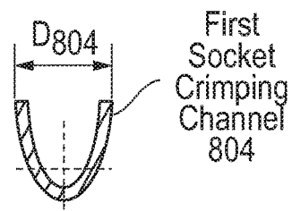
SECT 8C-8C
