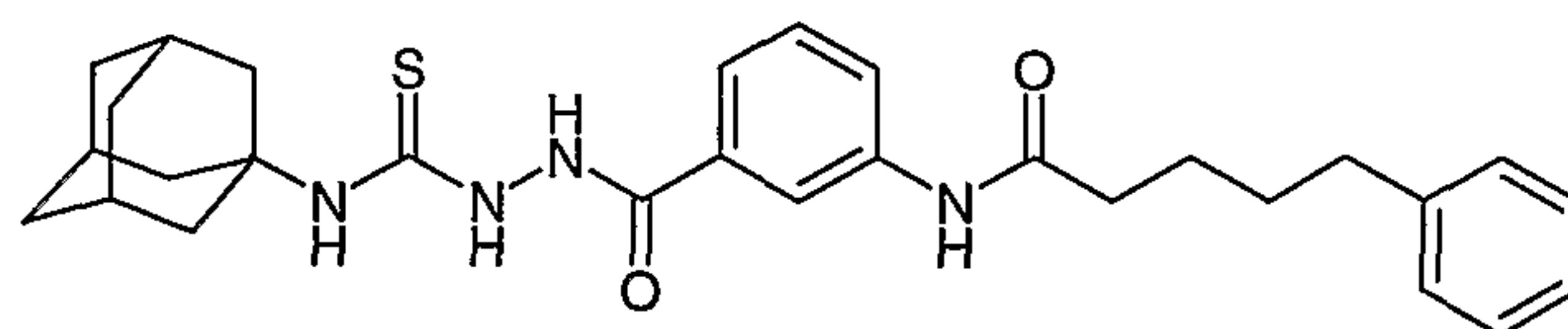
Compound # 41
