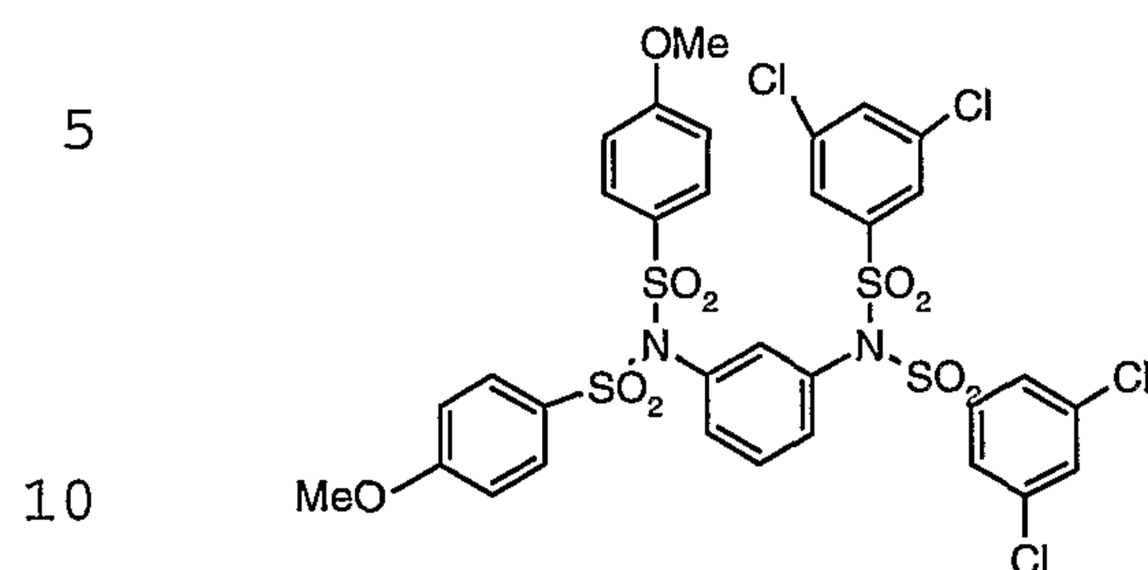
Compound # 10
