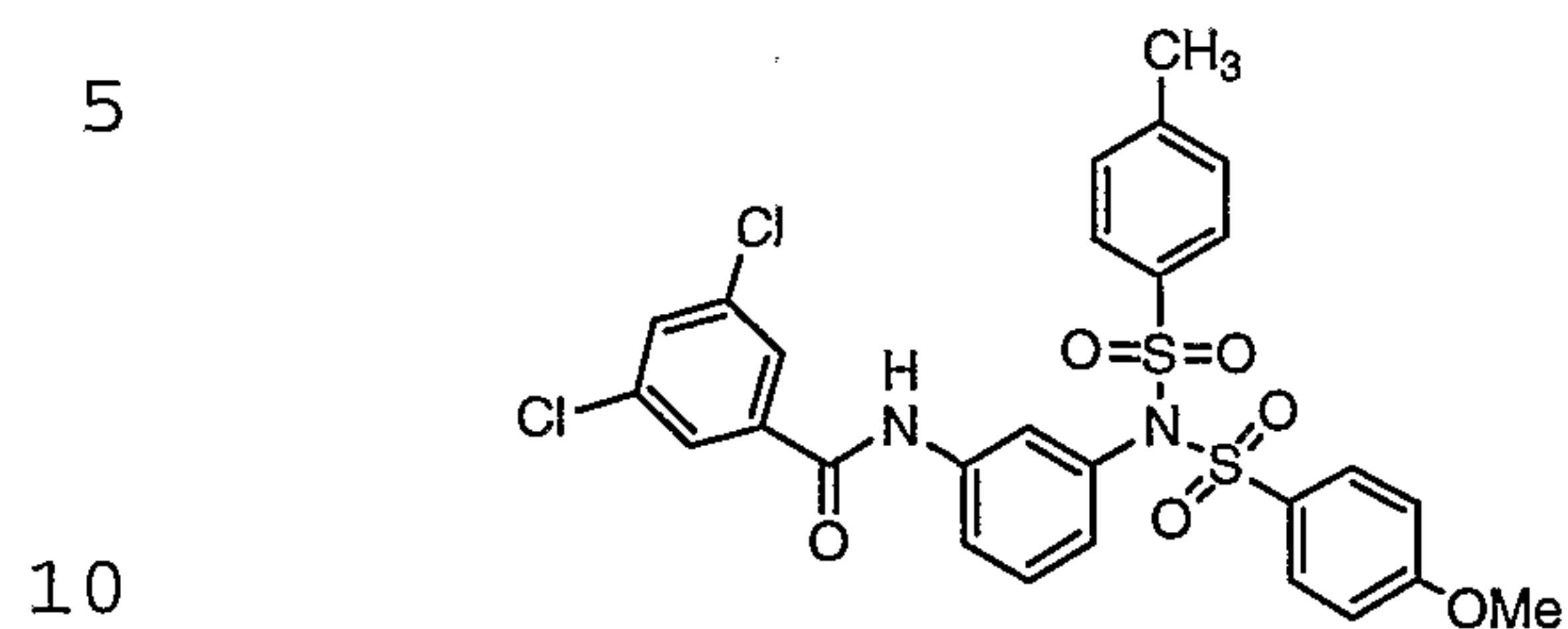
Compound # 3
