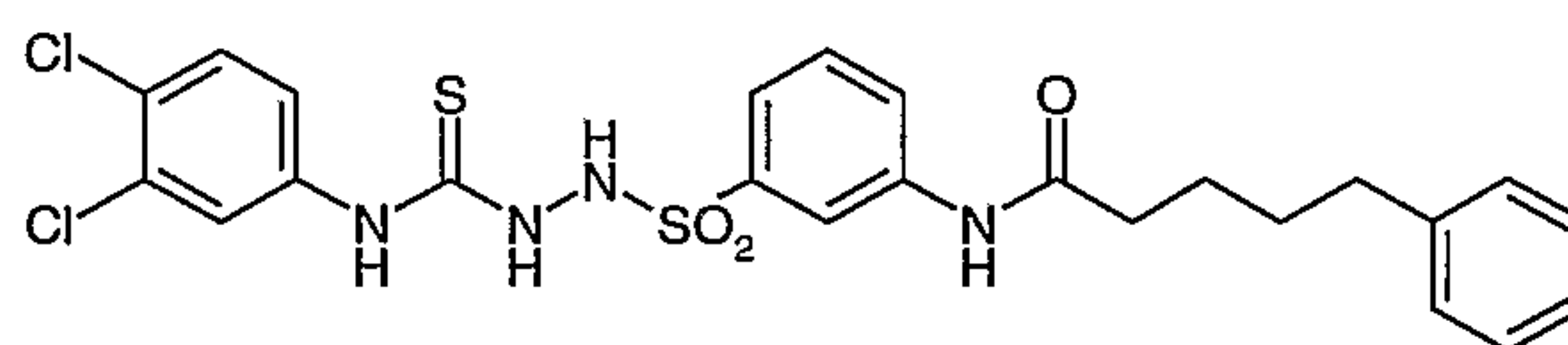
Compound # 35
