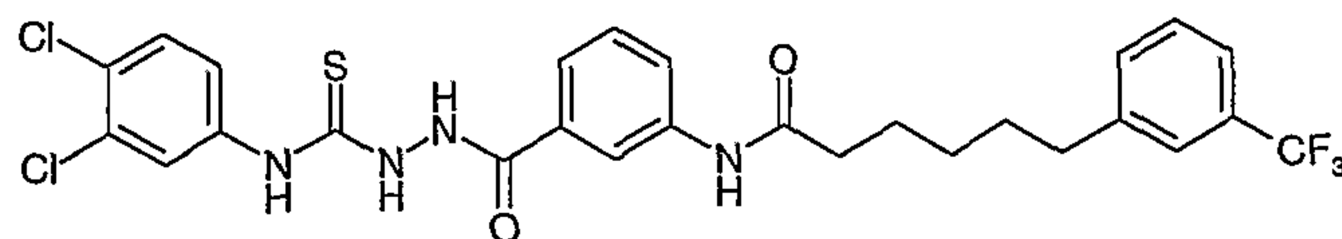
Compound # 32
