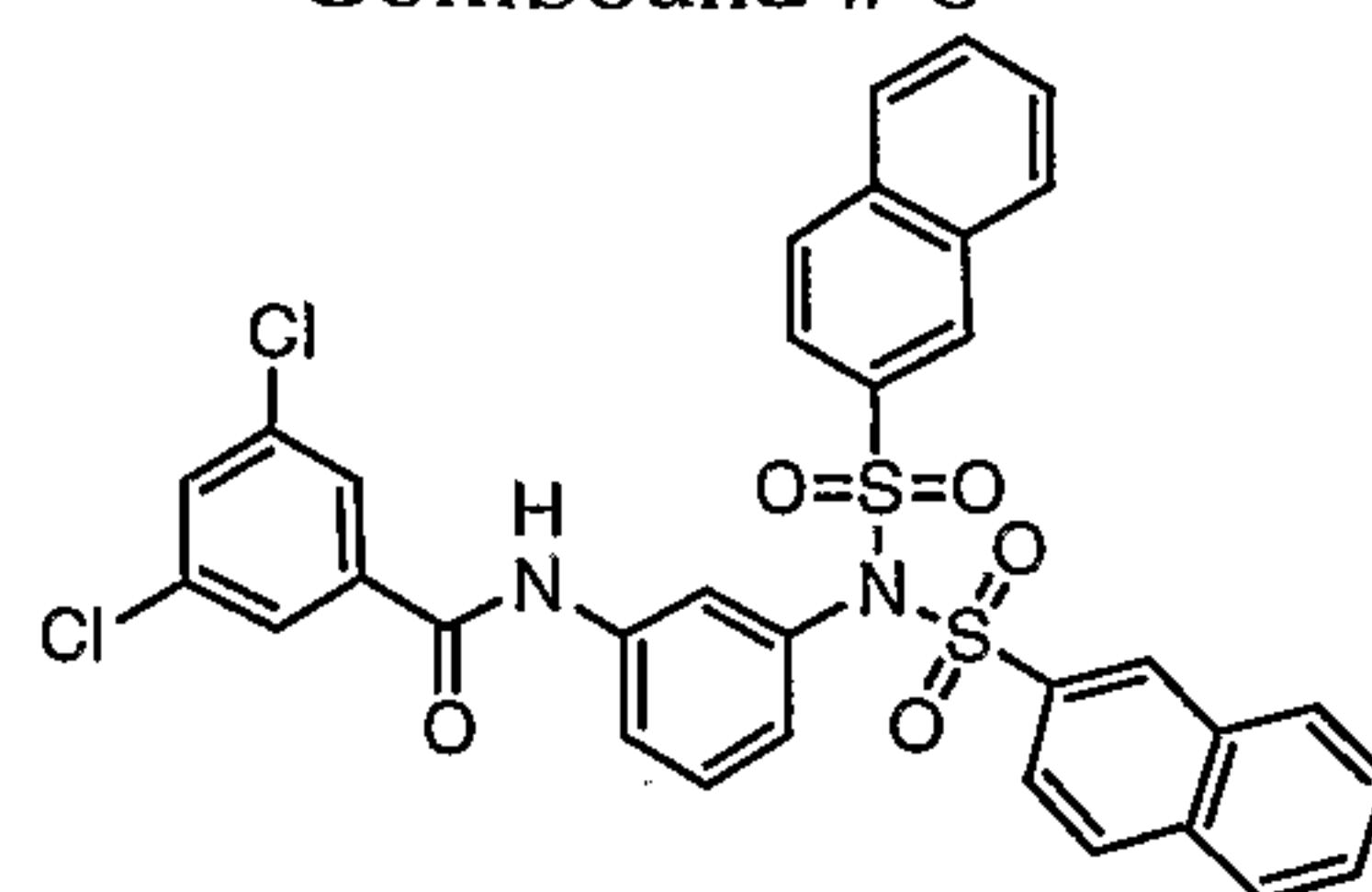
Compound # 8
