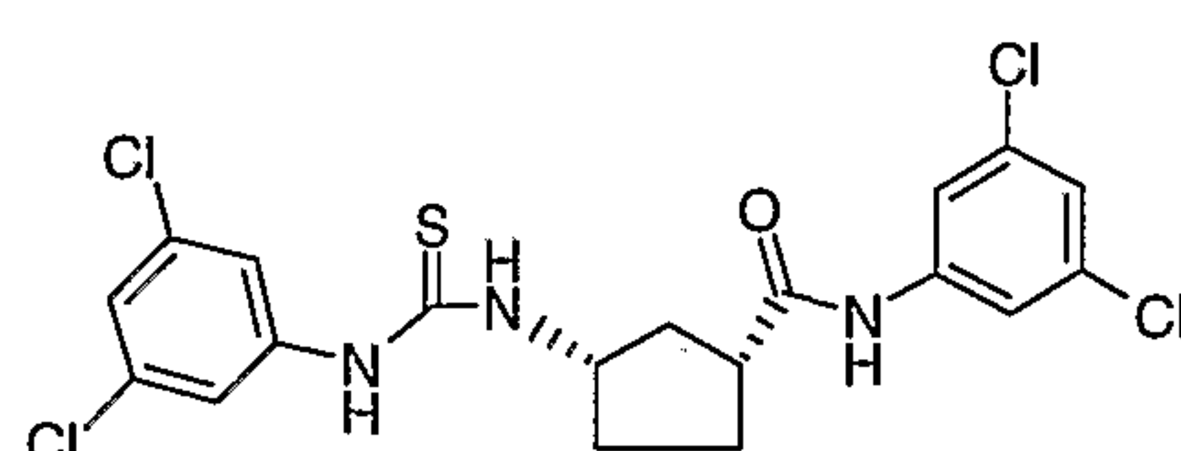
Compound # 19
