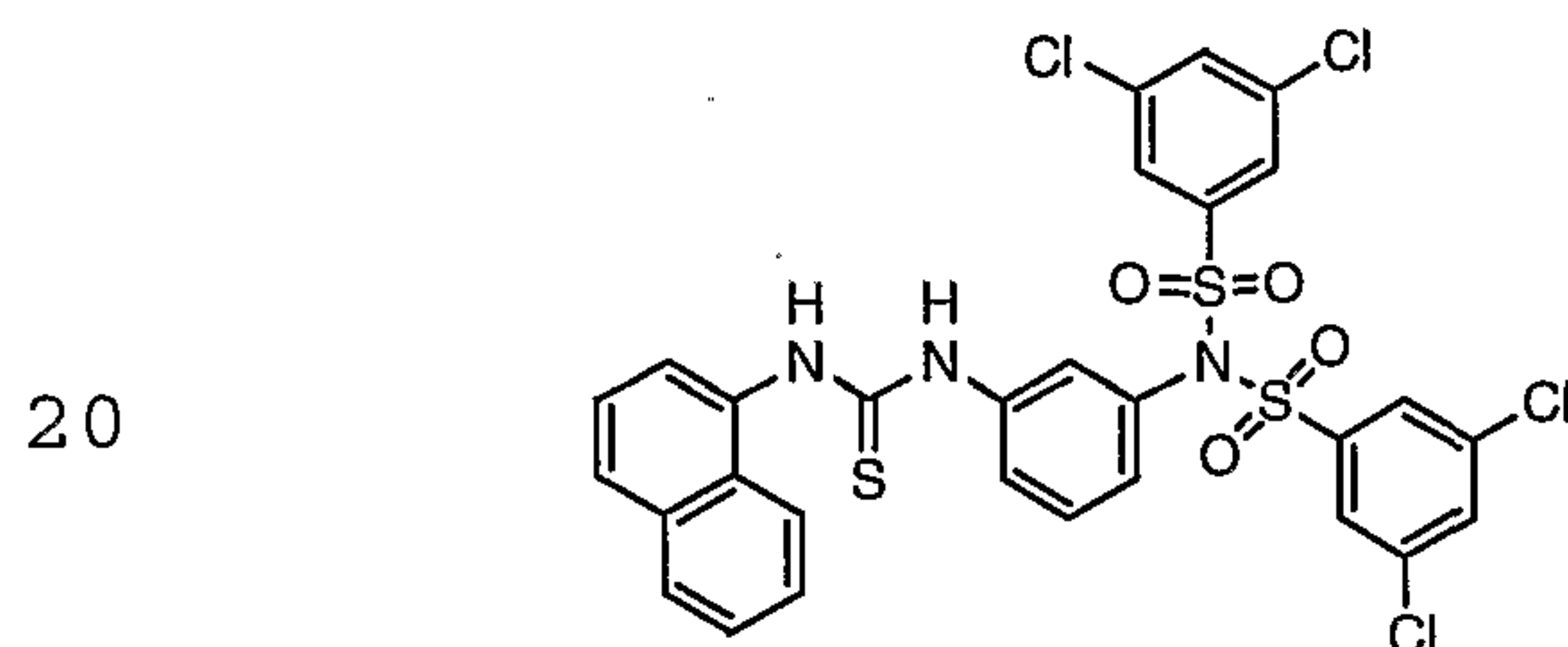
Compound # 5
