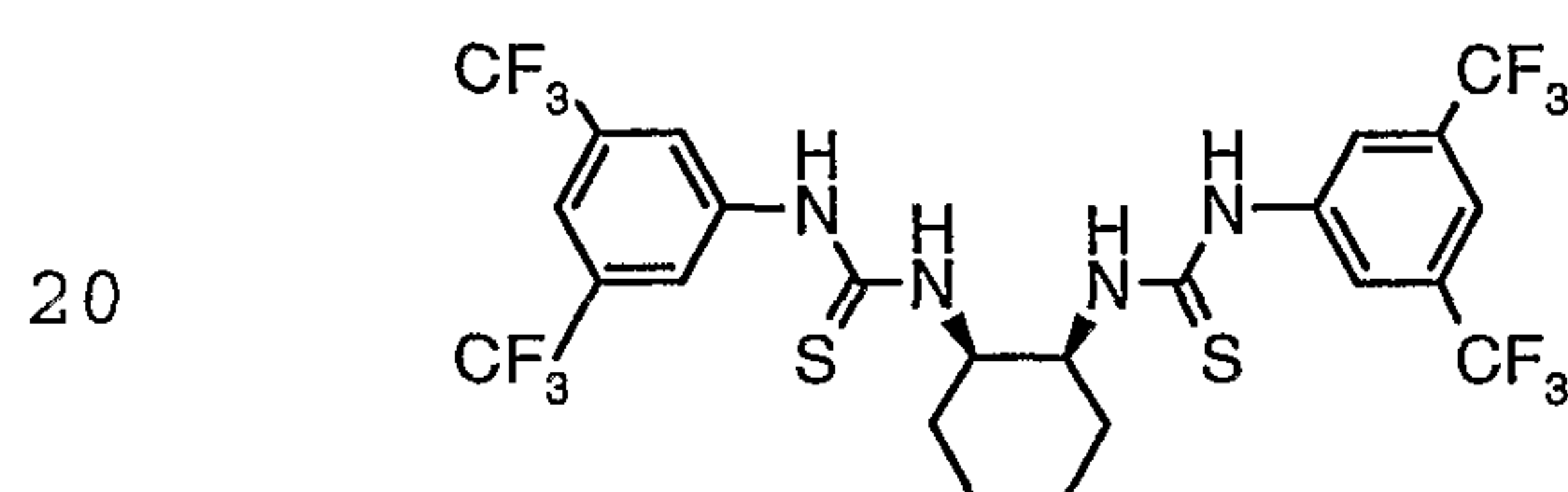
Compound # 12
