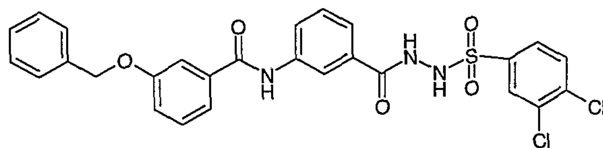
Compound # 31
