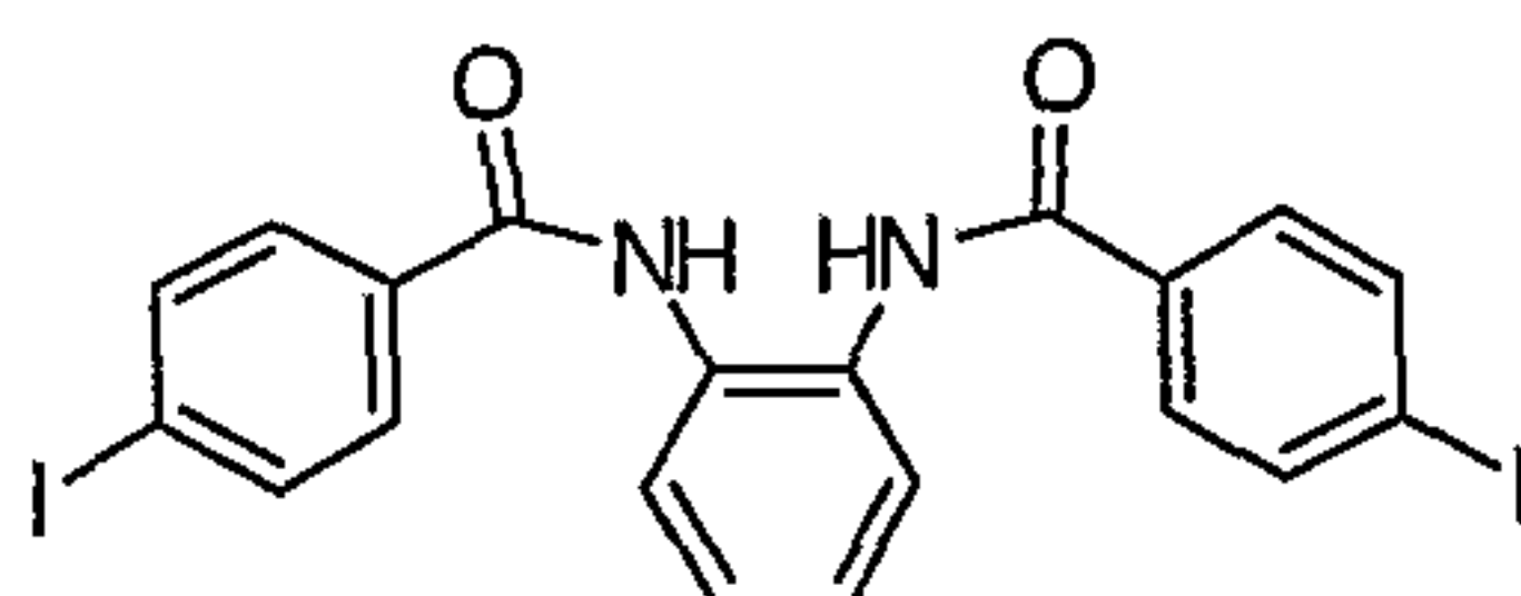
Compound # 29
