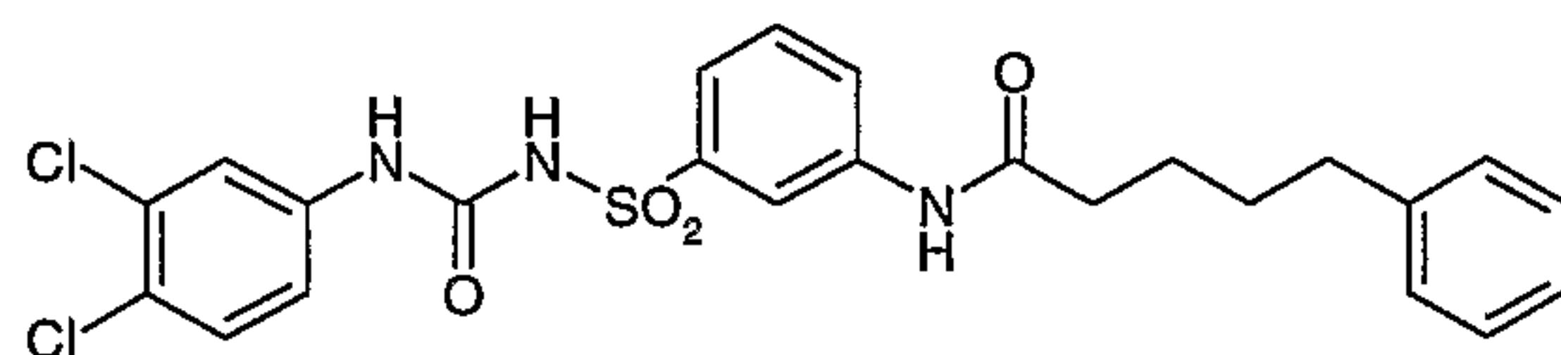
Compound # 34B
