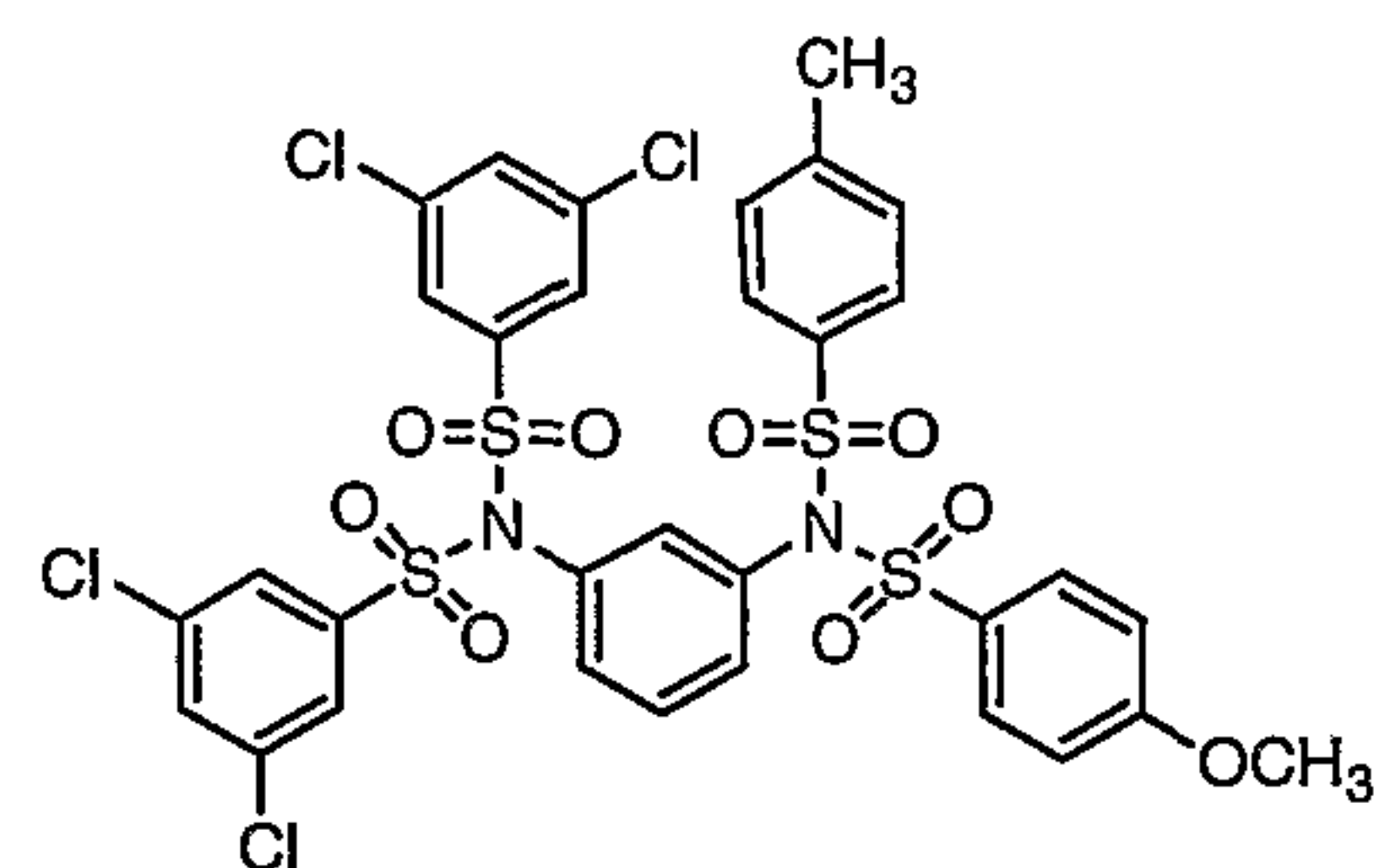
Compound # 4
