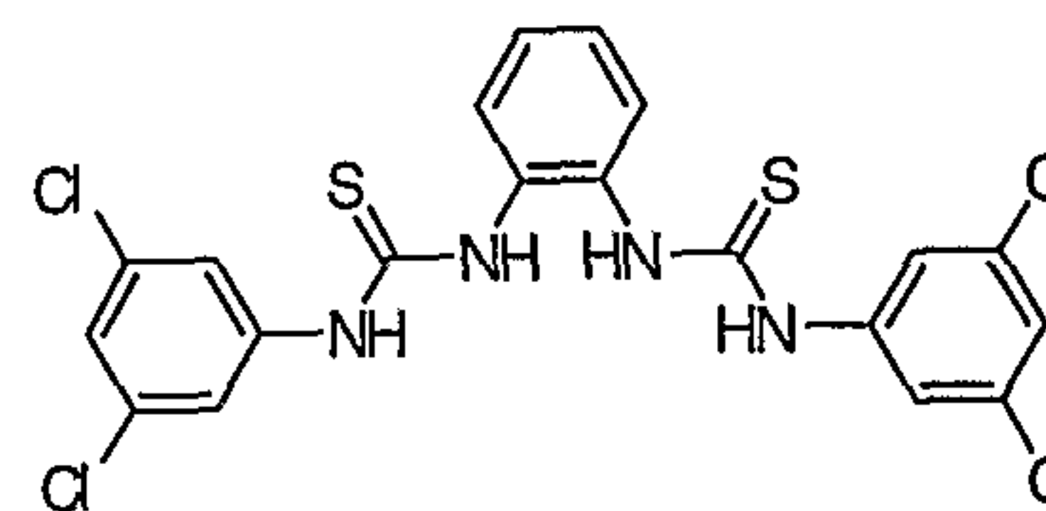
Compound # 28
