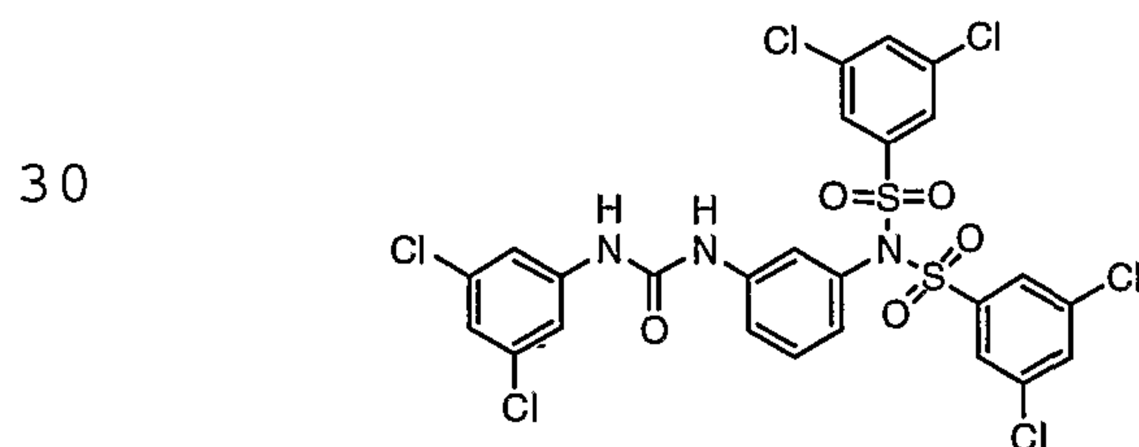
Compound # 7
