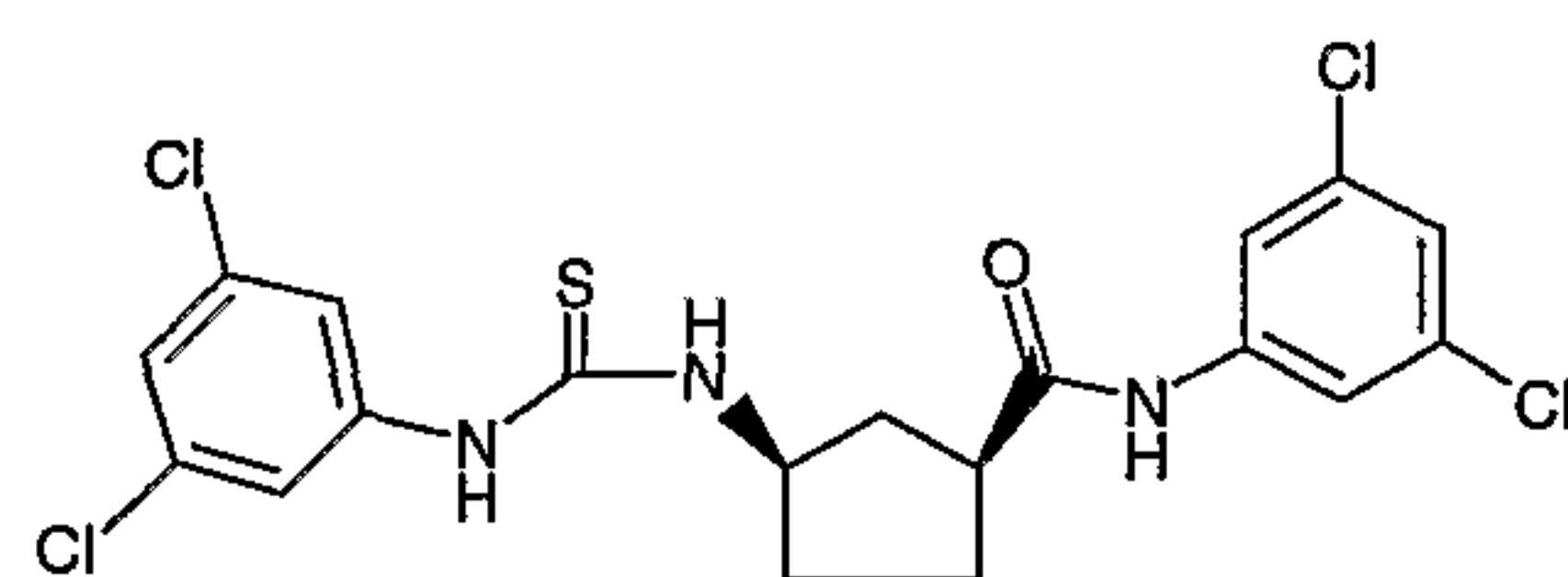
Compound # 17
