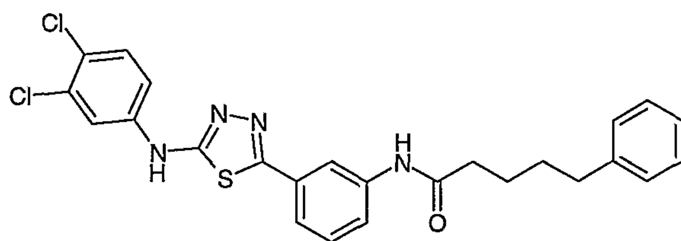
Compound # 40A
