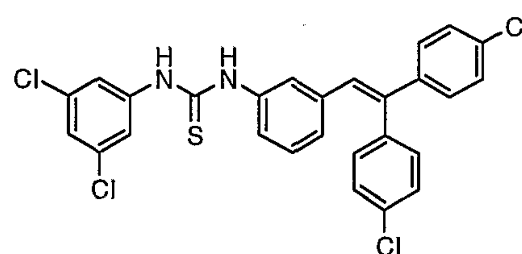
Compound # 20
