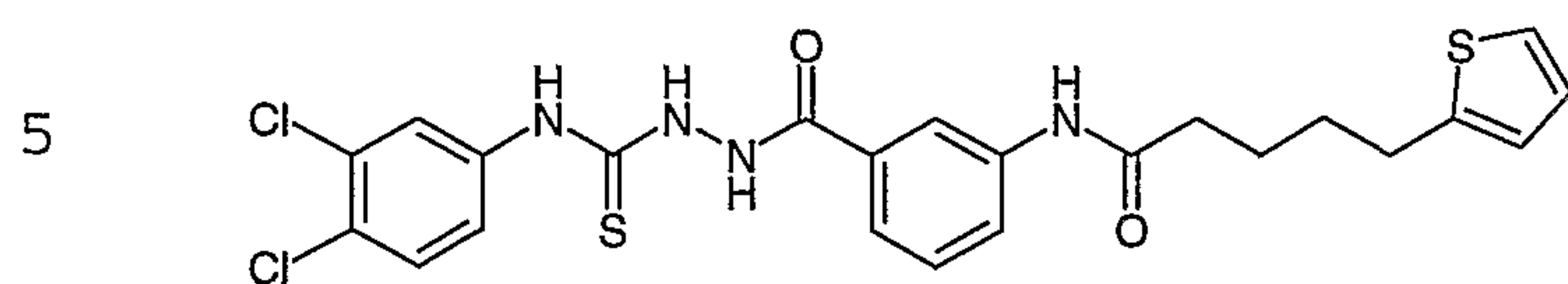
Compound # 38
