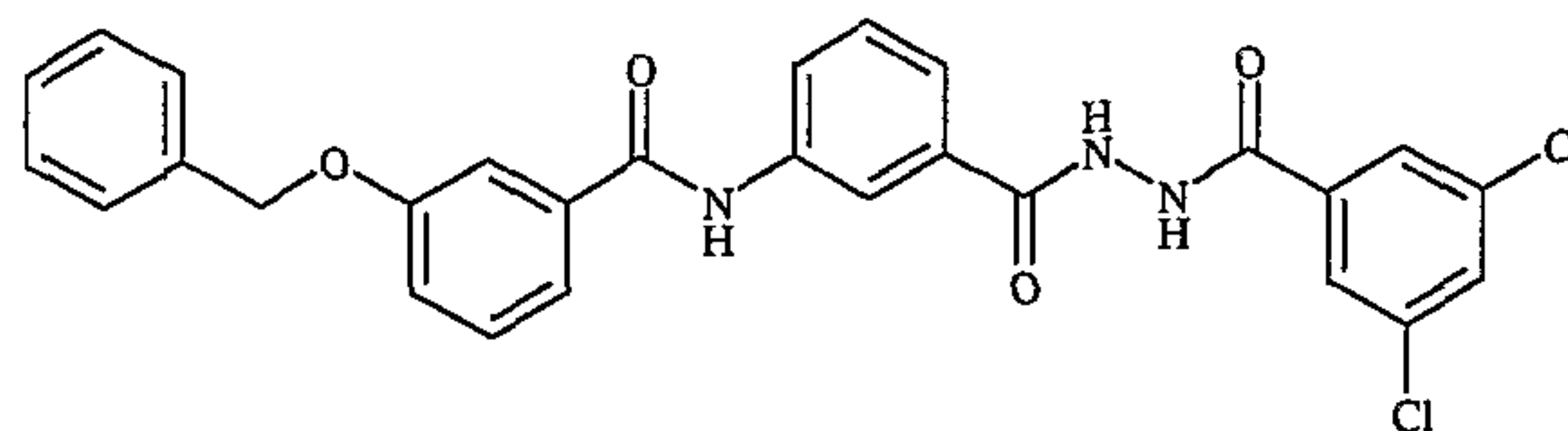
Compound # 30
