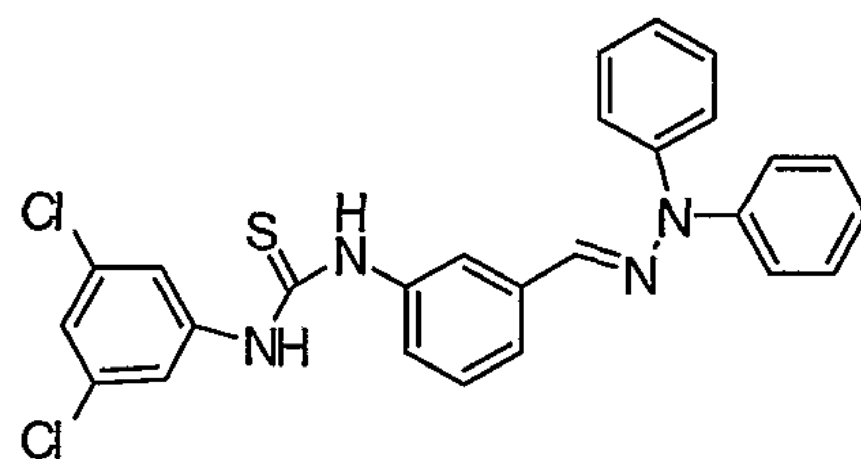
Compound # 21
