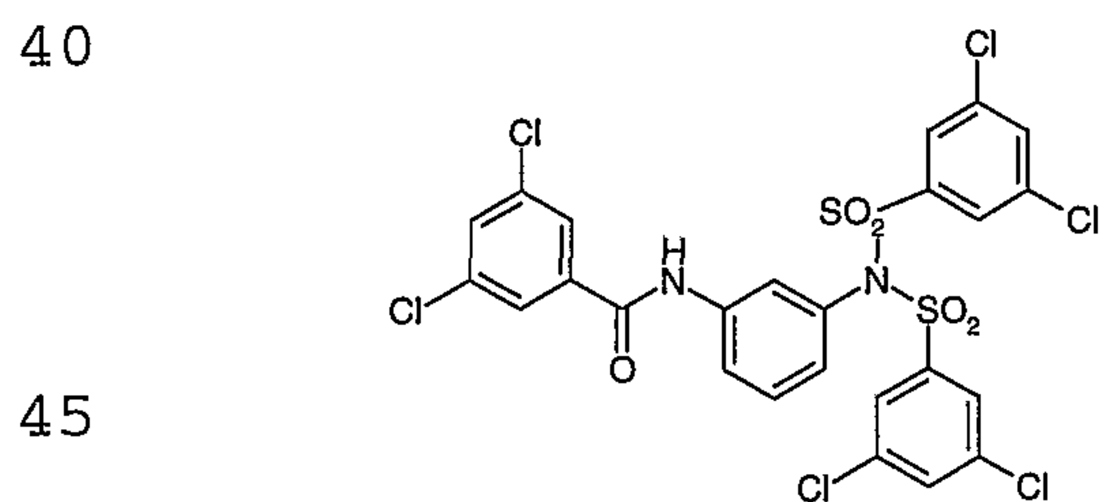
Compound # 8a
