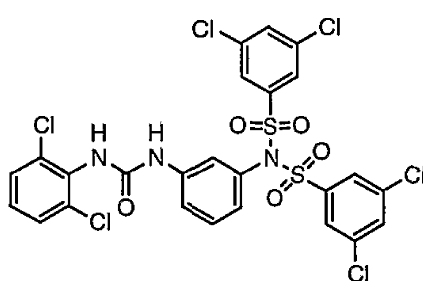
Compound # 6
