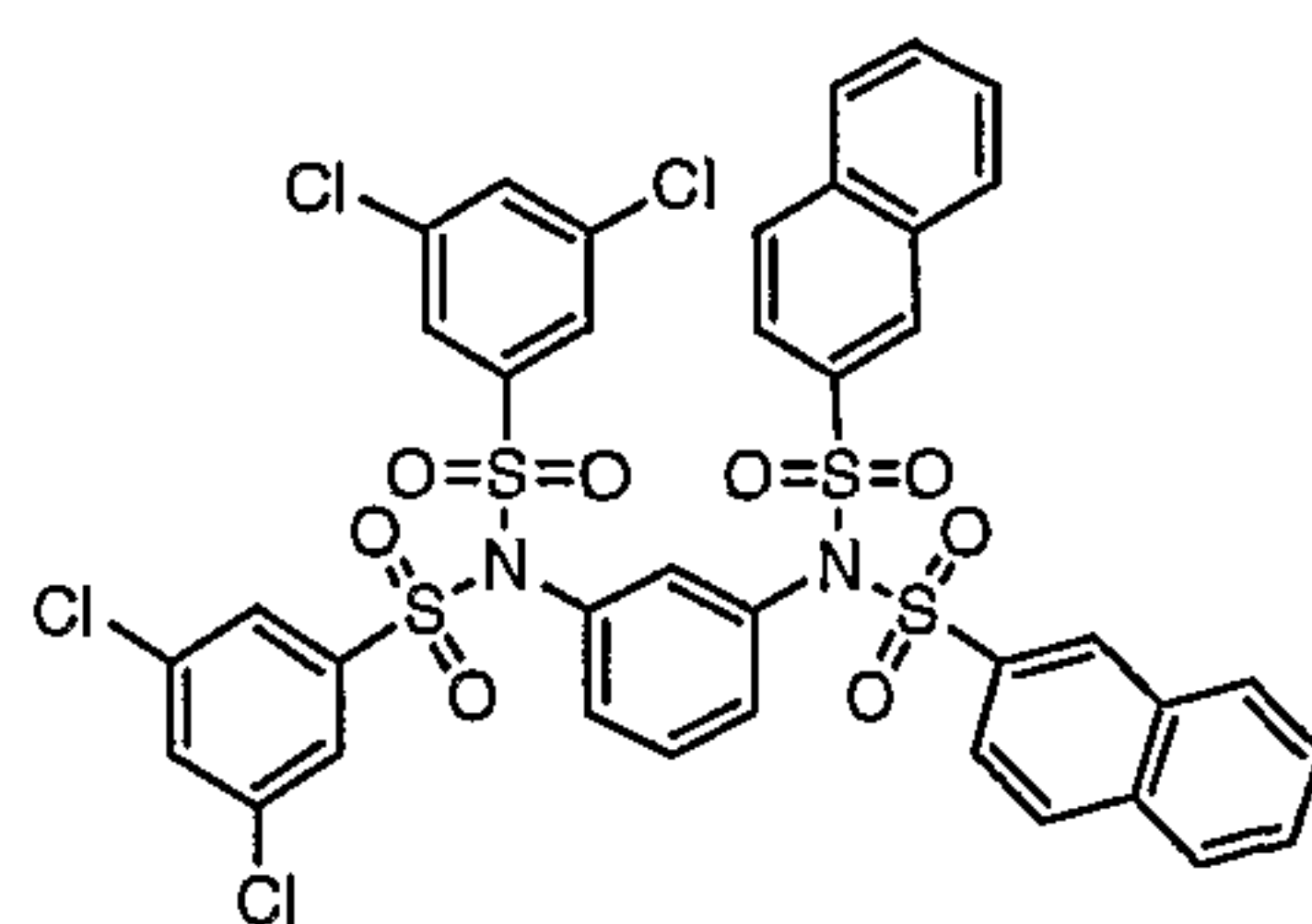
Compound # 9
