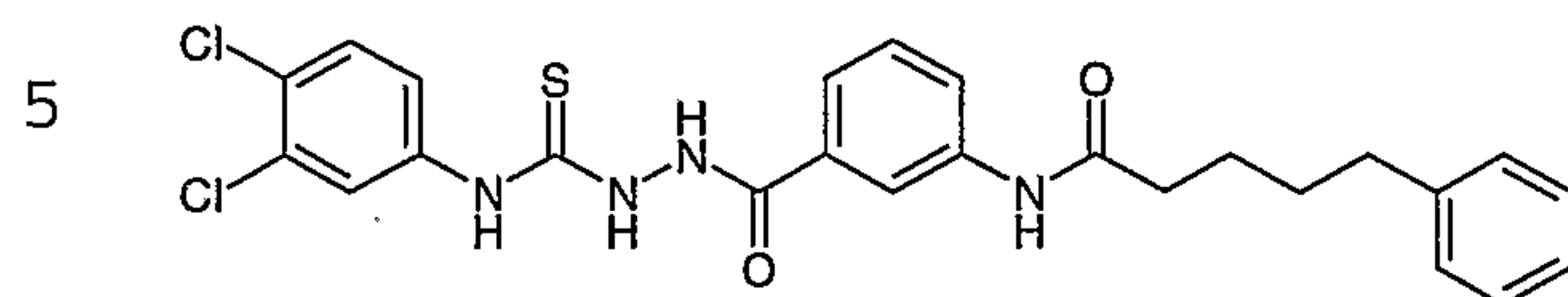
Compound # 33
