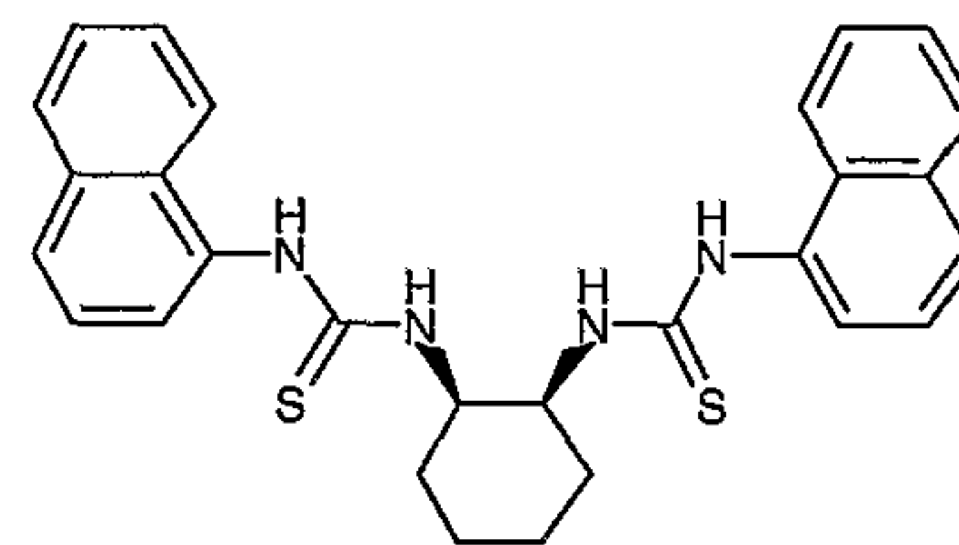
Compound # 11
