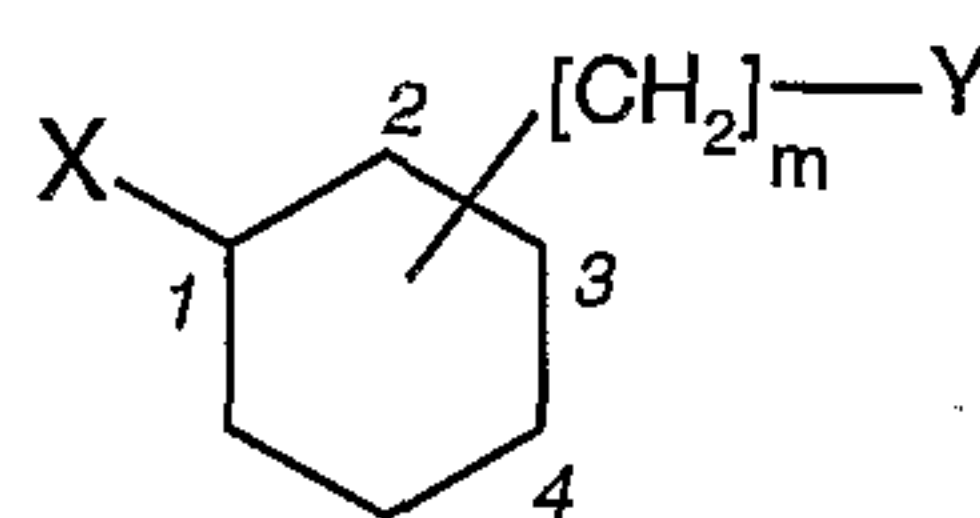
Formula IV
