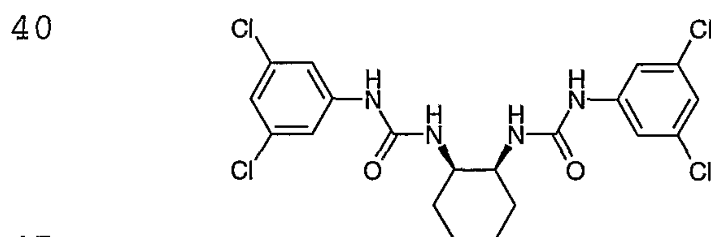
Compound # 15a
