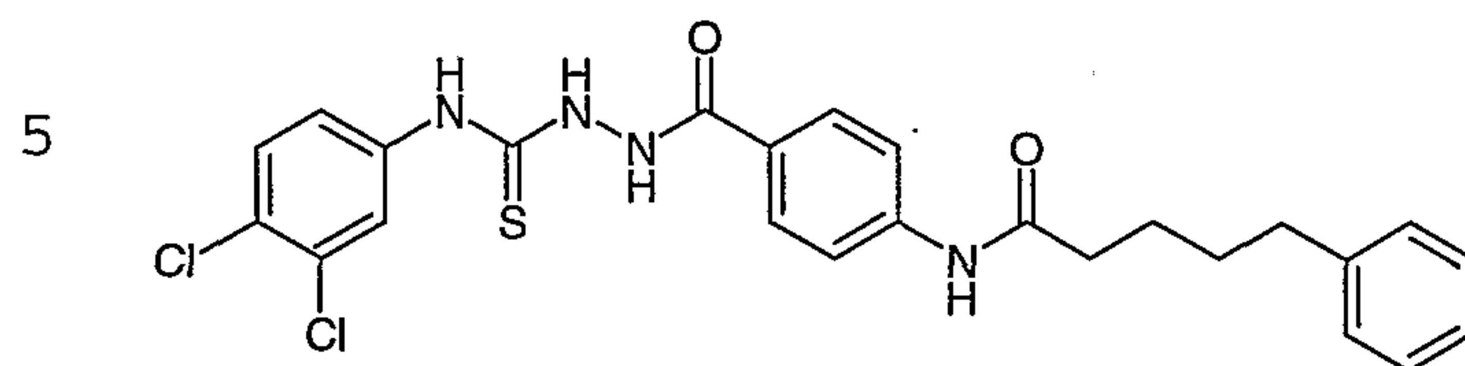
Compound # 43
