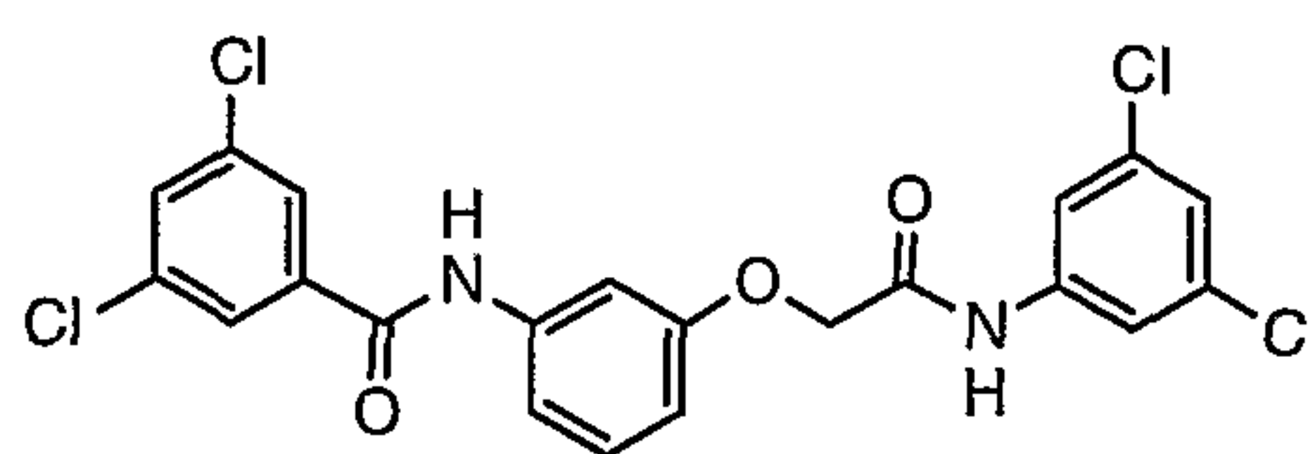
Compound # 24
