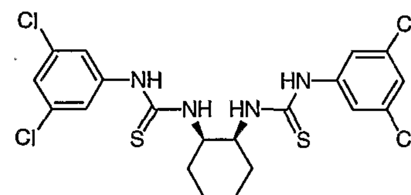
Compound # 15
