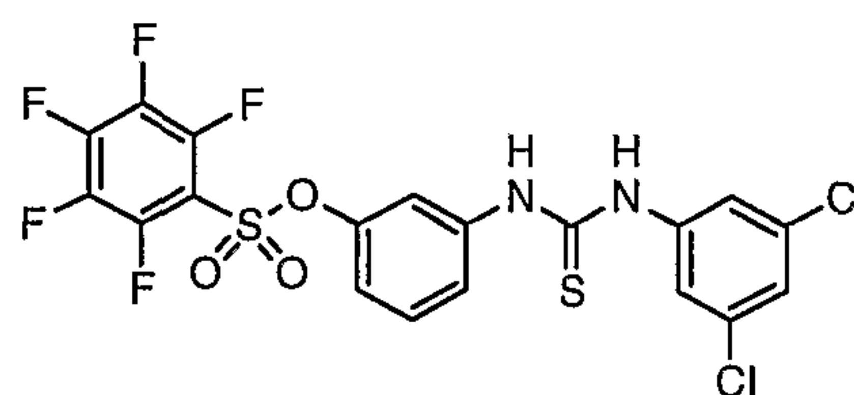
Compound # 22
