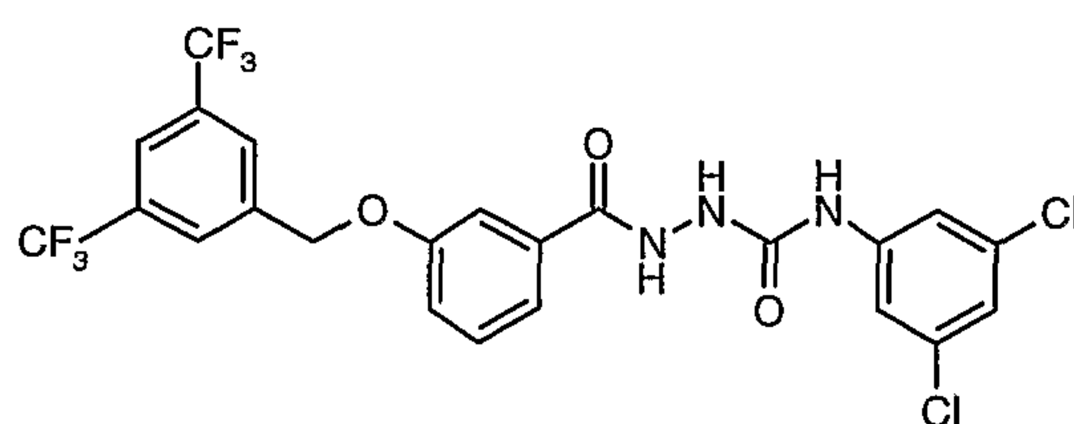
Compound # 23
