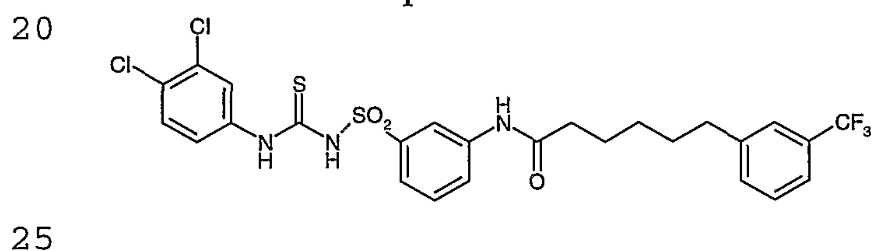
Compound # 45
