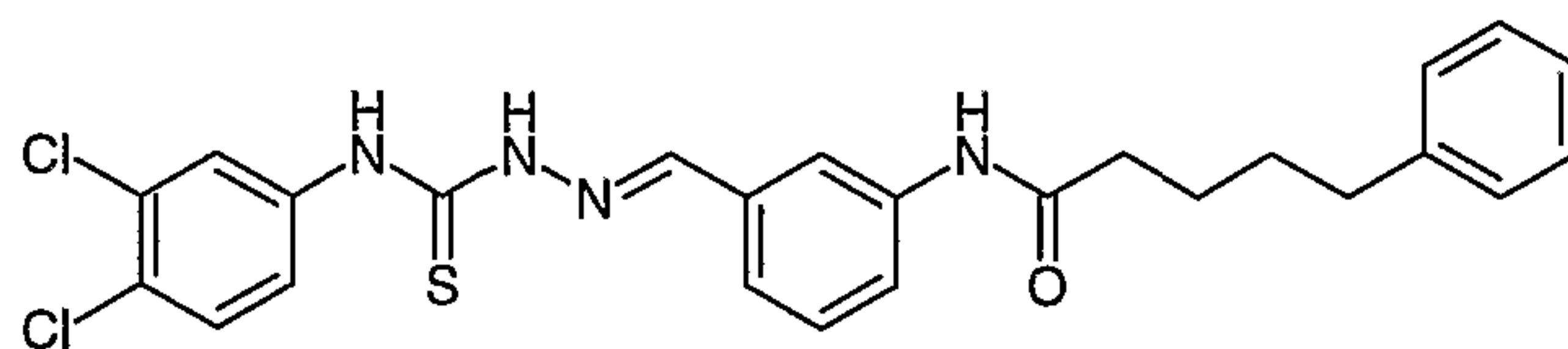
Compound # 39
