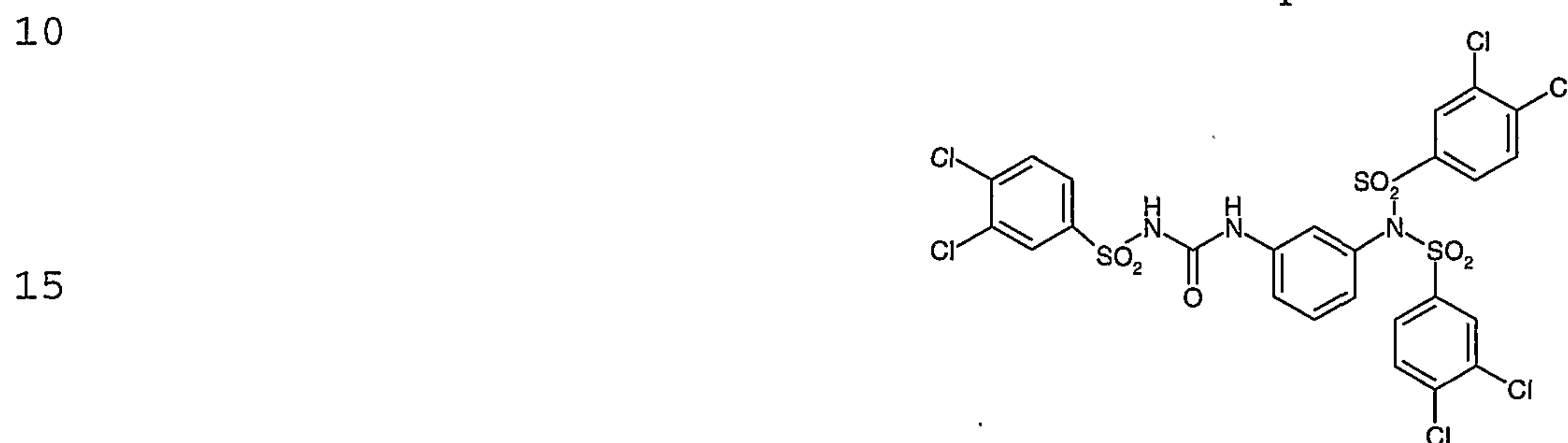
Compound # 45
