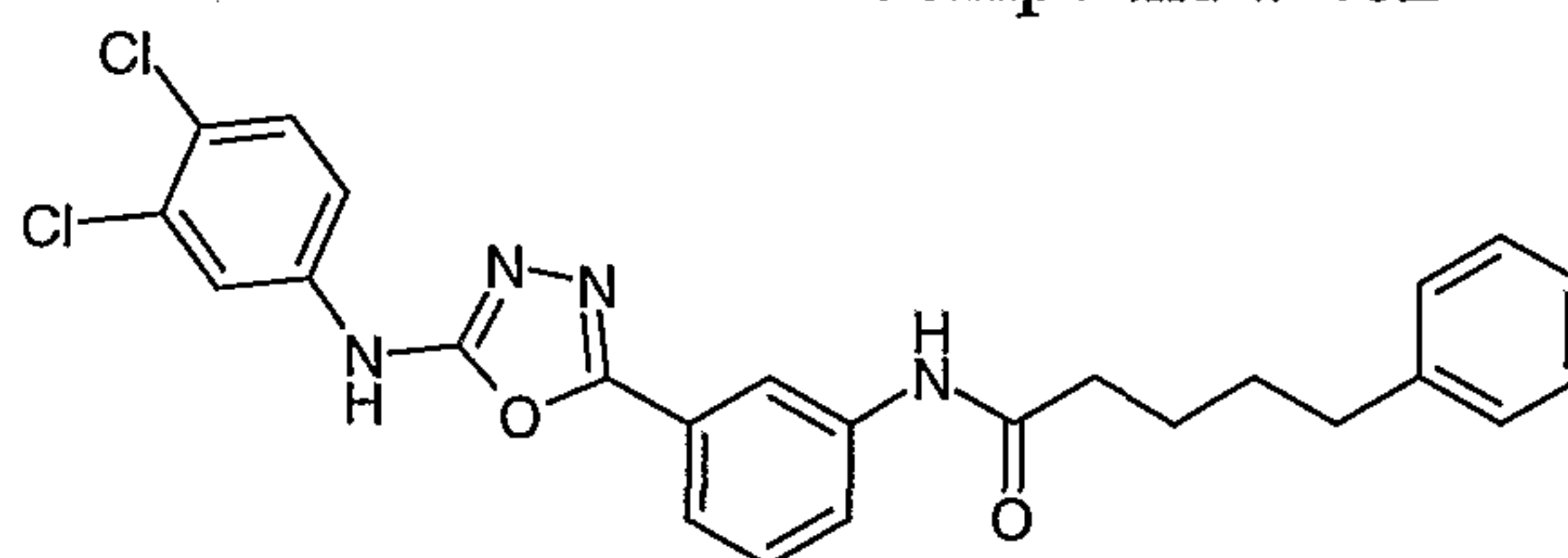
Compound # 40B
