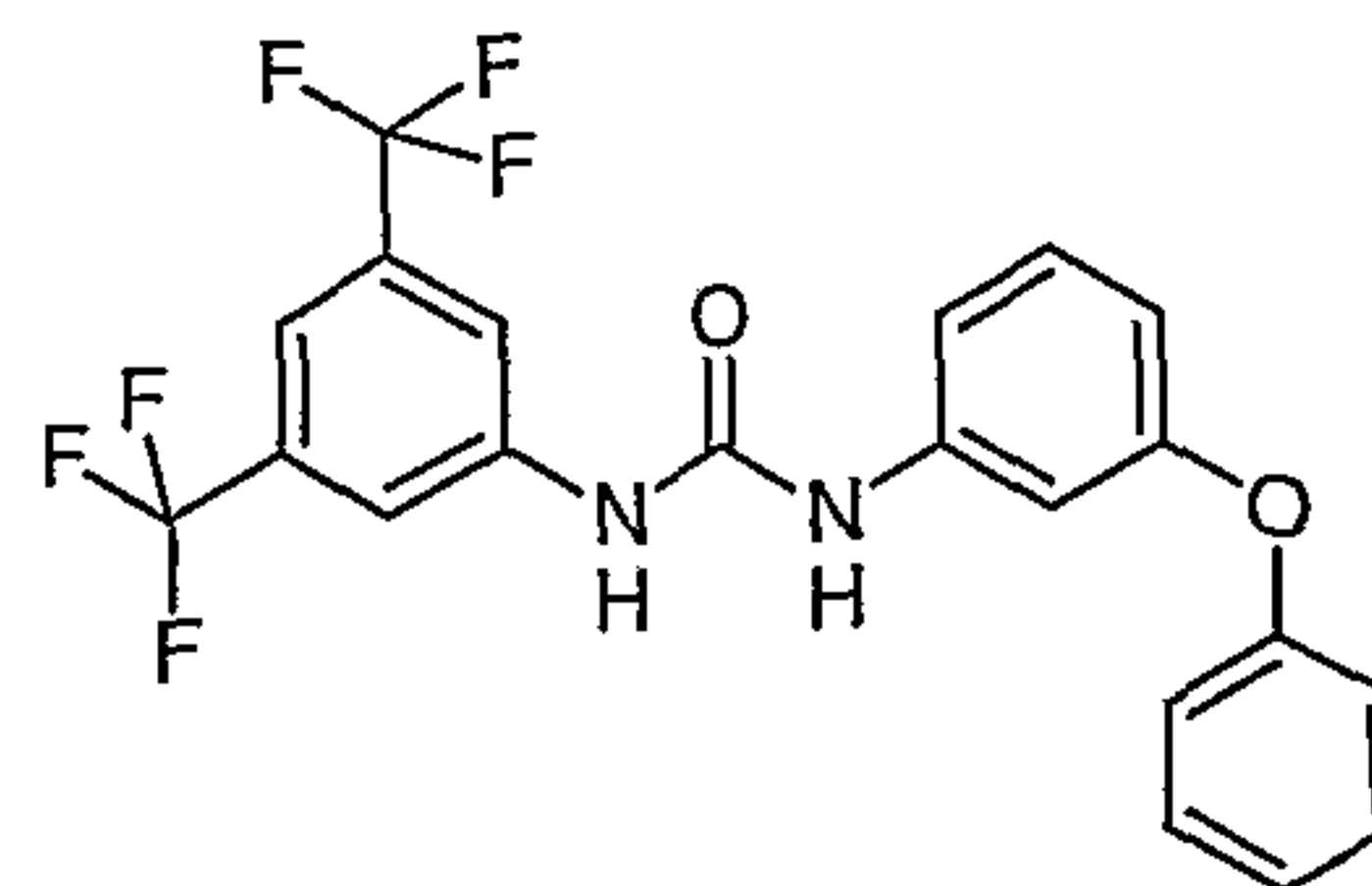
Compound # 26
