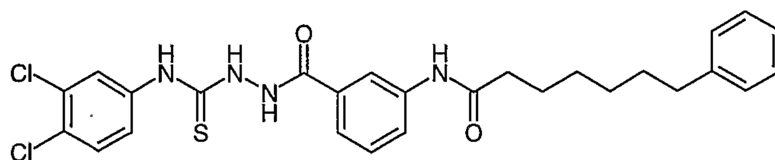
Compound # 37
