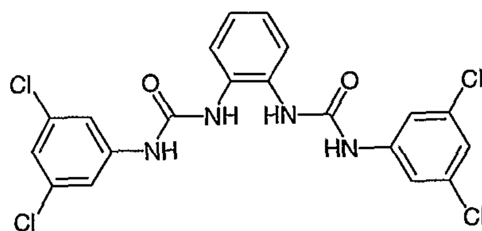
Compound # 27
