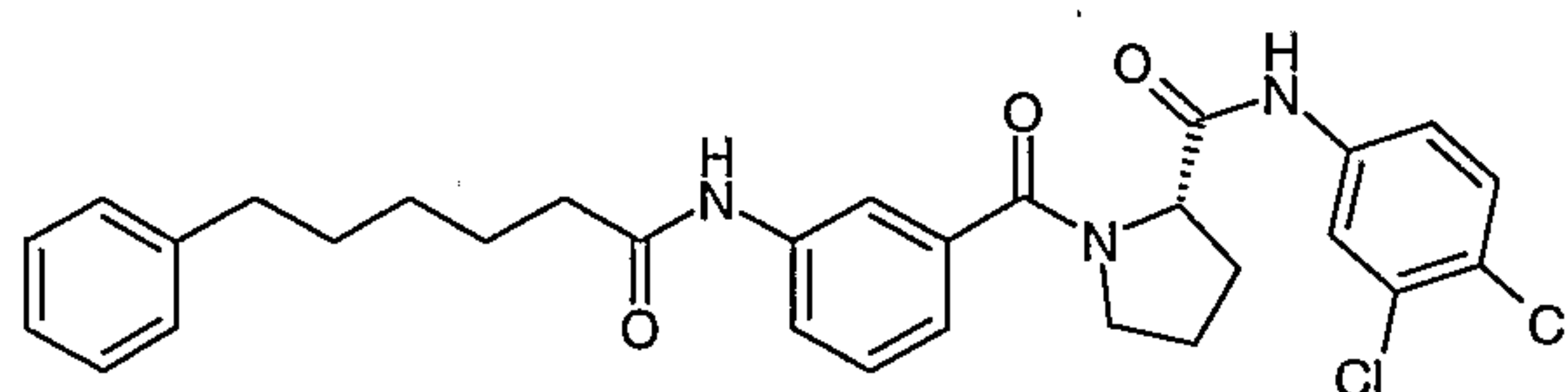
Compound # 36
