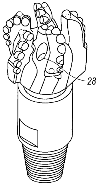
FIG. 1C (PRIOR ART)
