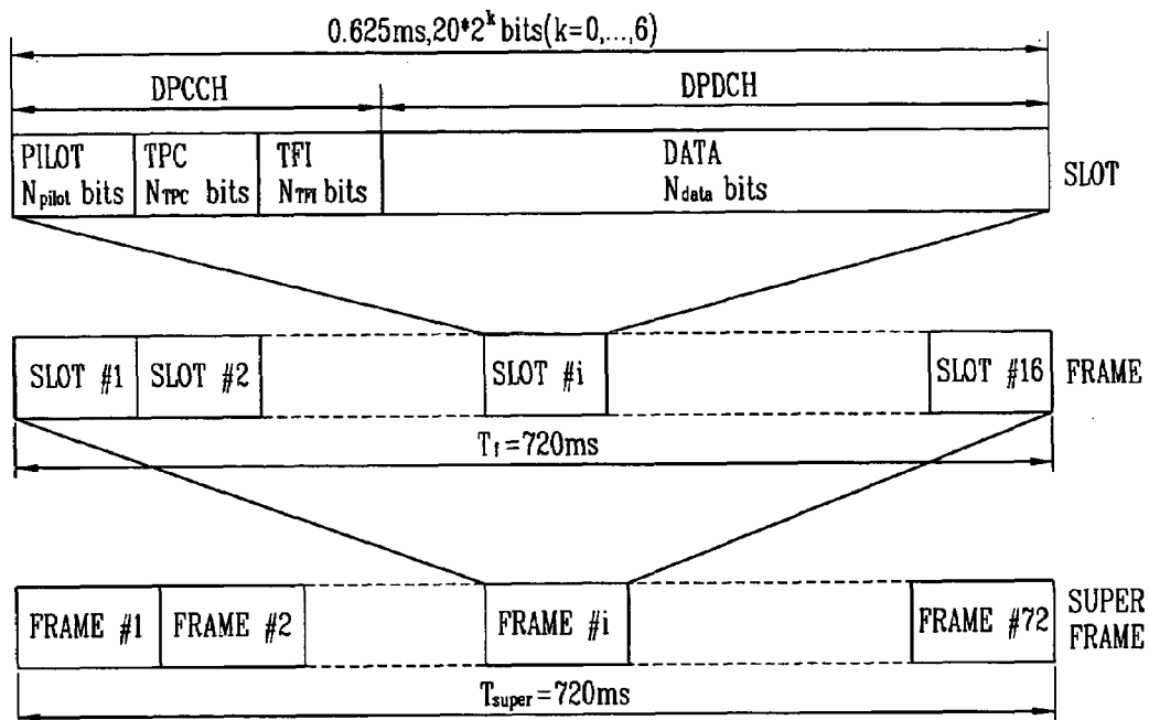
FIG. 2 RELATED ART
