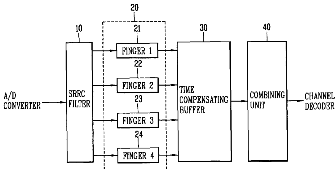
FIG. 3 RELATED ART
