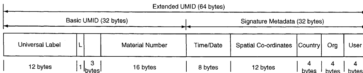
Basic and Extended UMID Structures
