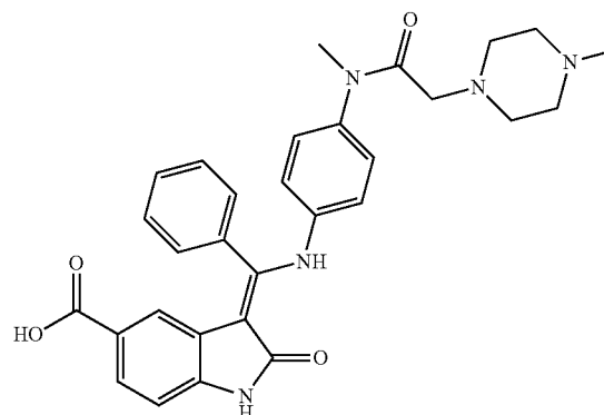
Compound 21
