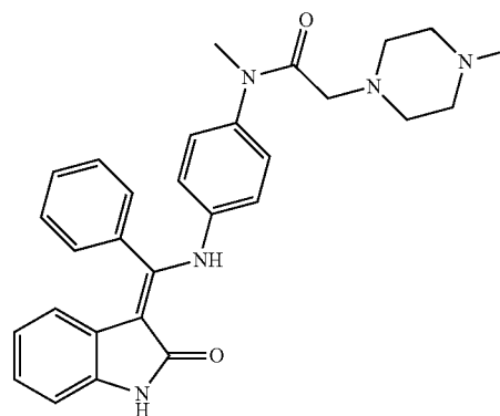
Compound 17
