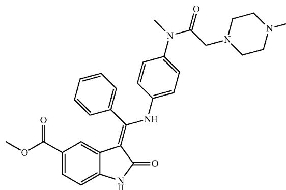
Compound 21
