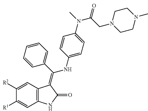
Formula II
