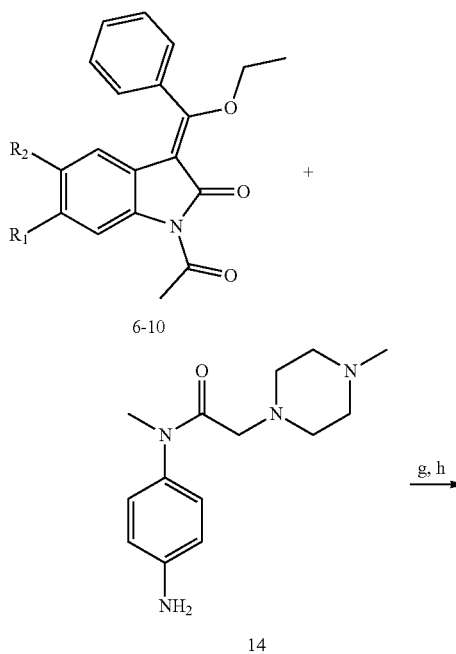
Scheme 2
