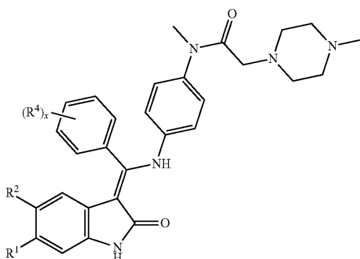
Formula III
