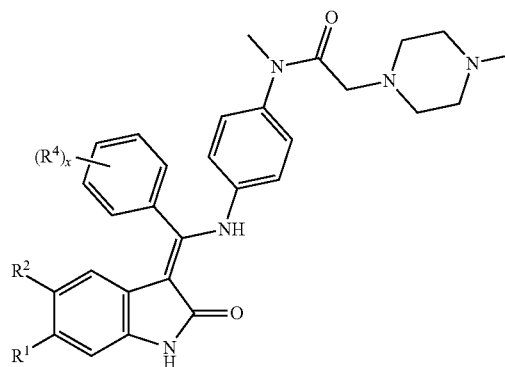
Formula III
