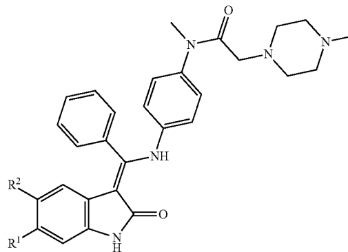
Formula II
