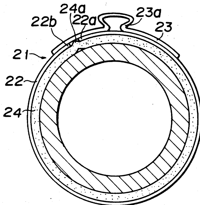
FIG. 11 PRIOR ART
