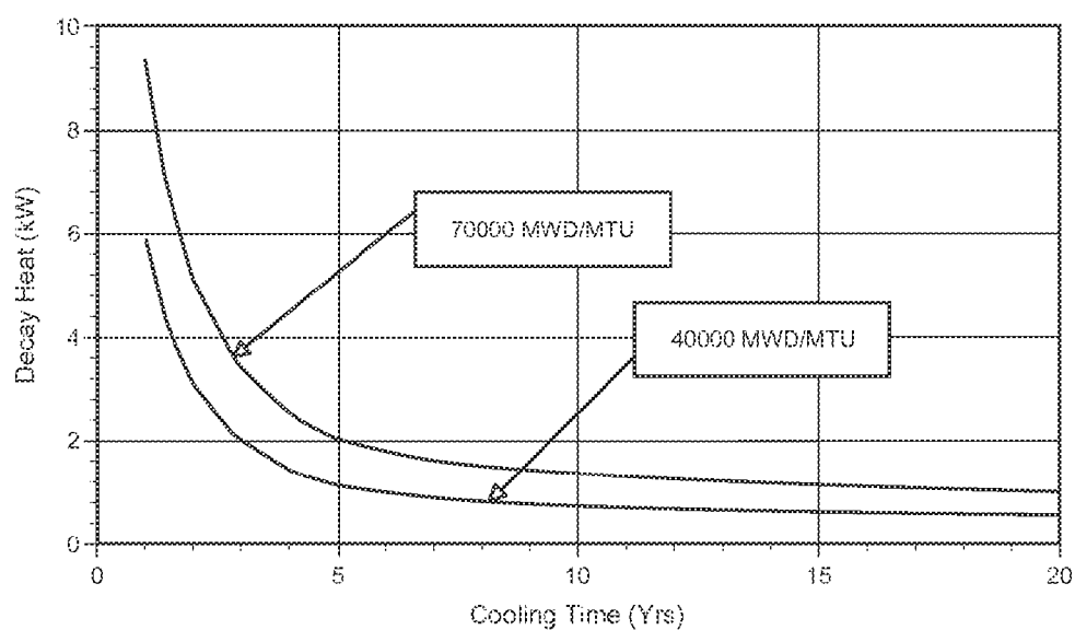
B&W 15x15 Fuel Assembly Decay Heat Curves
