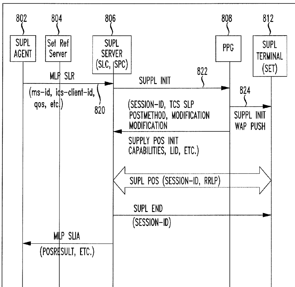
TYPICAL OMA SUPL CALL FLOW
