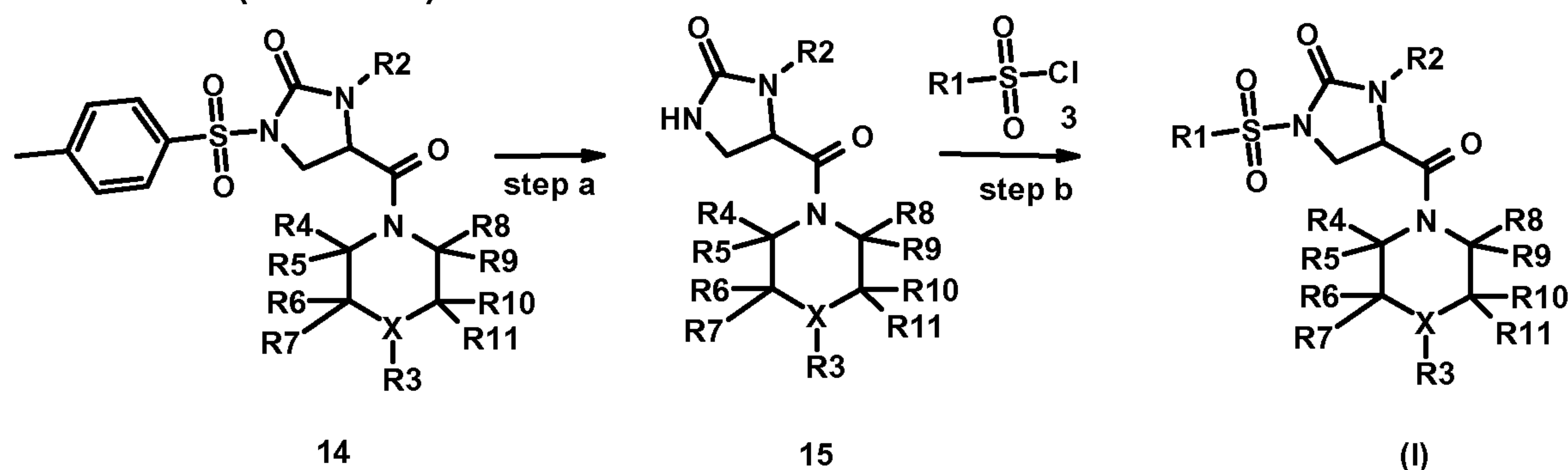
Scheme 3: (Method C)
