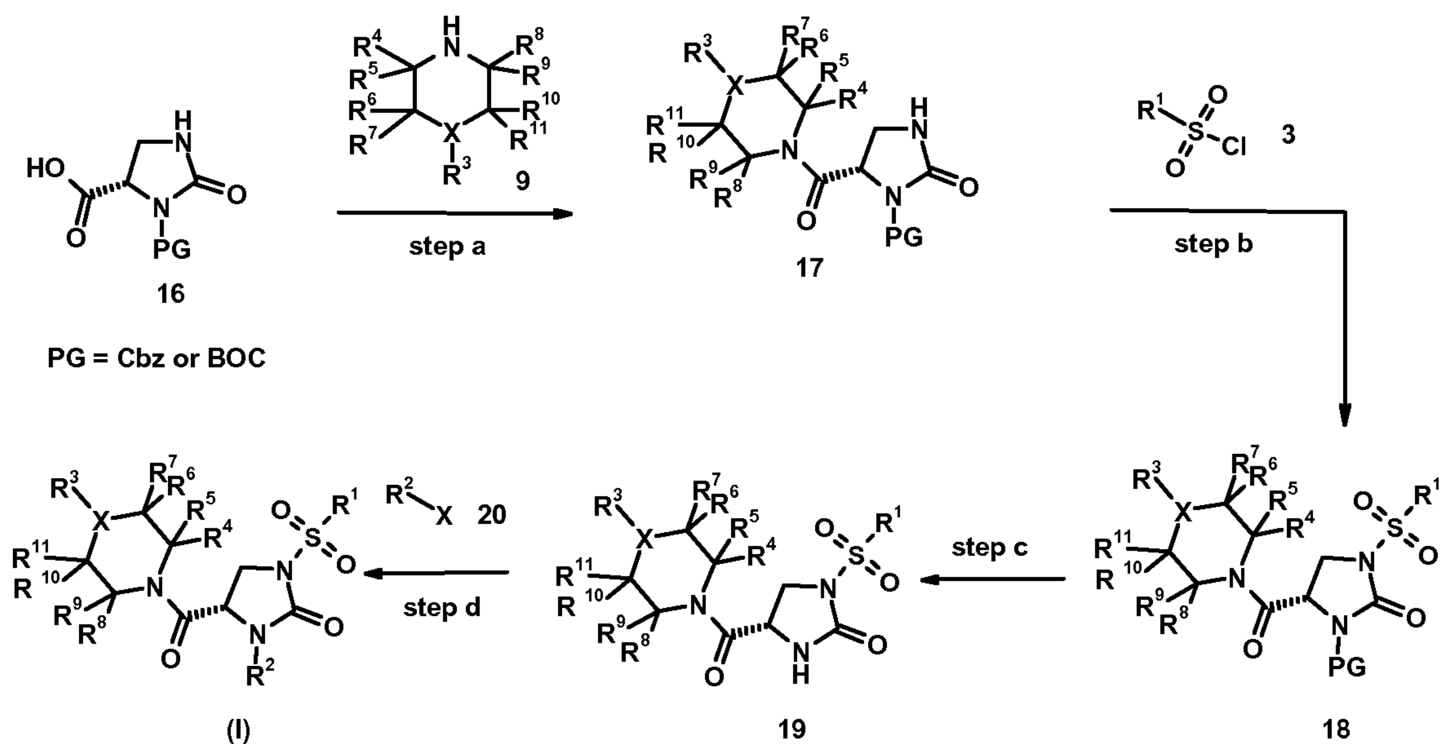
Scheme 4 (Method D)
