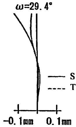
Astigmatism Fig. 6(B)
