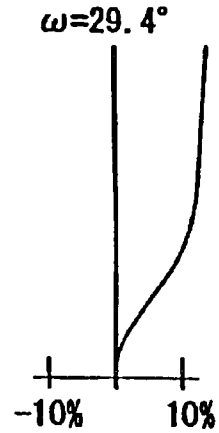
Distortion Fig. 6(C)
