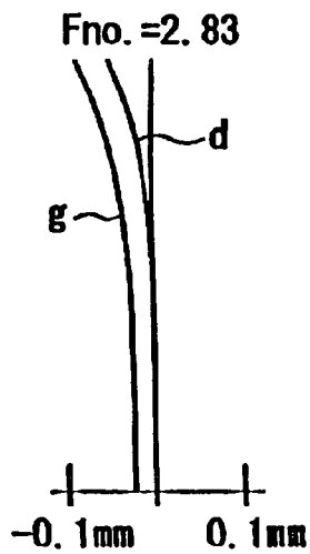
Spherical Aberration Fig. 10(A)
