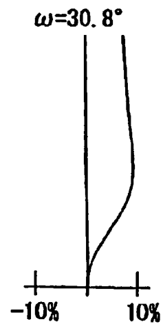
Distortion Fig. 7(C)
