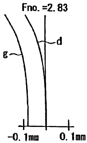
Spherical Aberration Fig. 7(A)
