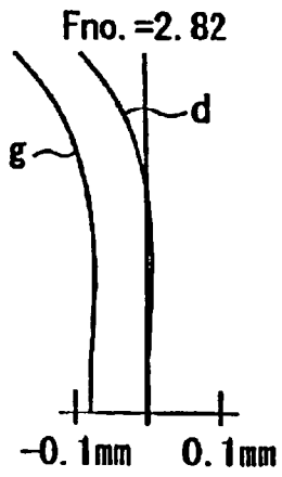
Spherical Aberration Fig. 6(A)
