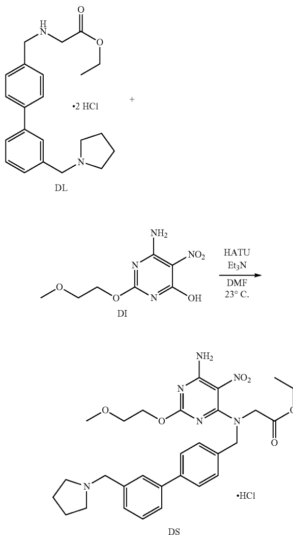
Scheme 86
