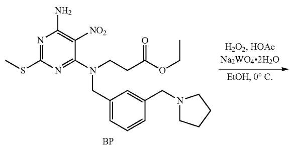
Scheme 36
