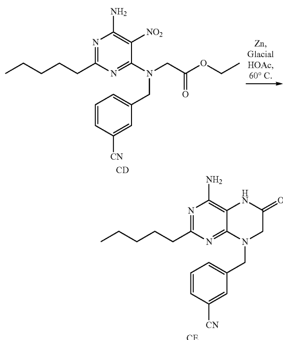
Scheme 52
