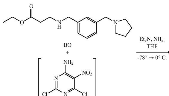
Scheme 40
