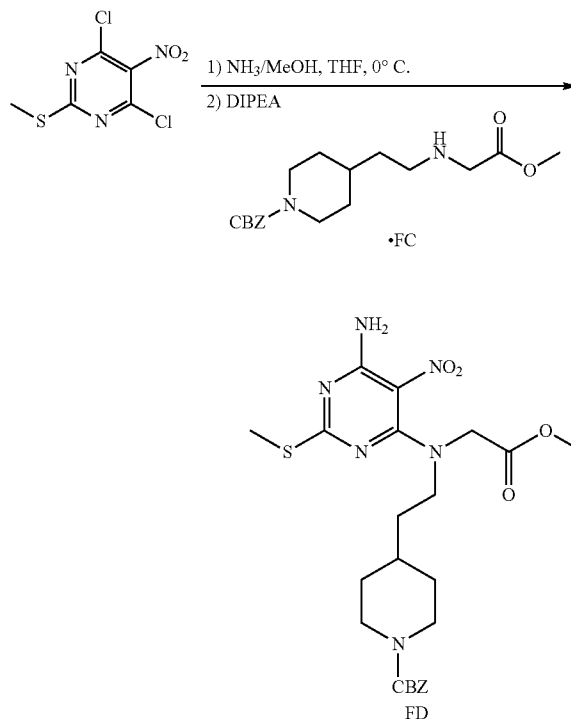
Scheme 92
