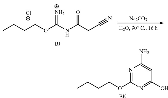
Scheme 29
