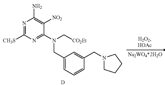
Scheme 32
