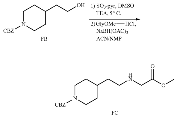
Scheme 91
