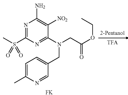
Scheme 100:
