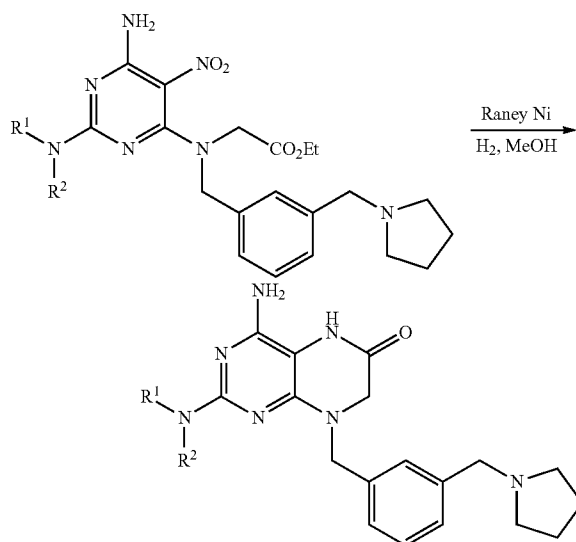
Scheme 17
