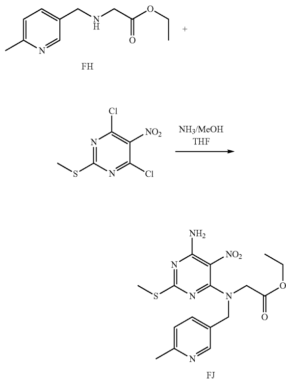
Scheme 98
