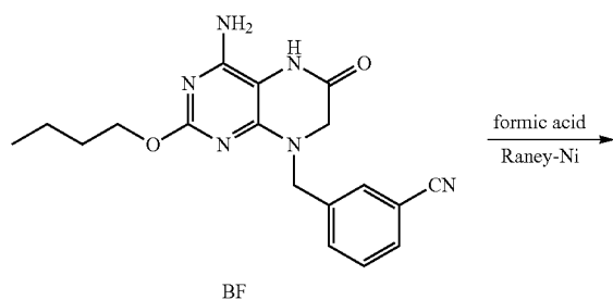
Scheme 24
