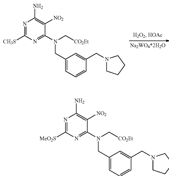
Scheme 11
