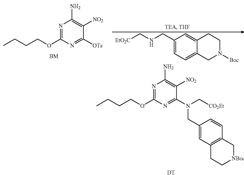
Scheme 89:
