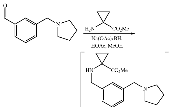
Scheme 12
