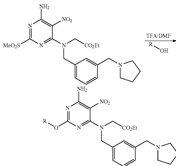
Scheme 14
