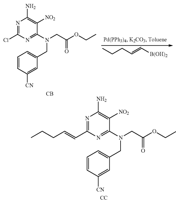
Scheme 50
