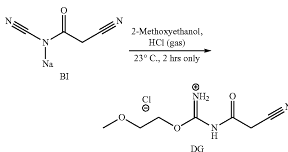
Scheme 74
