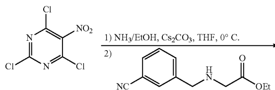
Scheme 49
