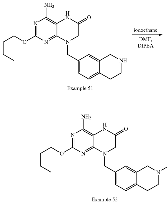
Scheme 48: Example 52
