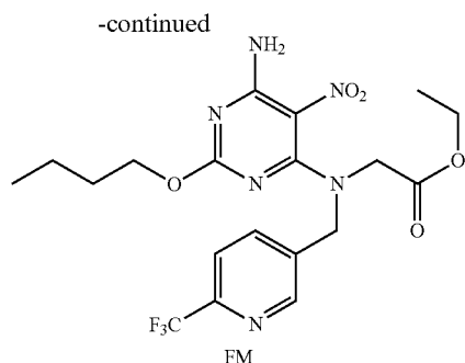
Scheme 105:
