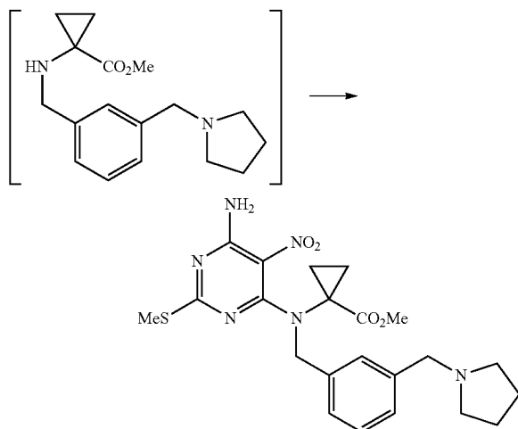
Scheme 19
