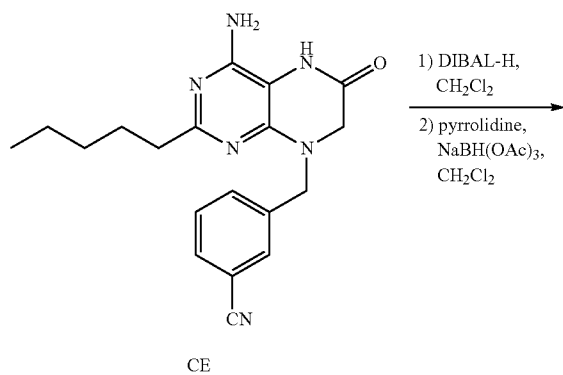
Scheme 53: Example 53
