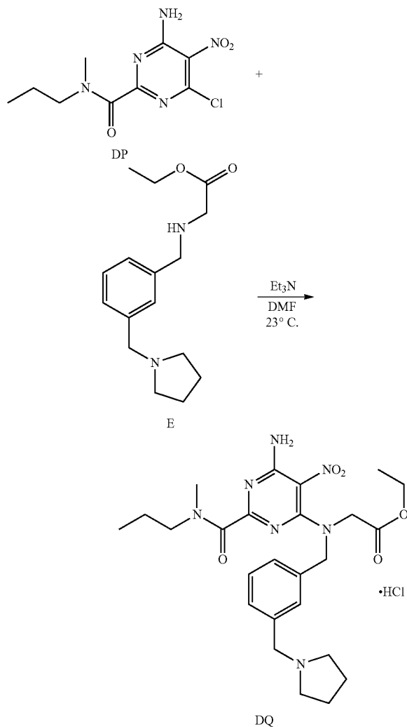
Scheme 83:
