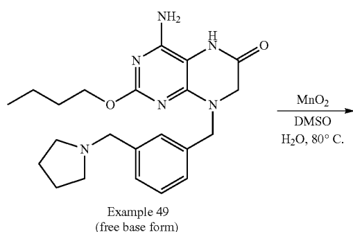
Scheme 87
