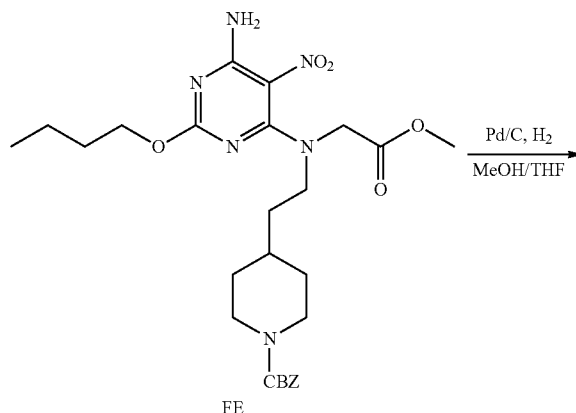
Scheme 94
