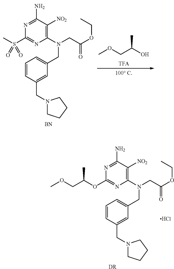
Scheme 85
