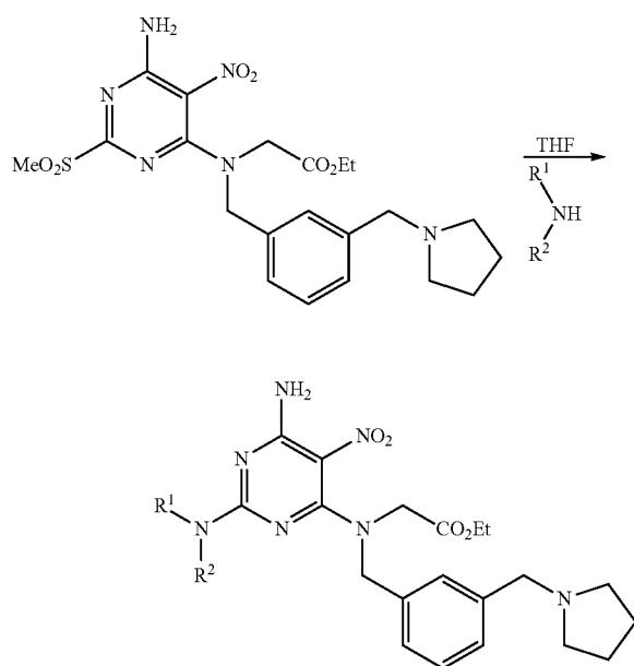
Scheme 16
