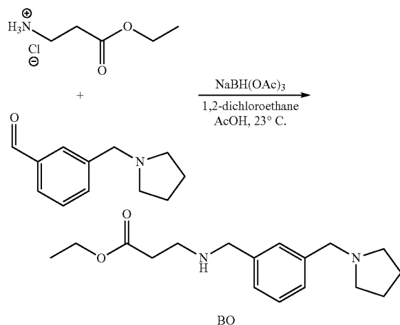
Scheme 33
