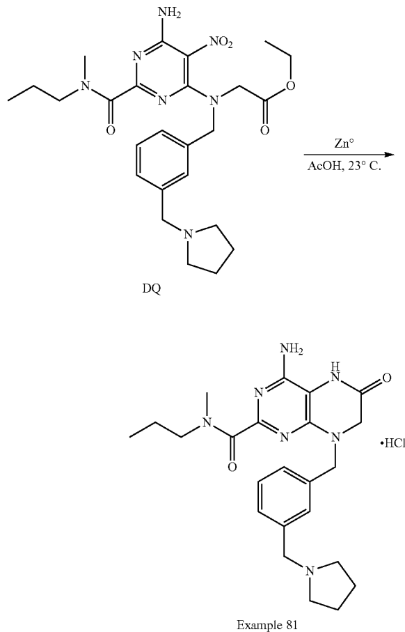
Scheme 84: Example 81
