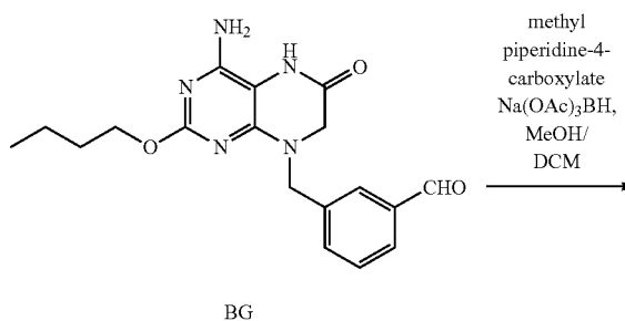
Scheme 54: Example 54
