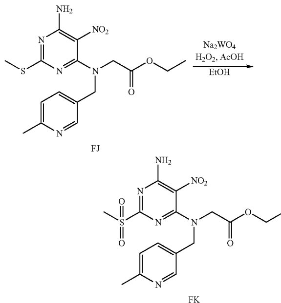
Scheme 99:
