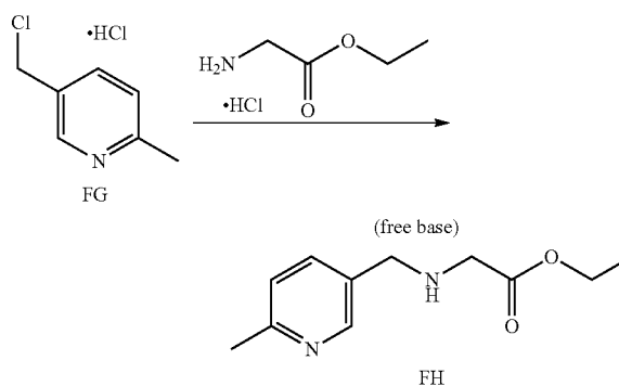
Scheme 97
