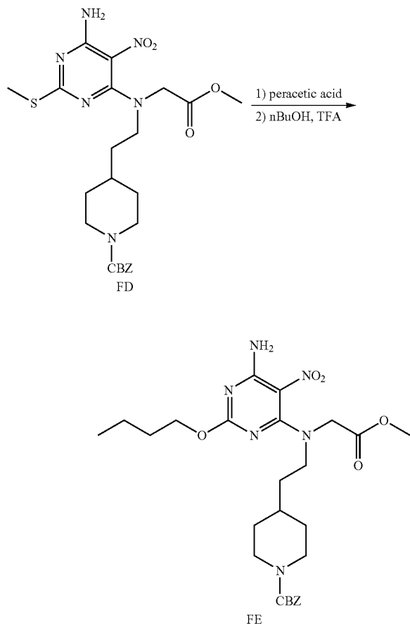
Scheme 93
