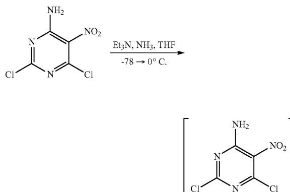
Scheme 39
