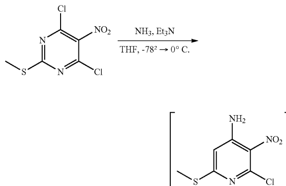
Scheme 34
