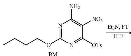
Scheme 104:
