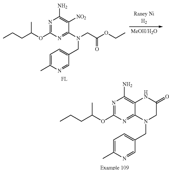
Scheme 101:
