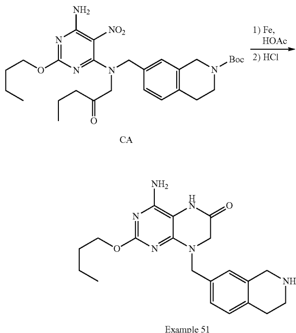
Scheme 47: Example 51
