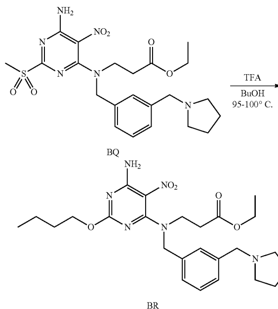
Scheme 37
