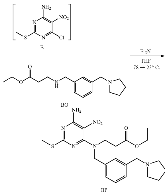
Scheme 35
