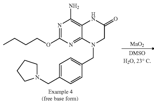
Scheme 88:
