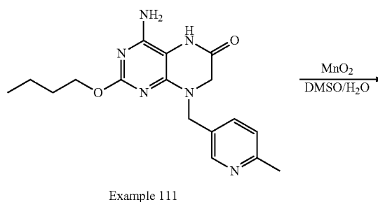
Scheme 111
